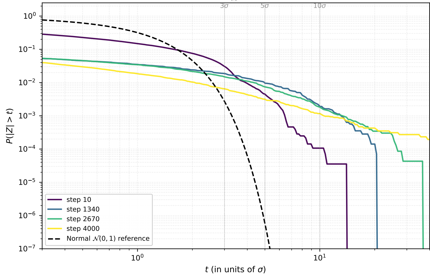
Token-level \delta = \log \pi_{\theta} - \log \pi_{\theta_{\text{old}}} has heavier tails than \mathcal{N}(0, 1)
