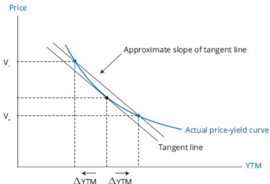
Figure 61.1: Approximate ModDur
