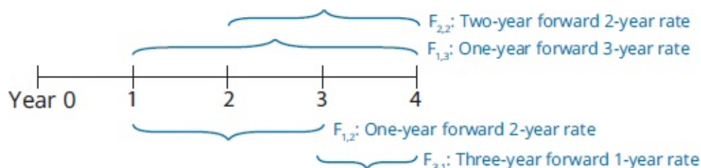
Figure 74.1: Forward Rates
