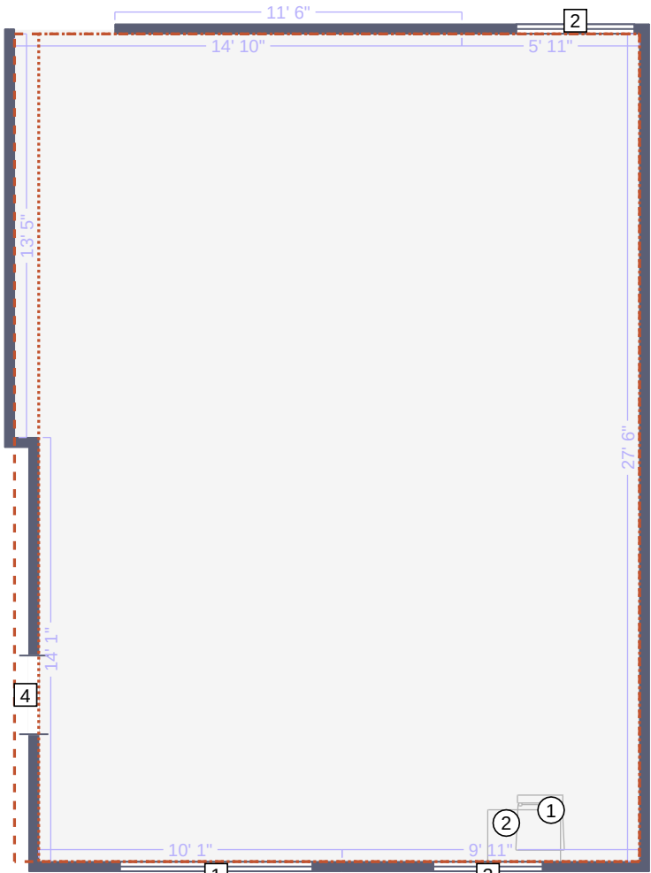
Other 1 Floor Plan
