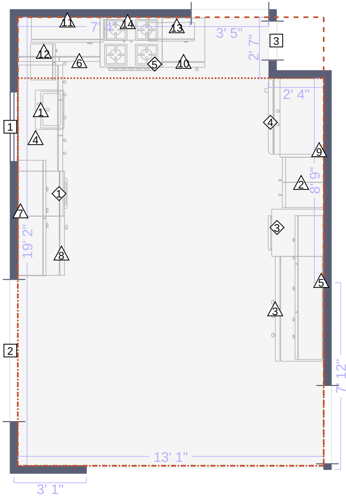
Kitchen Floor Plan
