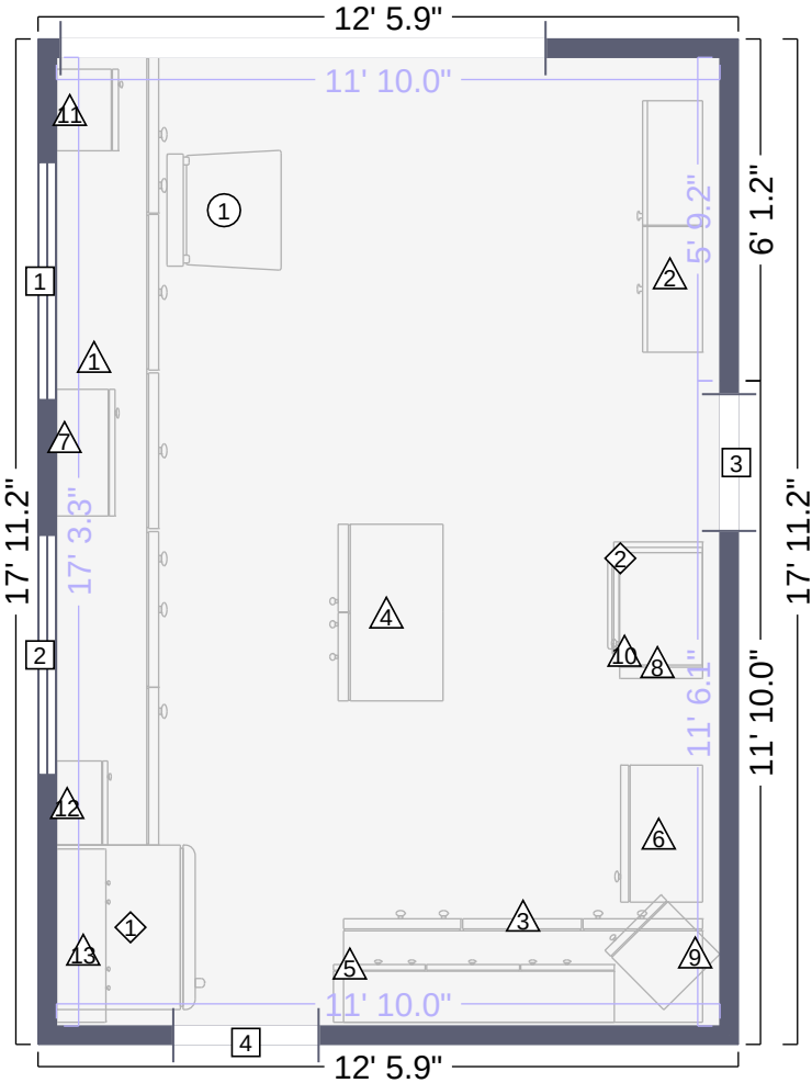
Kitchen Floor Plan
