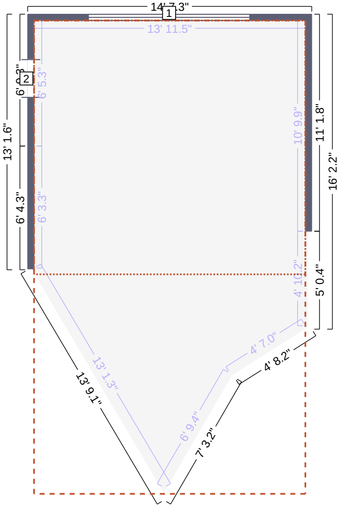
Other 3 Floor Plan
