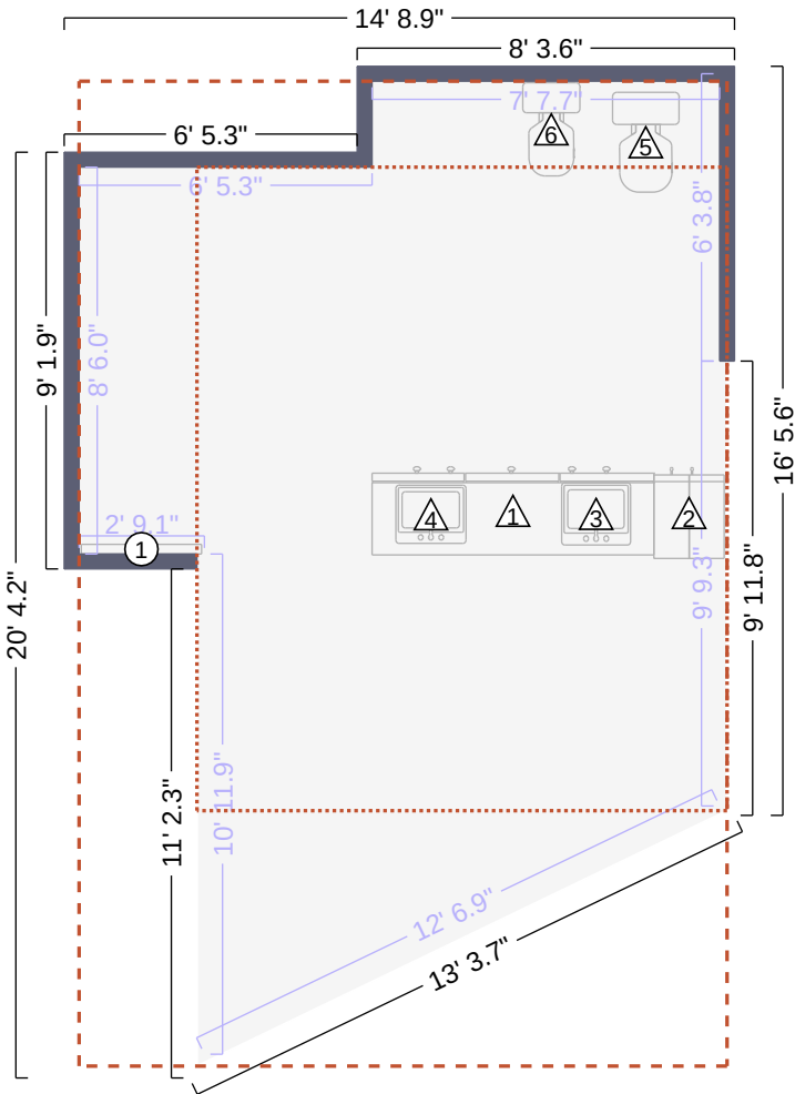
Bathroom 1 Floor Plan
