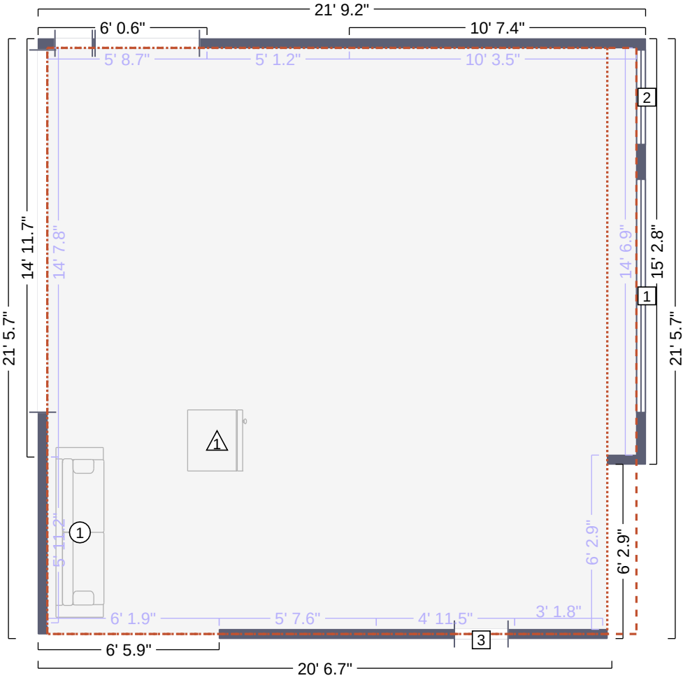
Other 1 Floor Plan
