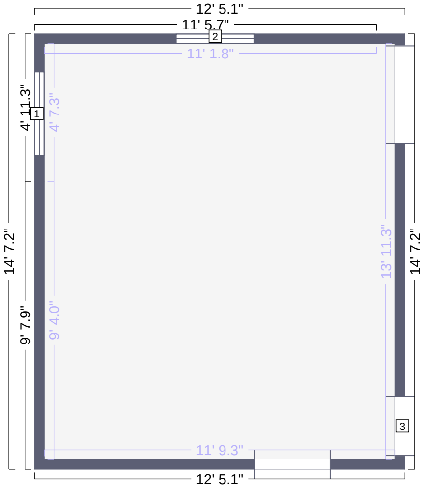
Other 3 Floor Plan
