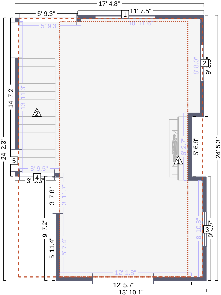
Living Room Floor Plan
