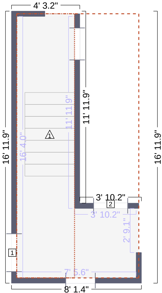
Other 4 Floor Plan
