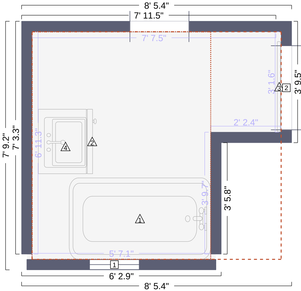
Bathroom 1 Floor Plan
