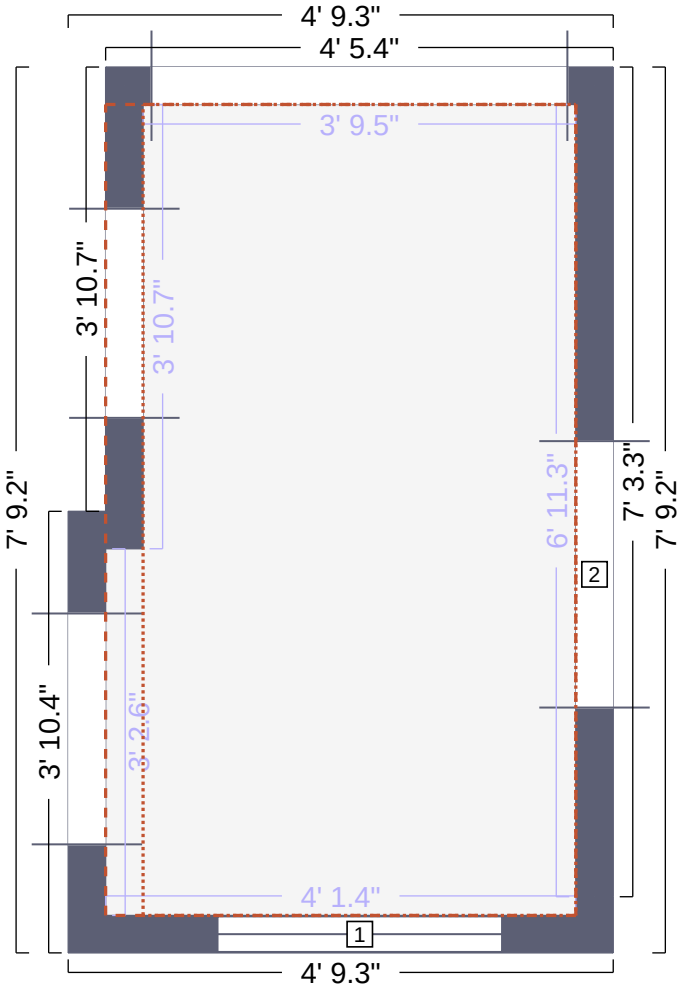
Other 5 Floor Plan
