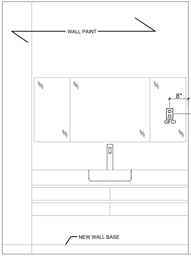
16 SECOND FLOOR GUEST TOILET SOUTH ELEVATION 1/2" = 1'
