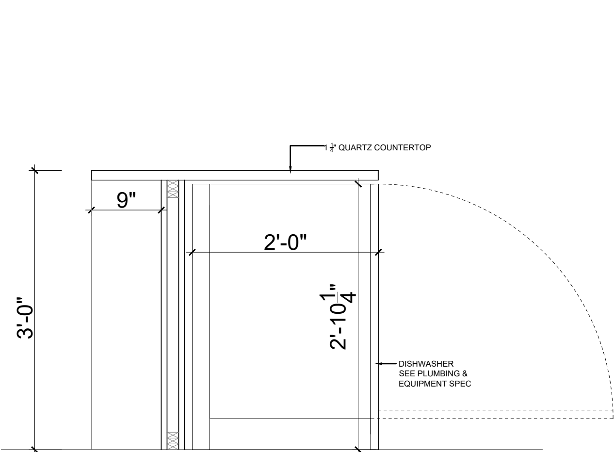
04 MILLWORK SECTION DETAIL 4 - DISHWASHER
