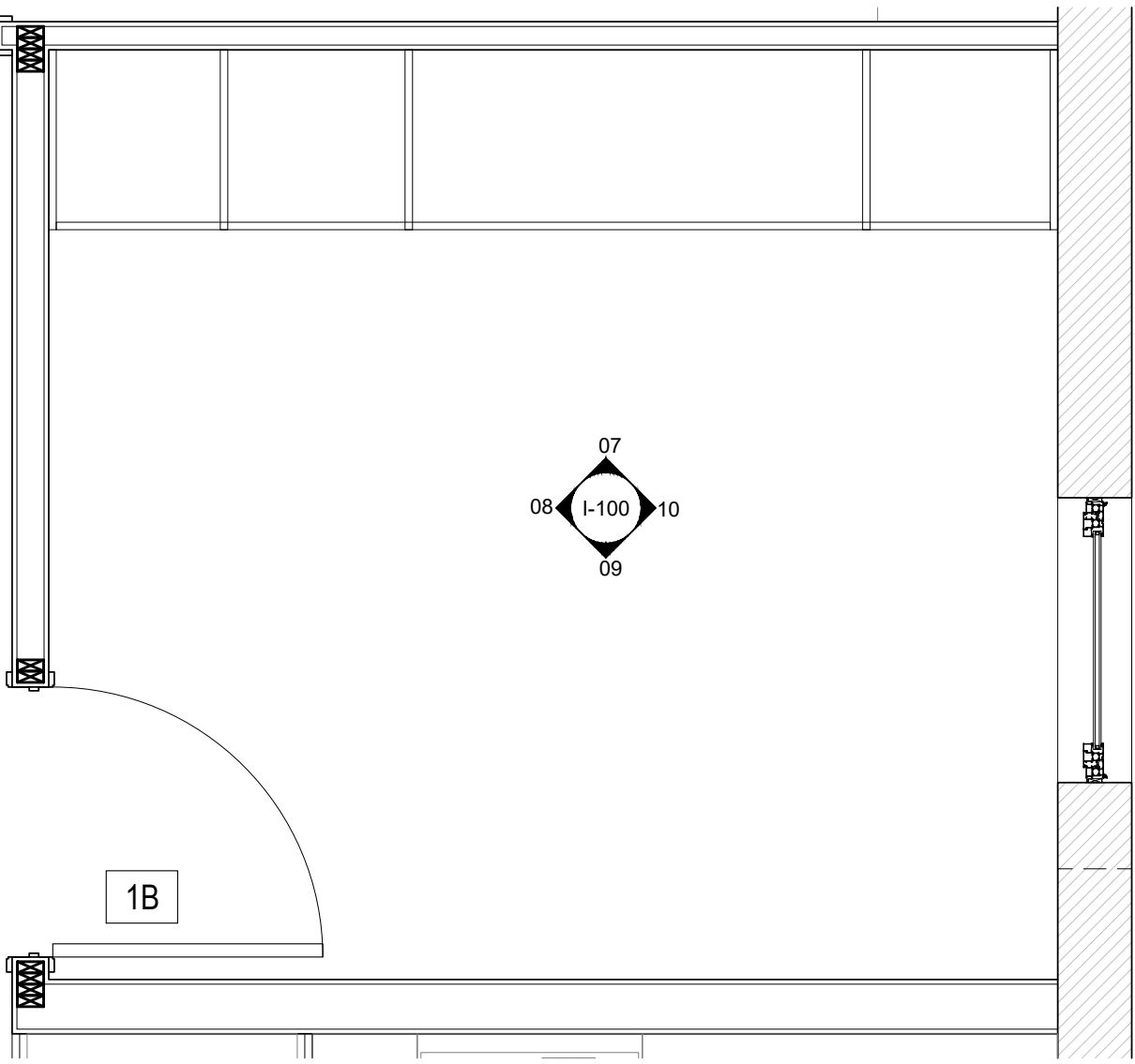
06 FIRST FLOOR GUEST BEDROOM ENLARGED PLAN 1/2" = 1'
