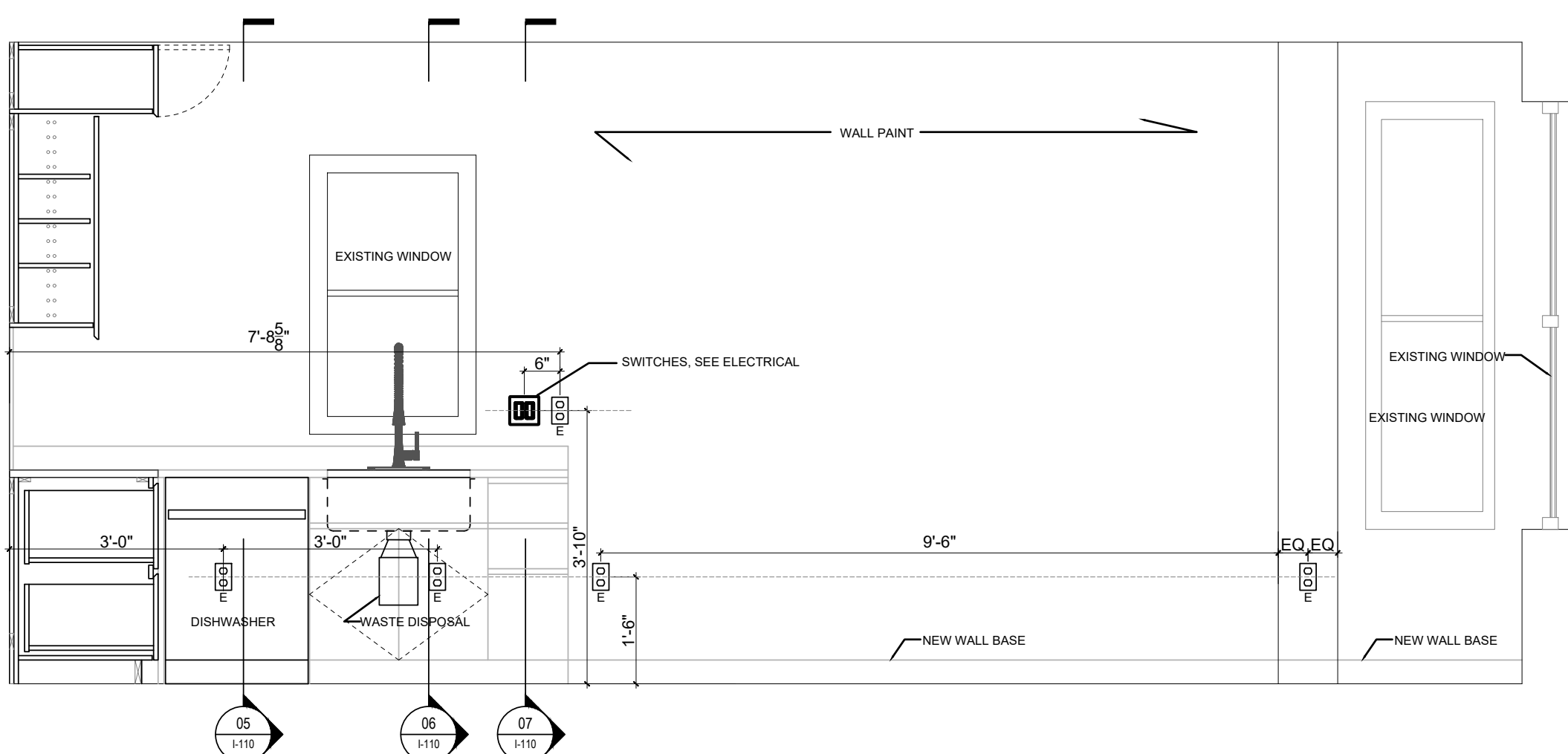
04 FIRST FLOOR LIVING ROOM & KITCHEN WEST ELEVATION 1/12" = 1'
