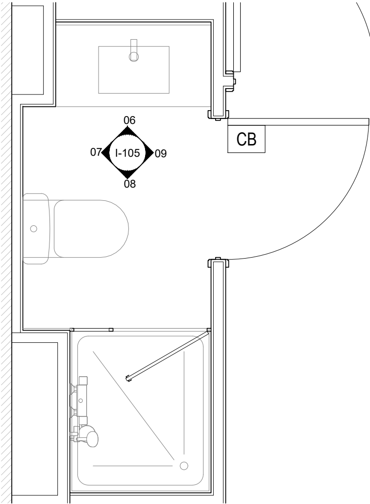
05 CELLAR TOILET ENLARGED PLAN 1/2" = 1'
