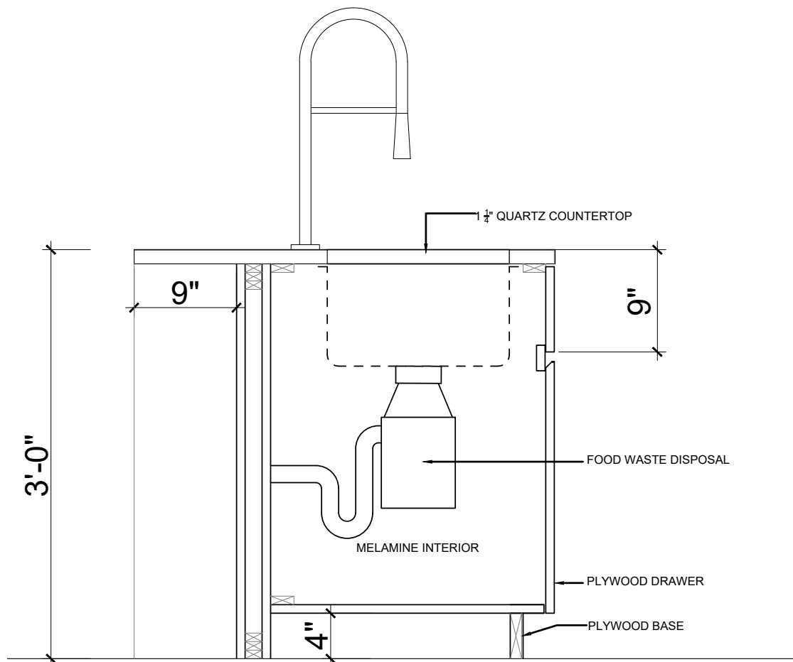
05 MILLWORK SECTION DETAIL 5 - SINK
