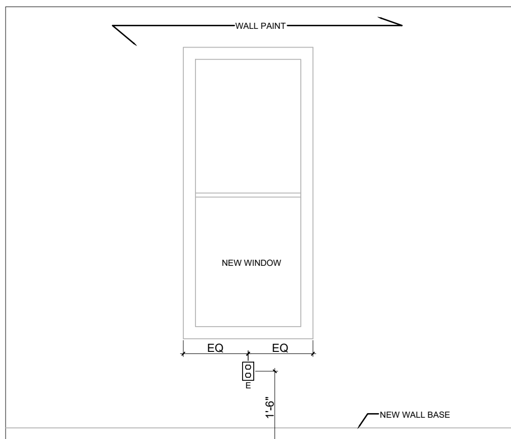
02 SECOND FLOOR GUEST BEDROOM SOUTH ELEVATION 1/2" = 1'
