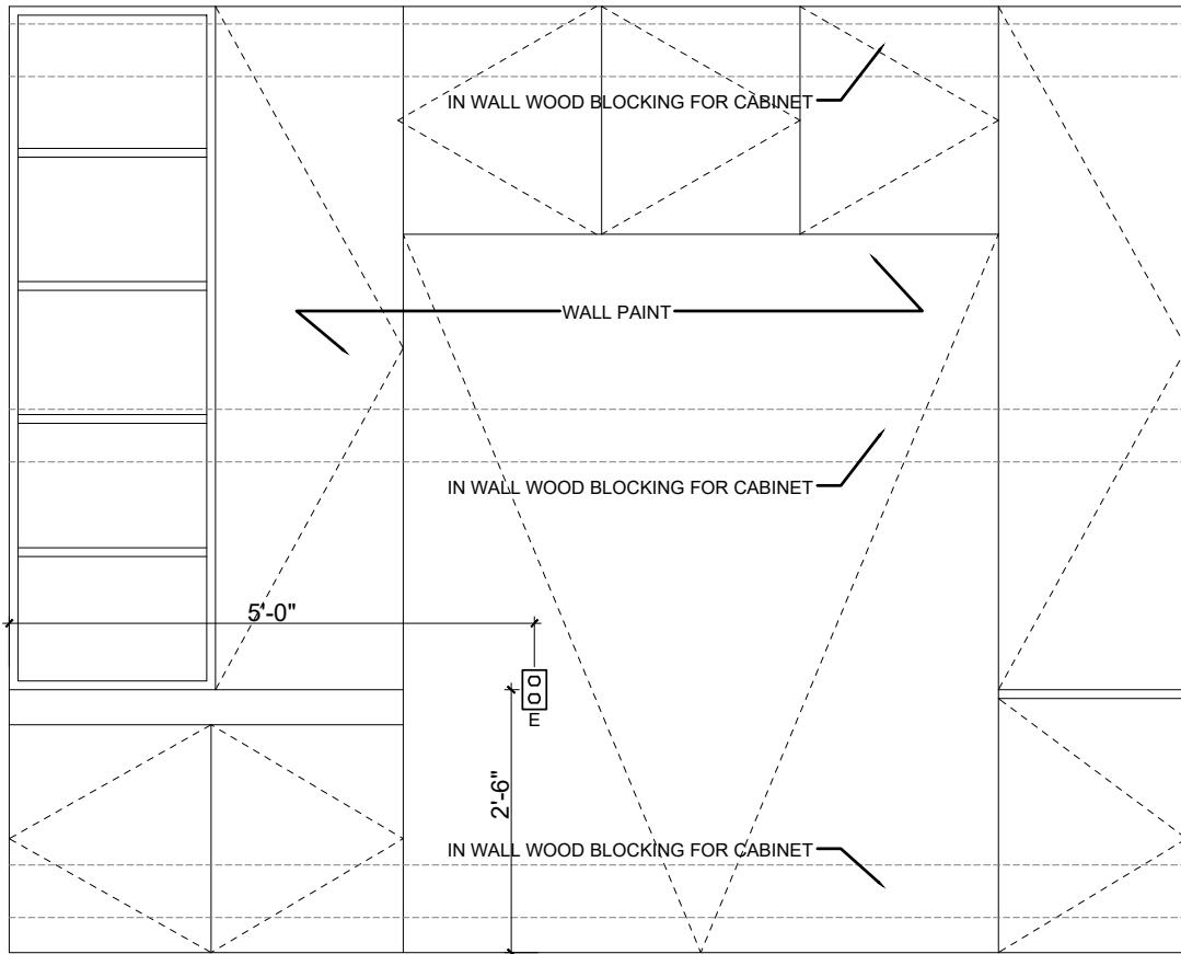
07 FIRST FLOOR GUEST BEDROOM SOUTH ELEVATION 1/2" = 1'
