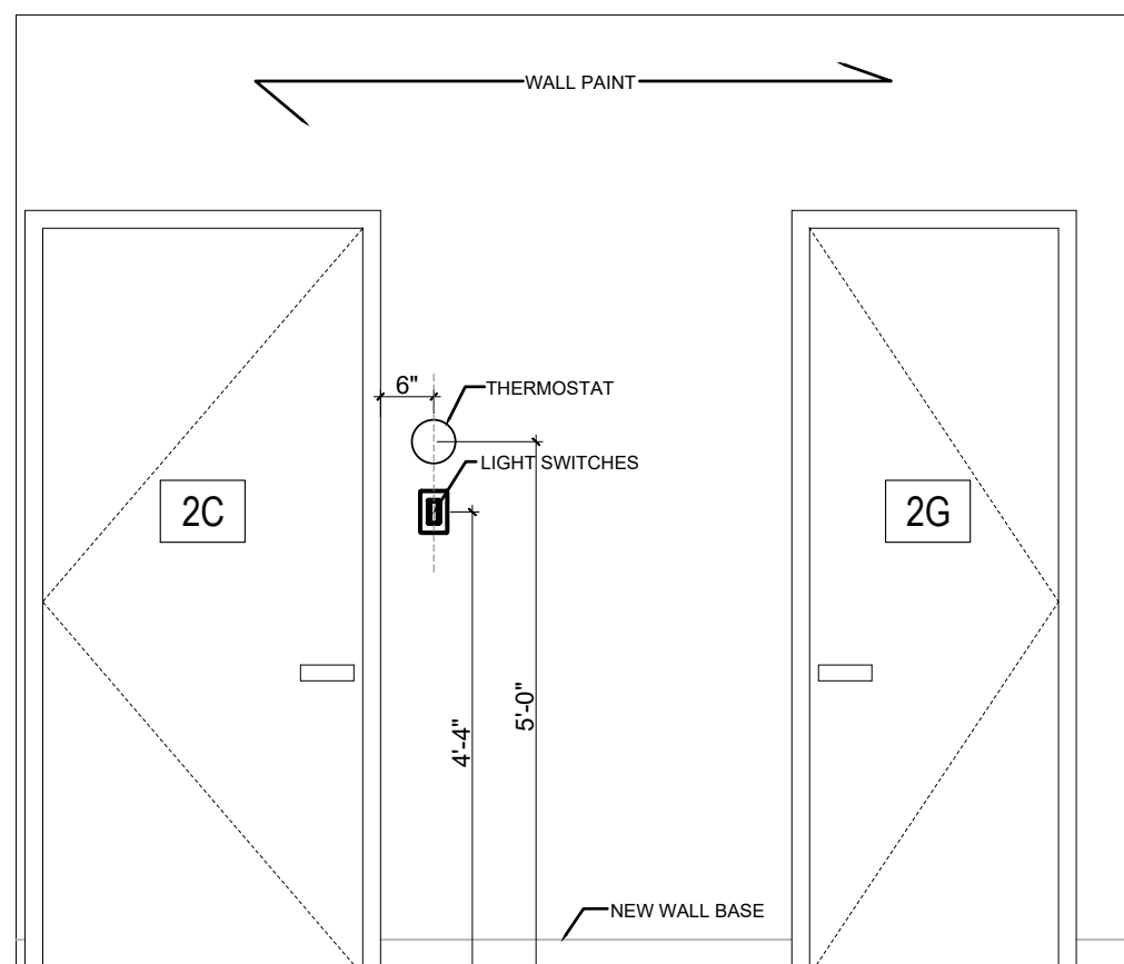
04 SECOND FLOOR GUEST BEDROOM NORTH ELEVATION 1/2" = 1'
