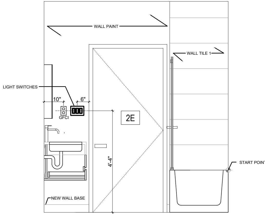
19 SECOND FLOOR GUEST TOILET WEST ELEVATION 1/2" = 1'
