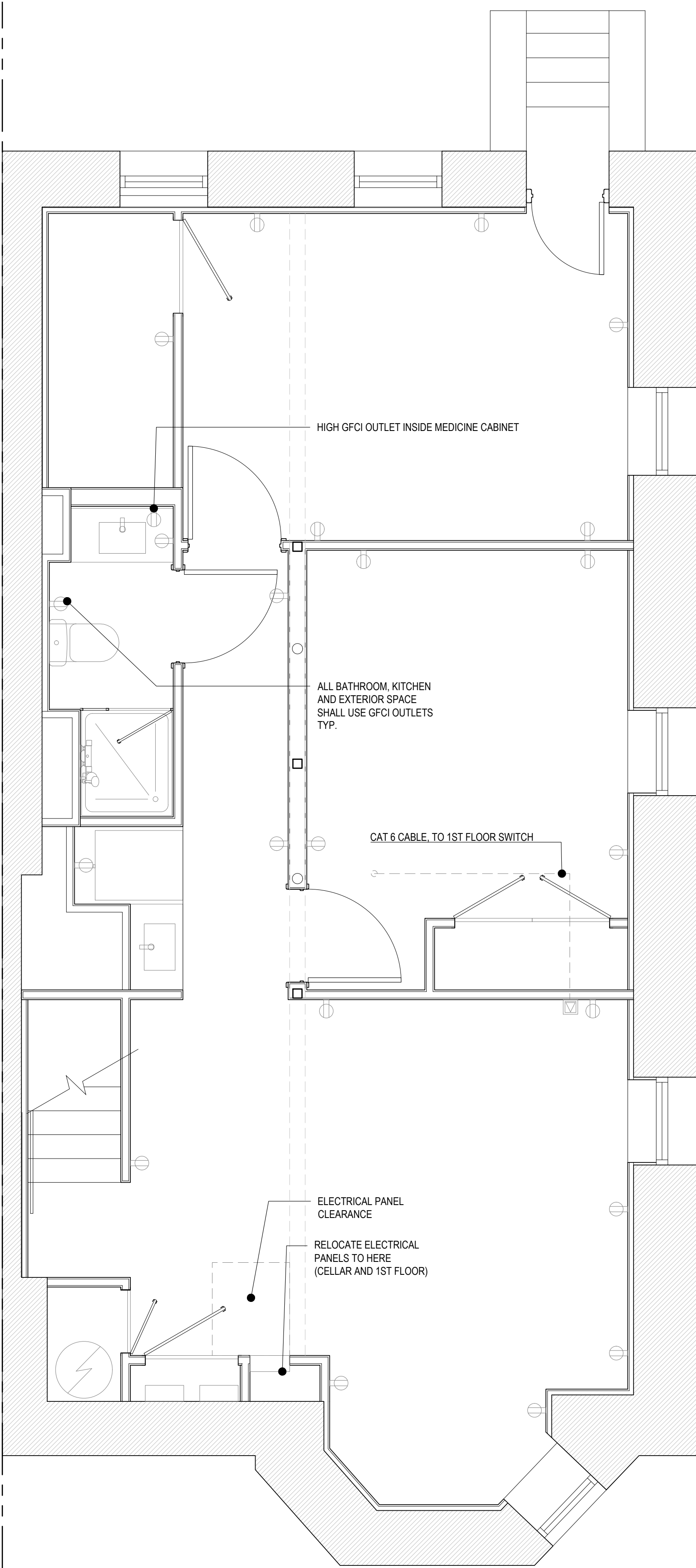
01 BASEMENT FLOOR - POWER PLAN 3/16" = 1'
