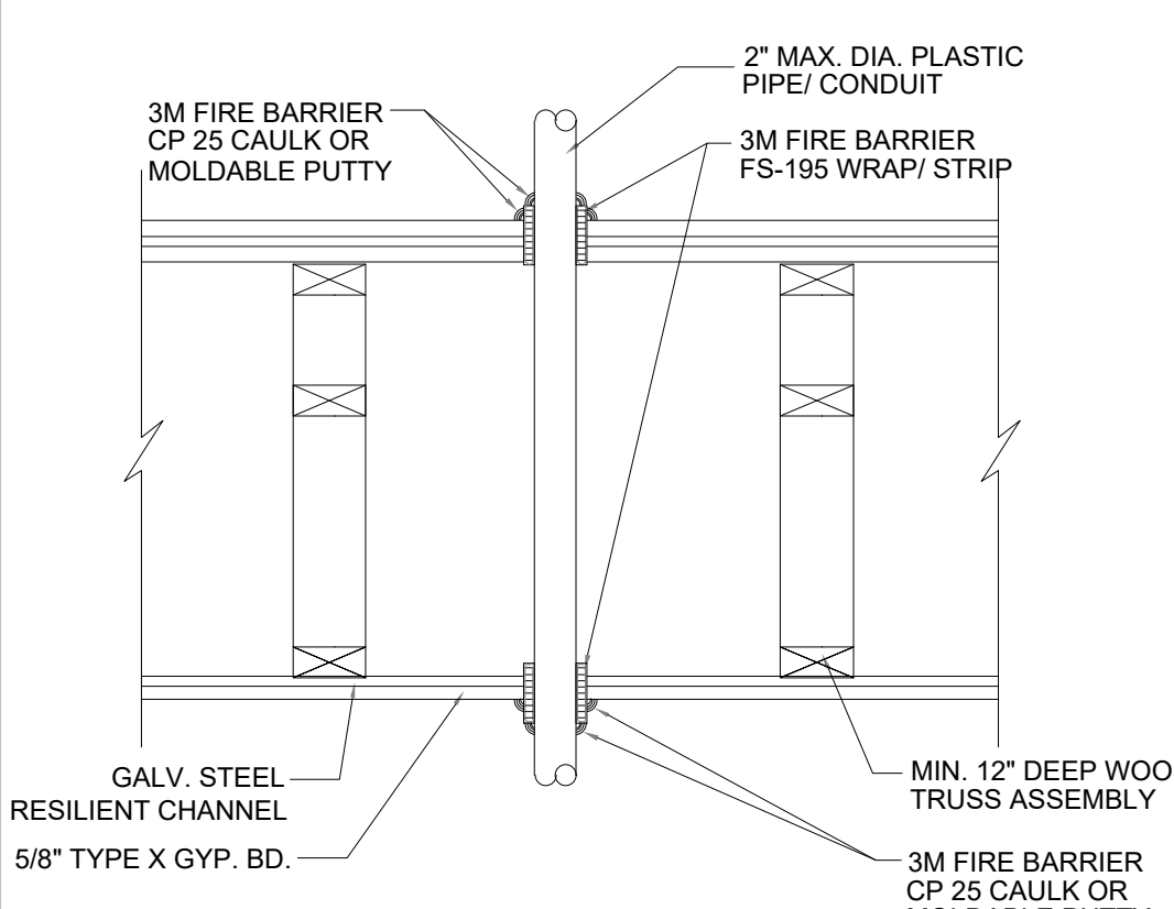
PENETRATION FIRESTOP FOR 2" MAX. DIA. PLASTIC PIPE/ CONDUIT THROUGH A WOOD & METAL PIPE TRUSS FLOOR/ CEILING ASSEMBLY- 1 HR. RATED U.L. LISTING - F-C-2008
