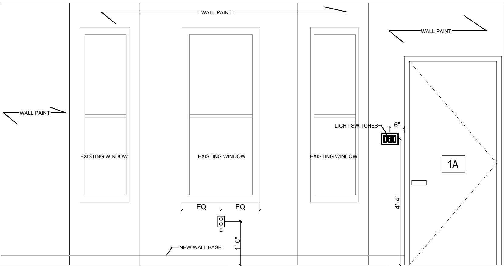
03 FIRST FLOOR LIVING ROOM & KITCHEN NORTH ELEVATION 1/12" = 1'
