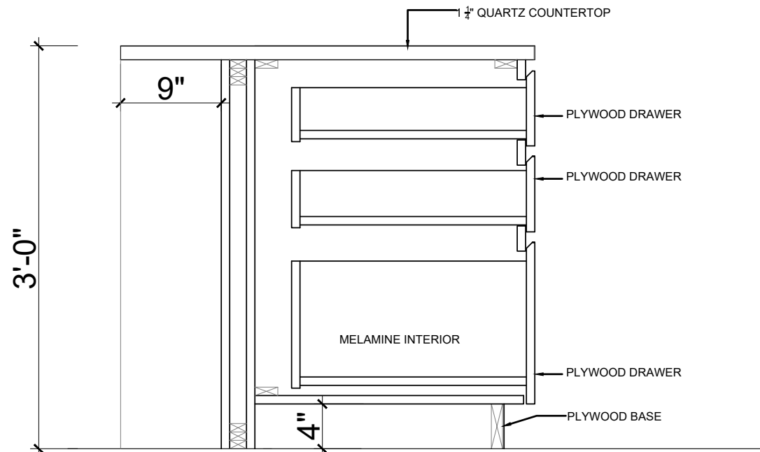
07 MILLWORK SECTION DETAIL 7 - DRAWER
