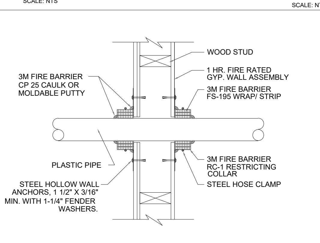
PENETRATION FIRESTOP FOR 4" MAX. DIA. ABS & PVC PLASTIC PIPE THROUGH A GYPSUM WALLBOARD ASSEMBLY- 1 HR. RATED U.L. LISTING - W-L-2059
