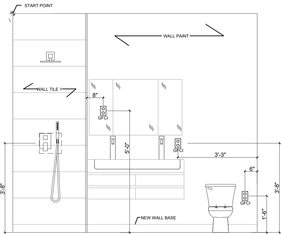
10 SECOND FLOOR MASTER TOILET NORTH ELEVATION 1/2" = 1'
