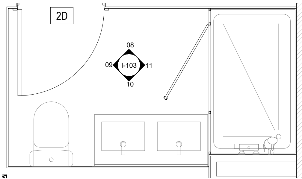
07 SECOND FLOOR MASTER TOILET ENLARGED PLAN 1/2" = 1'
