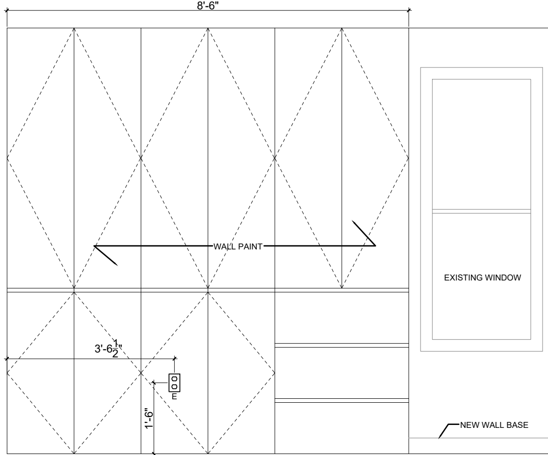
05 FIRST FLOOR MASTER BEDROOM WEST ELEVATION 1/2" = 1'
