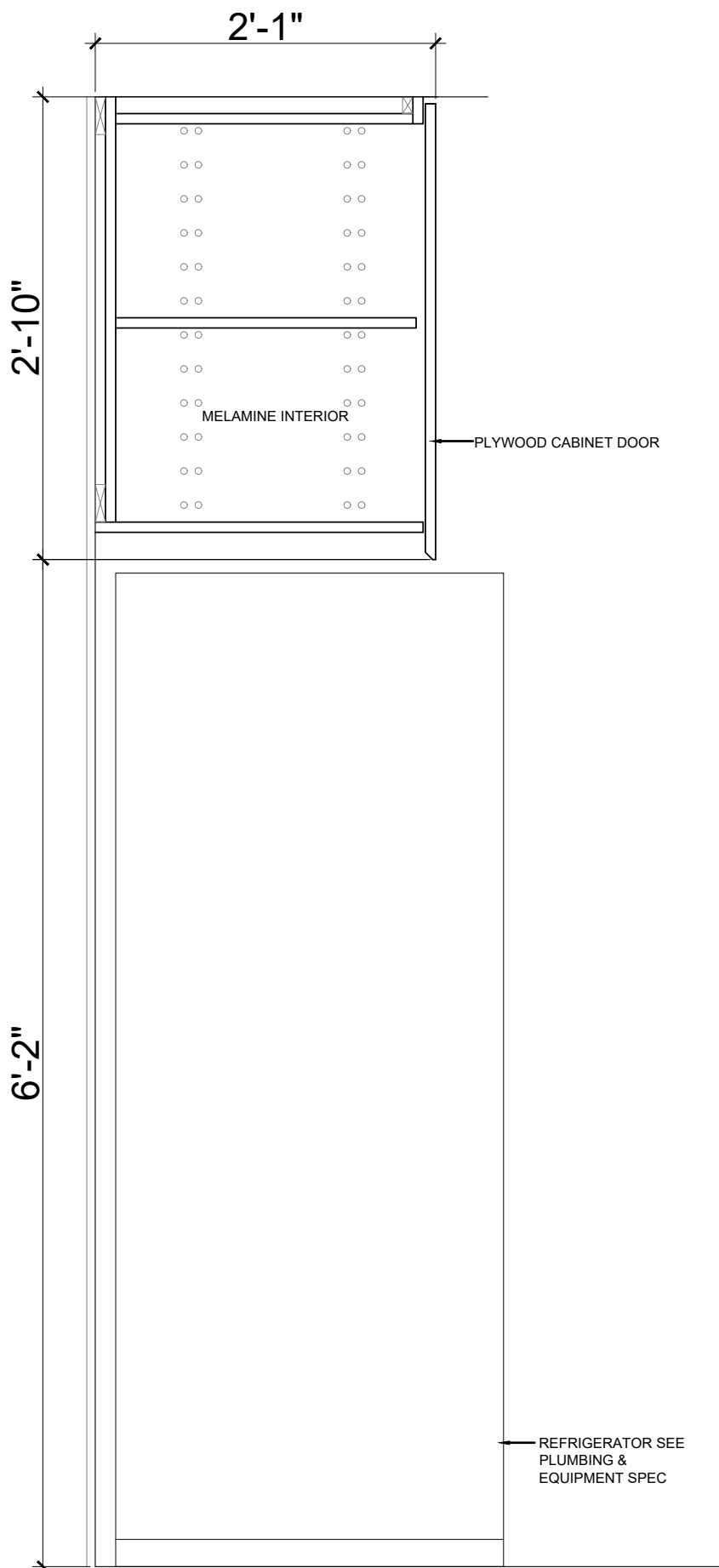
01 MILLWORK SECTION DETAIL 1 - REFRIGERATOR
