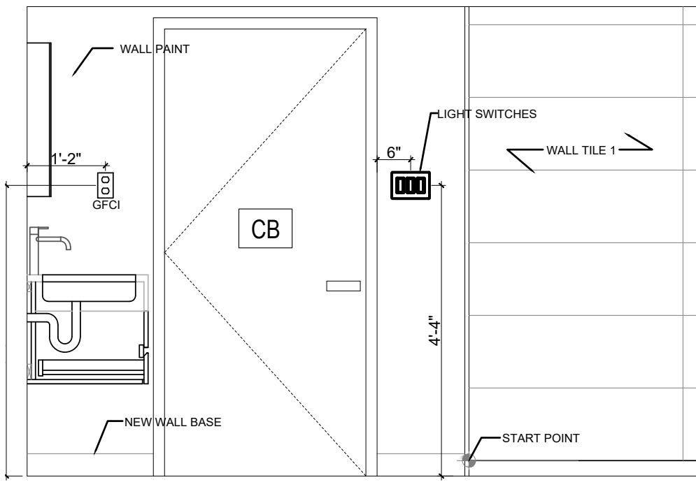
09 CELLAR TOILET WEST ELEVATION 1/2" = 1'
