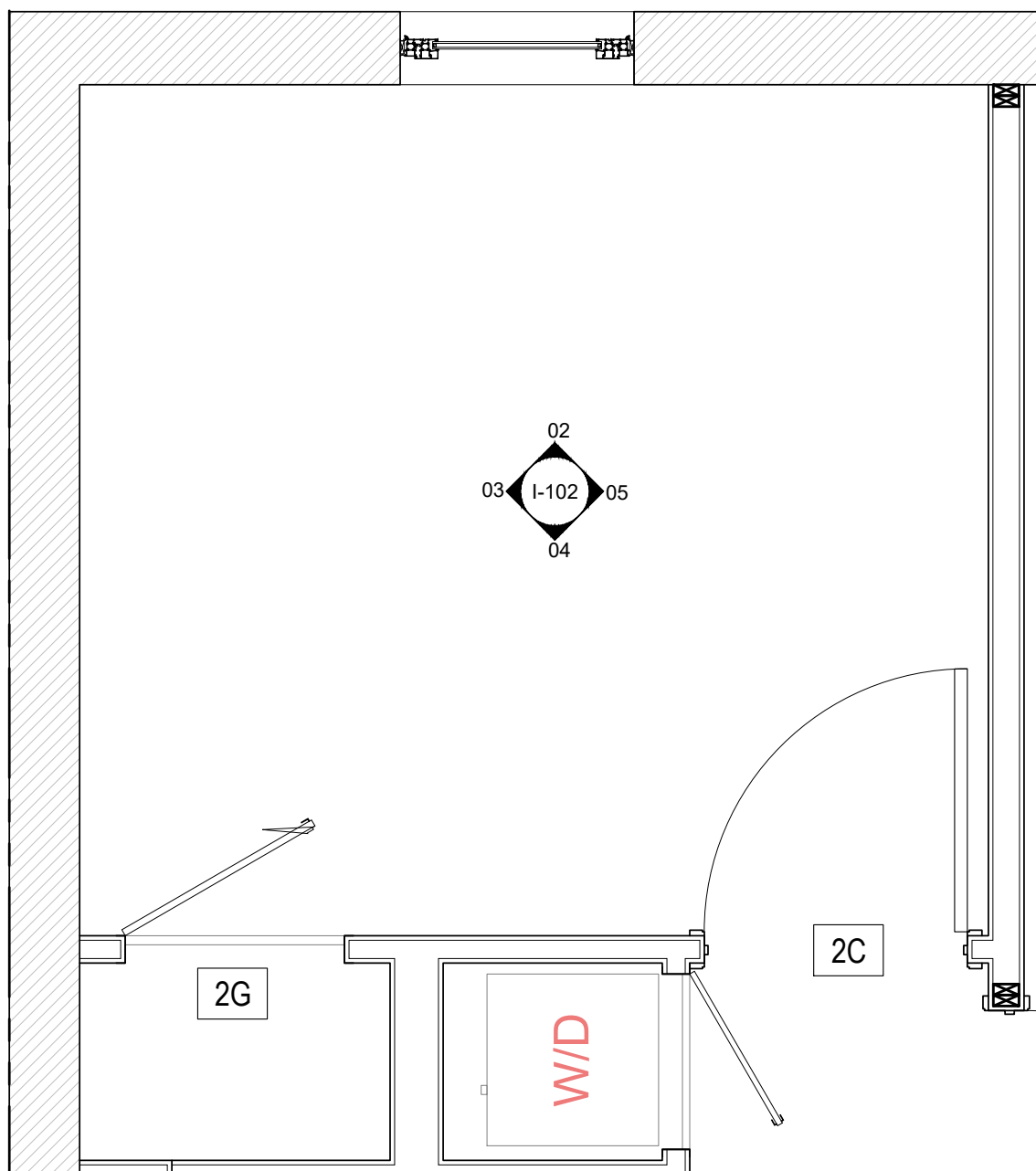
01 SECOND FLOOR GUEST BEDROOM ENLARGED PLAN 1/2" = 1'
