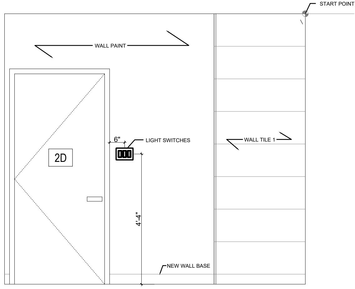
08 SECOND FLOOR MASTER TOILET SOUTH ELEVATION 1/2" = 1'
