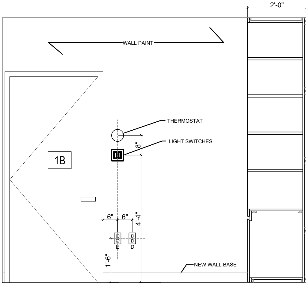
08 FIRST FLOOR GUEST BEDROOM EAST ELEVATION 1/2" = 1'
