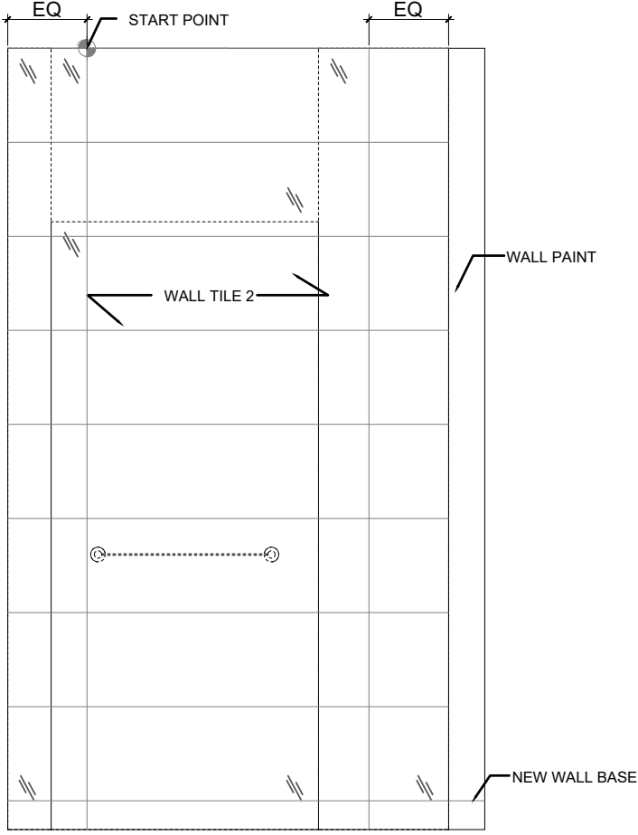
11 SECOND FLOOR MASTER TOILET WEST ELEVATION 1/2" = 1'
