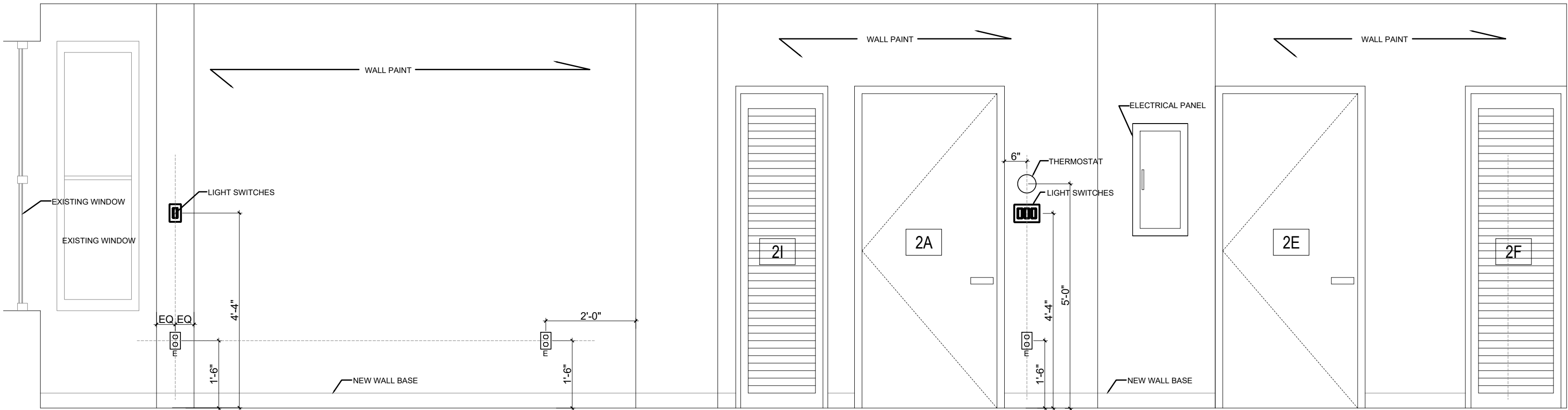
02 SECOND FLOOR LIVING ROOM & CORRIDOR EAST ELEVATION 1/2" = 1'
