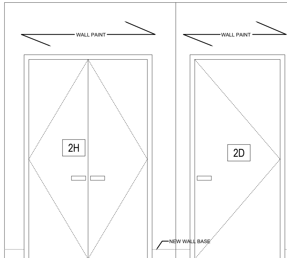
09 SECOND FLOOR MASTER BEDROOM NORTH ELEVATION 1/2" = 1'
