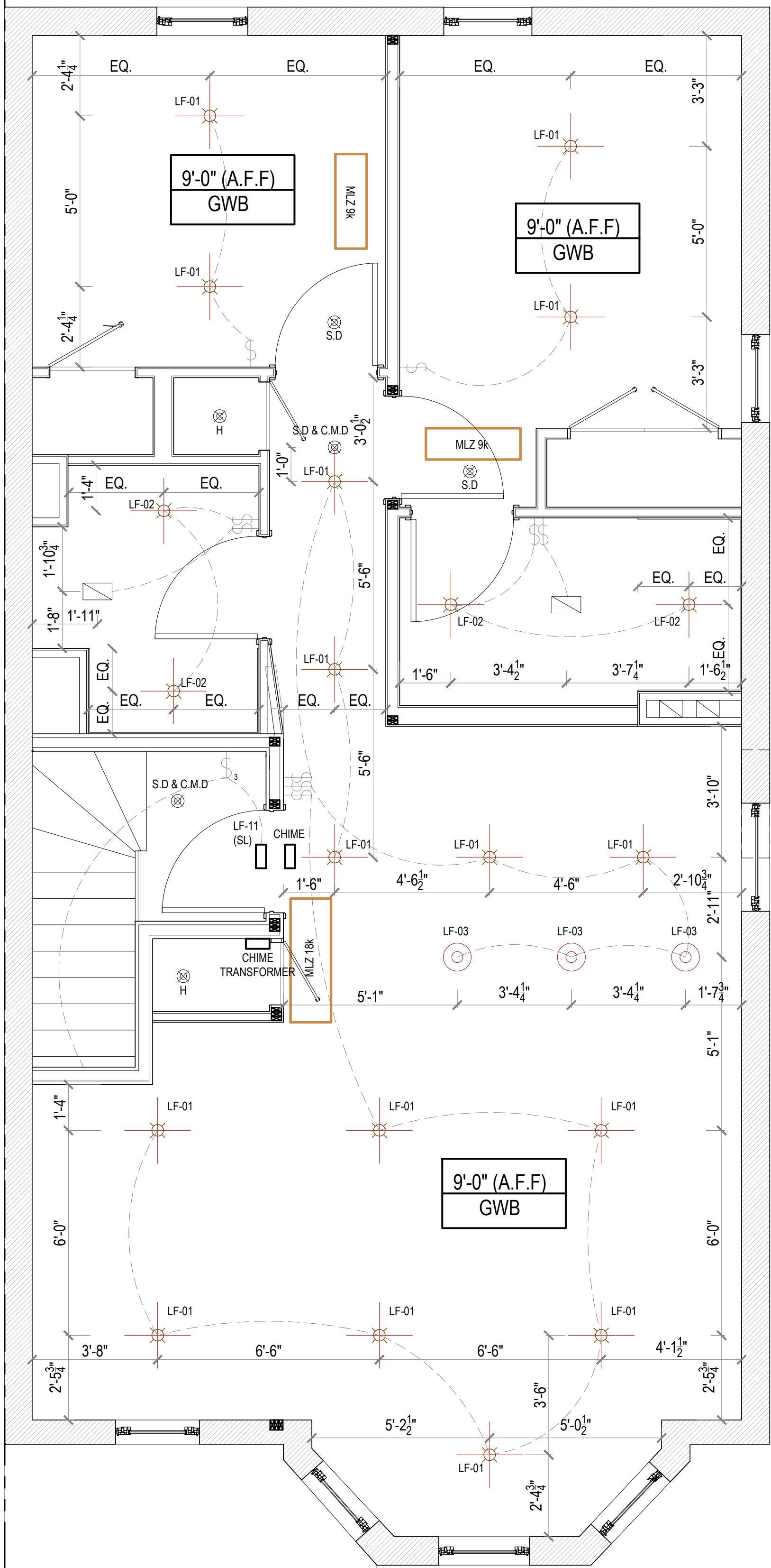
03 2ND FLOOR - RCP
