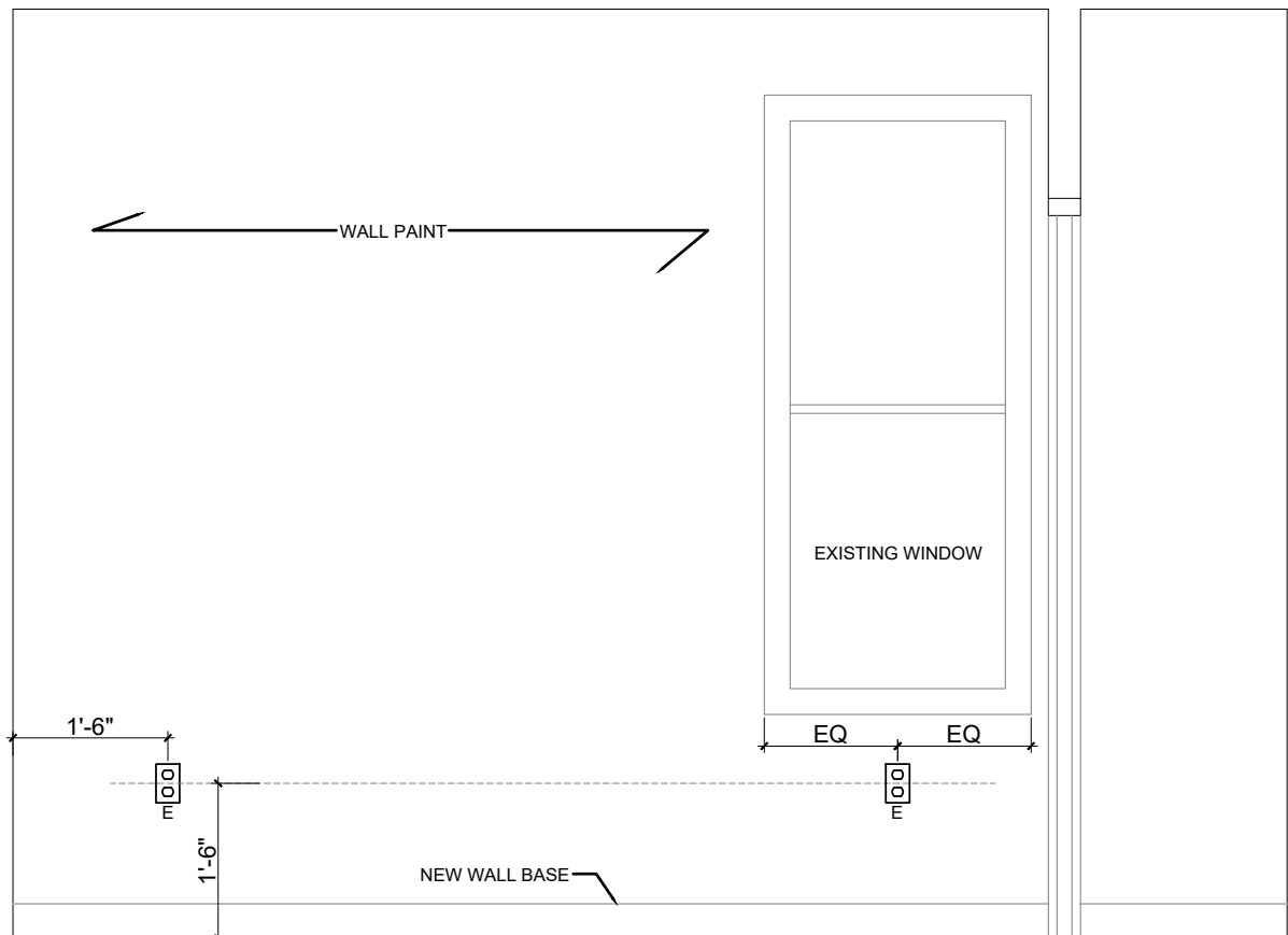
10 SECOND FLOOR MASTER BEDROOM WEST ELEVATION 1/2" = 1'
