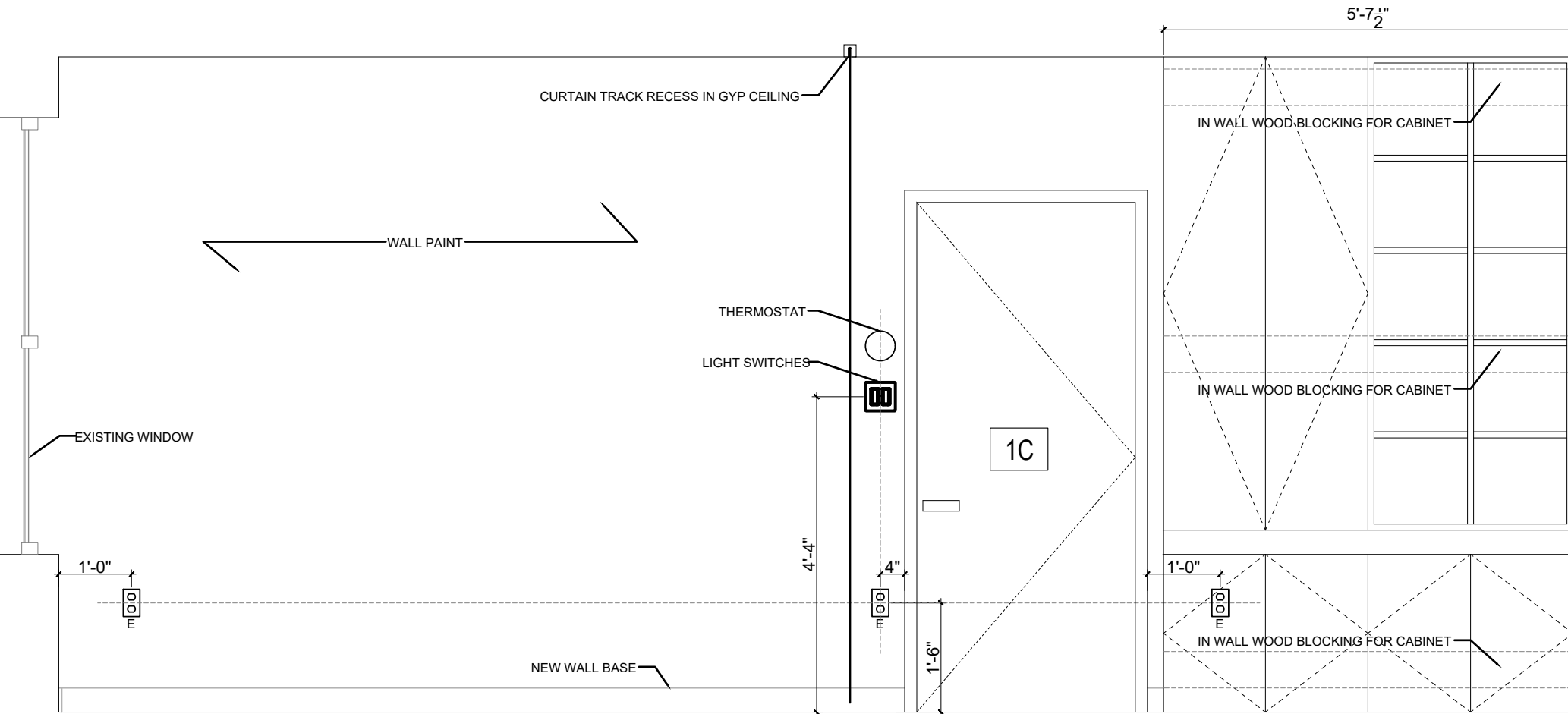
04 FIRST FLOOR MASTER BEDROOM NORTH ELEVATION 1/2" = 1'
