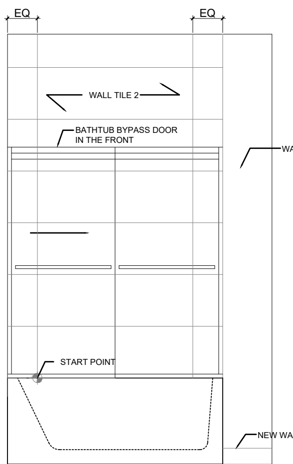
08 FIRST FLOOR TOILET NORTH ELEVATION 1/12" = 1'
