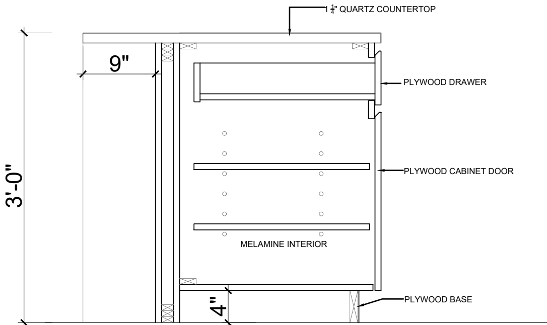
06 MILLWORK SECTION DETAIL 6 - DRAWER AND CABINET
