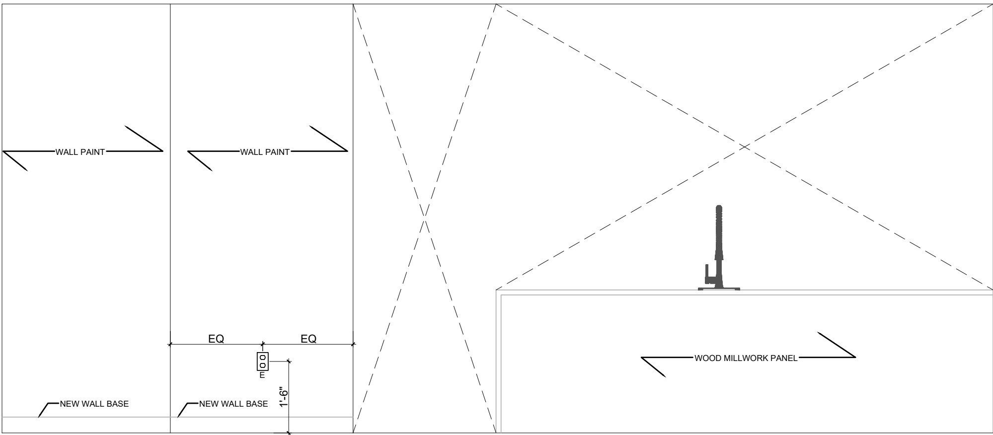
01 SECOND FLOOR LIVING ROOM SOUTH ELEVATION 1/2" = 1'
