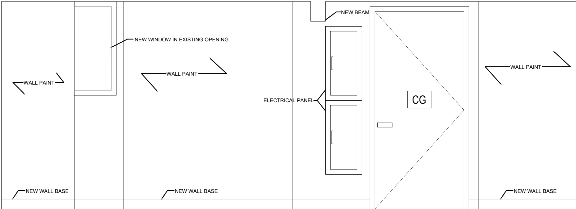
03 SECOND FLOOR LIVING ROOM NORTH ELEVATION 1/2" = 1'
