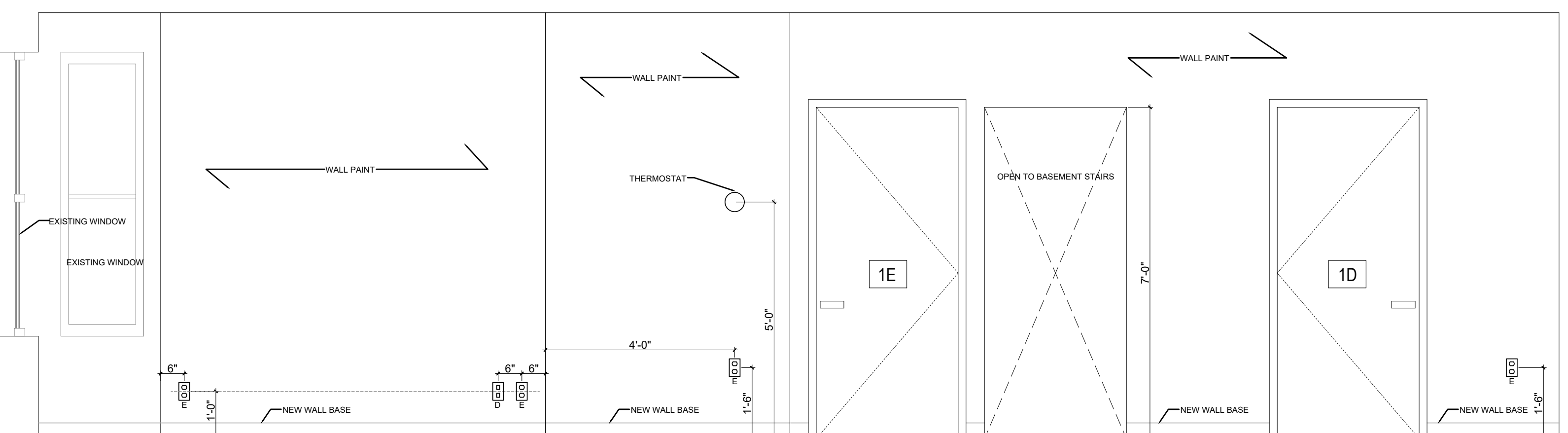
04 FIRST FLOOR LIVING ROOM & KITCHEN WEST ELEVATION 1/12" = 1'
