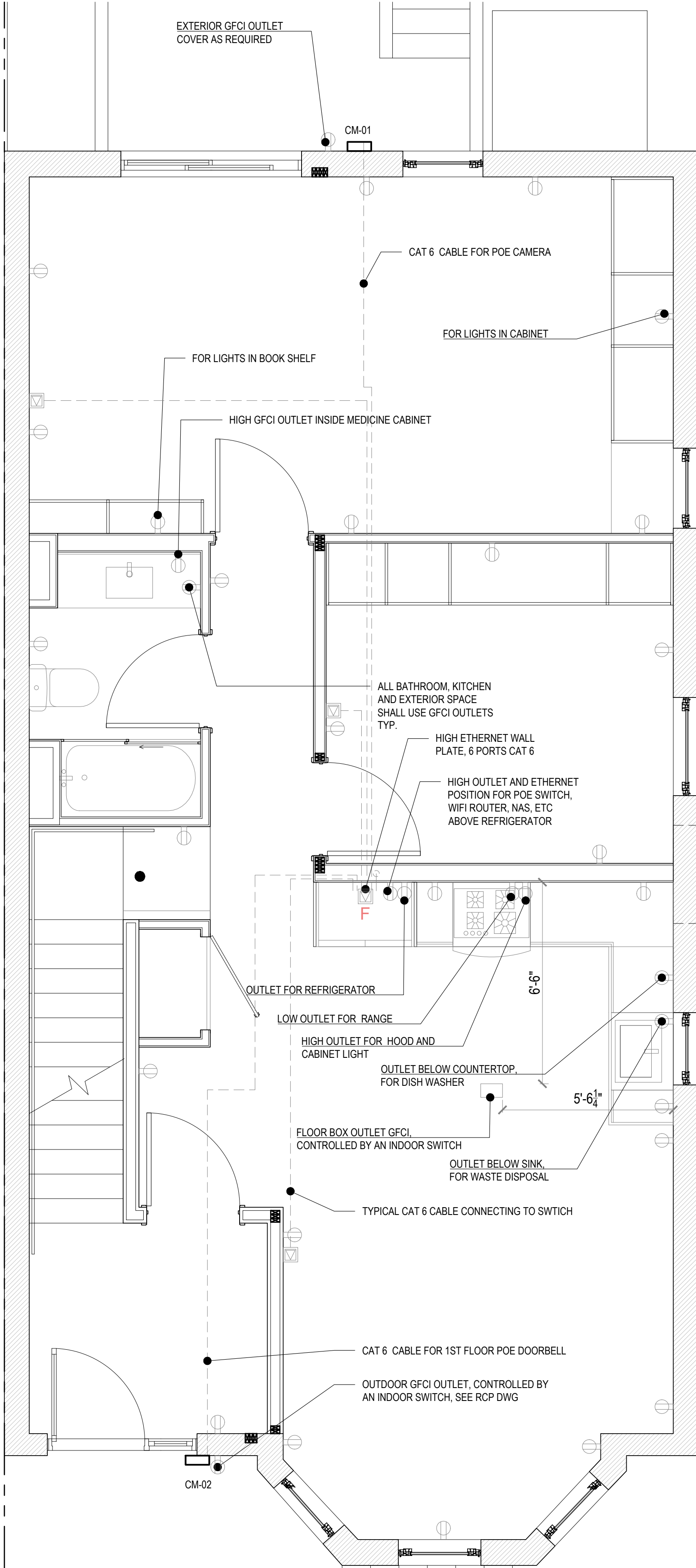
02 1ST FLOOR - POWER PLAN 3/16" = 1'
