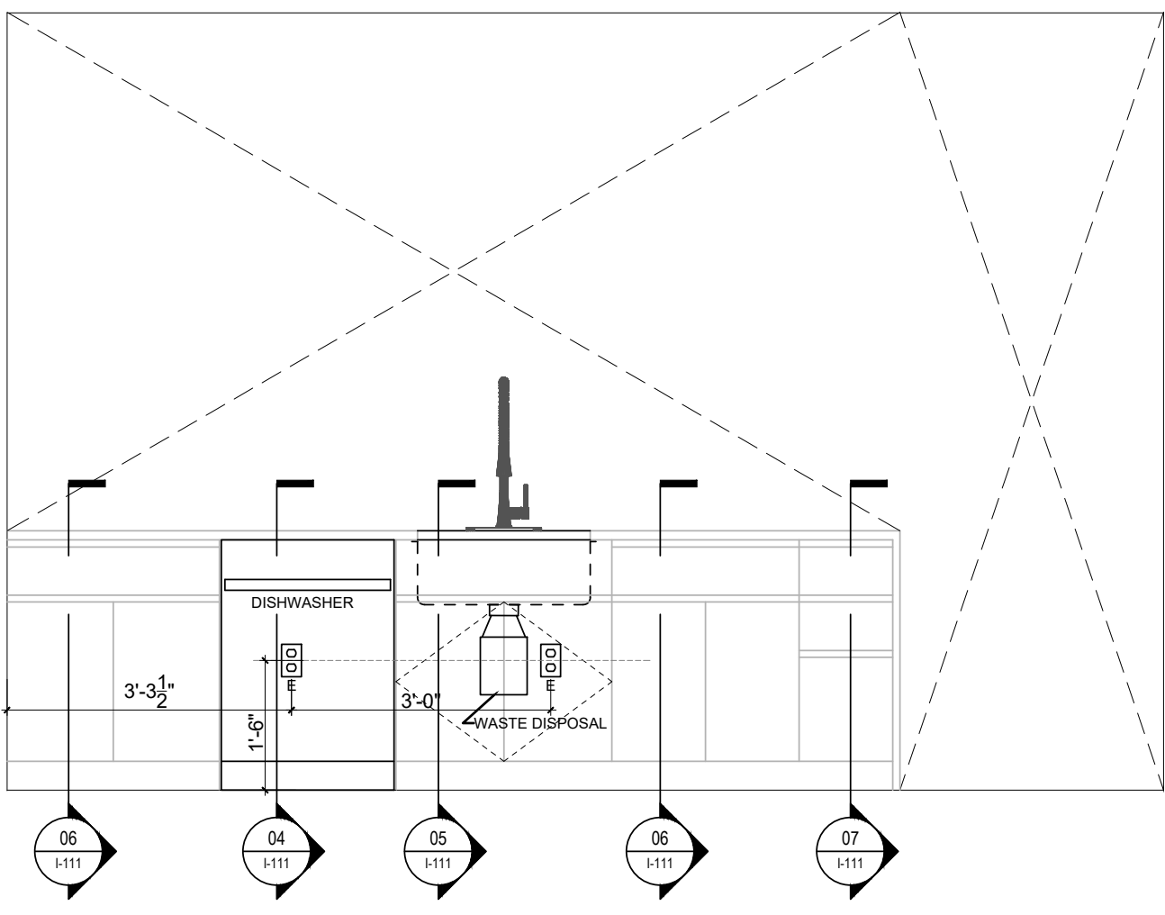
06 SECOND FLOOR KITCHEN NORTH ELEVATION 1/2" = 1'
