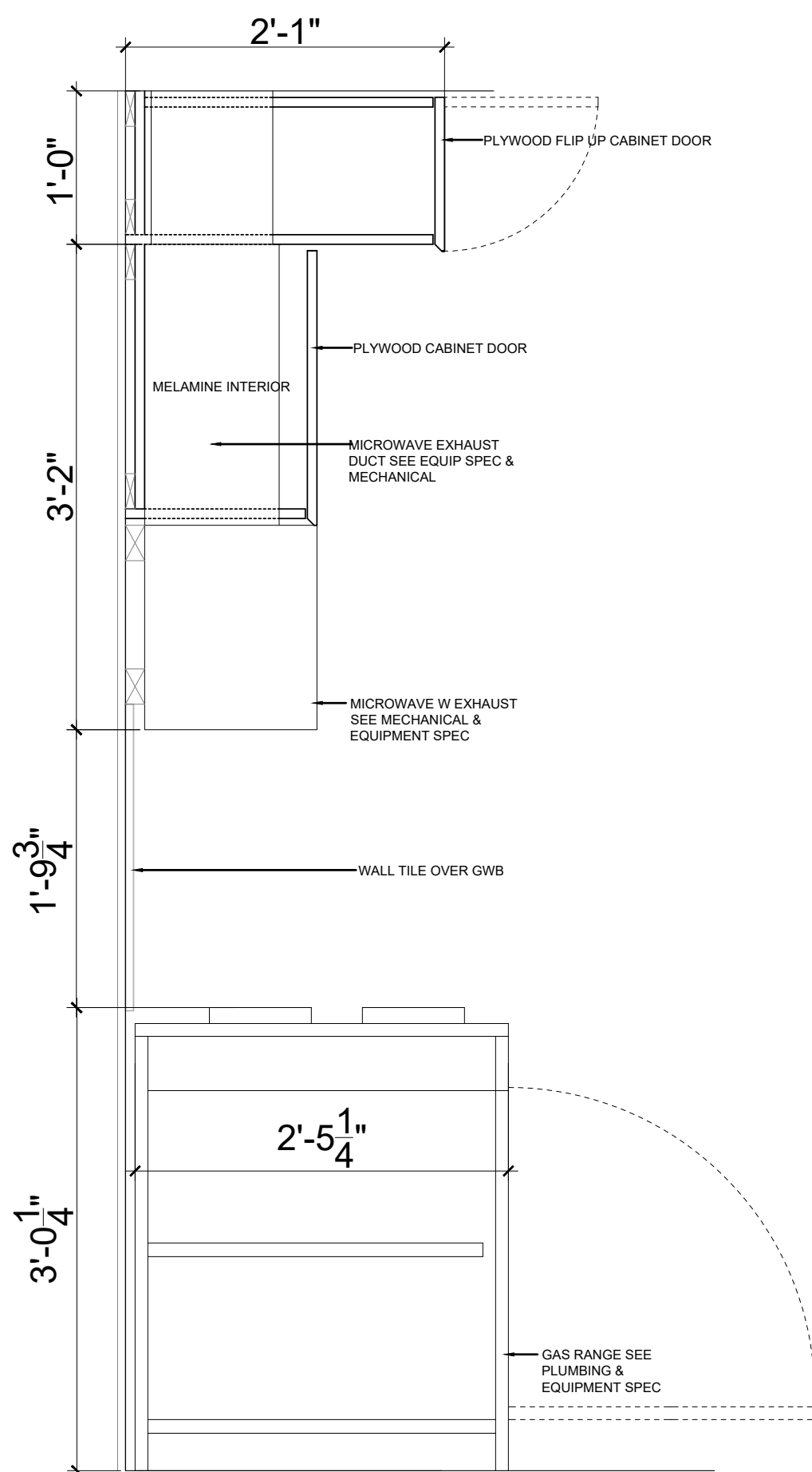
03 MILLWORK SECTION DETAIL 3 - GAS RANGE & MICROWAVE
