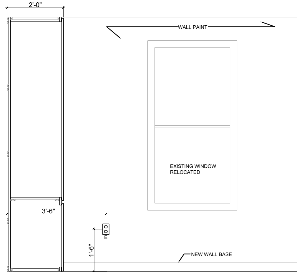
10 FIRST FLOOR GUEST BEDROOM WEST ELEVATION 1/2" = 1'
