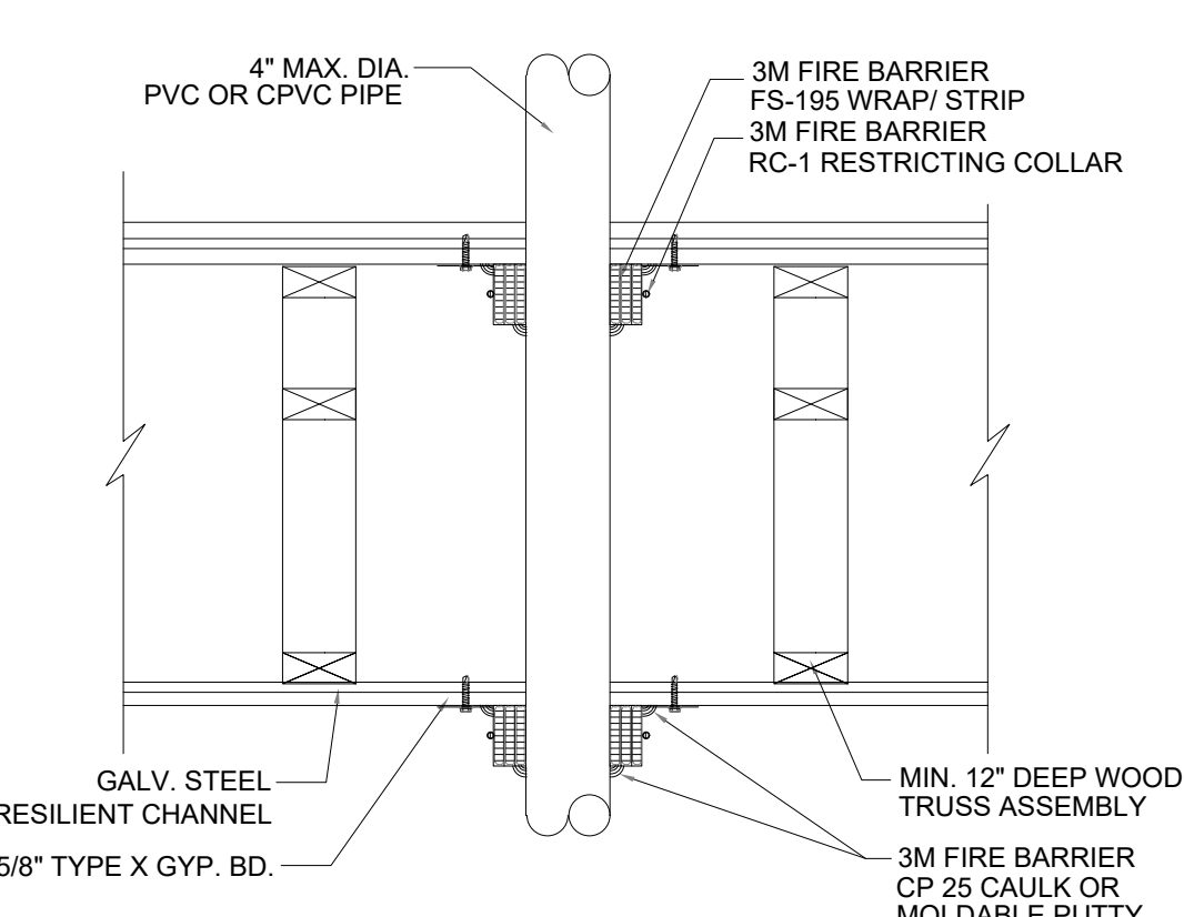
PENETRATION FIRESTOP FOR 4" MAX. DIA. PLASTIC PIPE THROUGH A WOOD & METAL PIPE TRUSS FLOOR/ CEILING ASSEMBLY- 1 HR. RATED U.L. LISTING - F-C-2029
