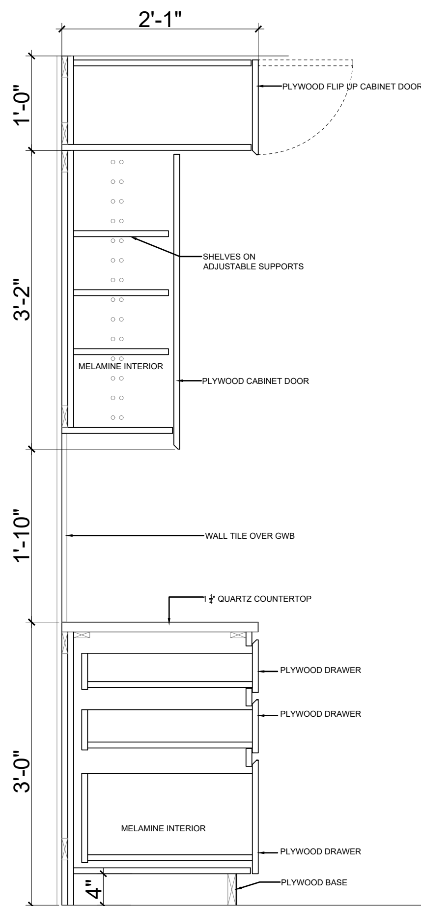
02 MILLWORK SECTION DETAIL 2 - CABINET AND DRAWER
