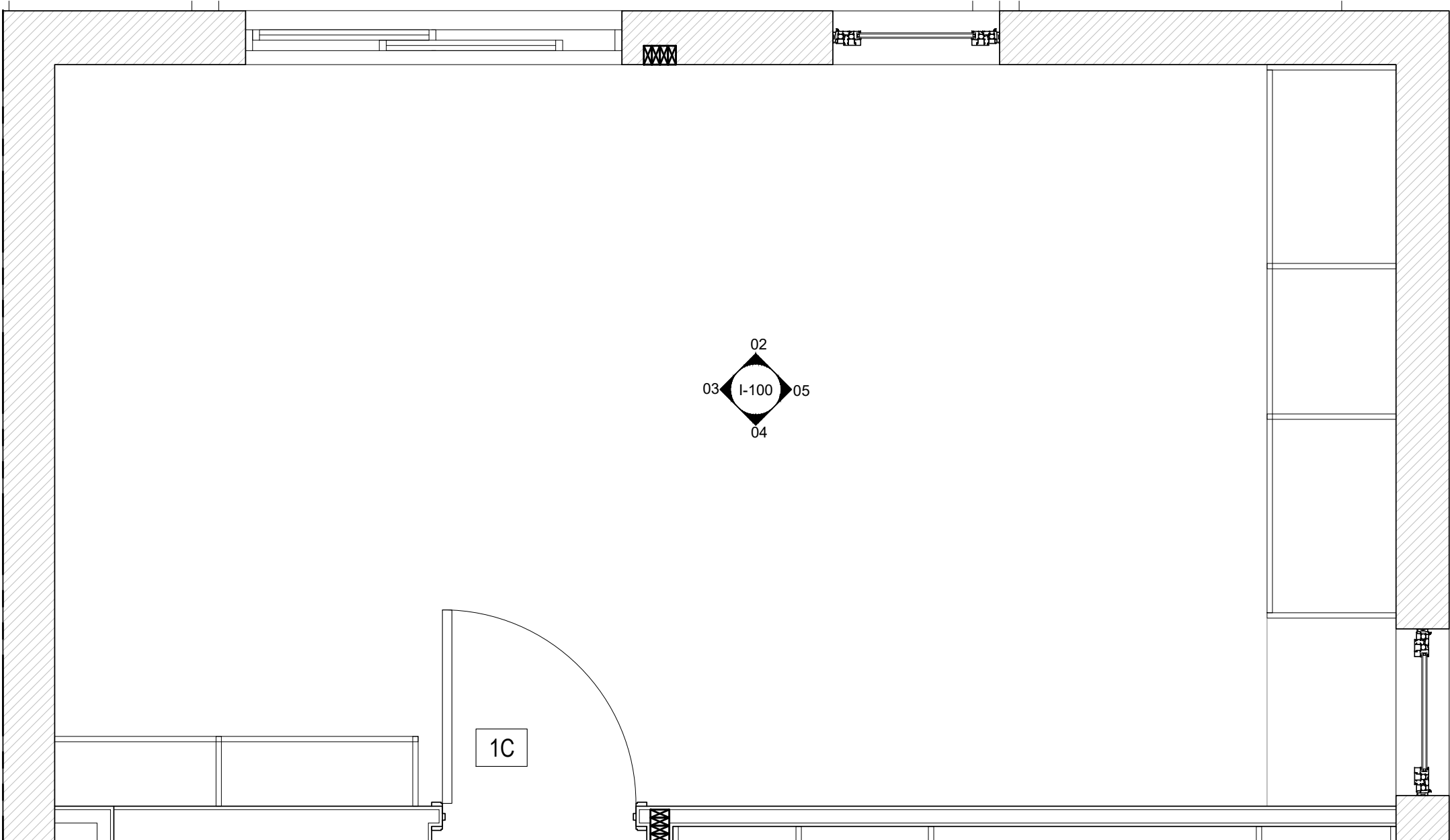
01 FIRST FLOOR MASTER BEDROOM ENLARGED PLAN 1/2" = 1'
