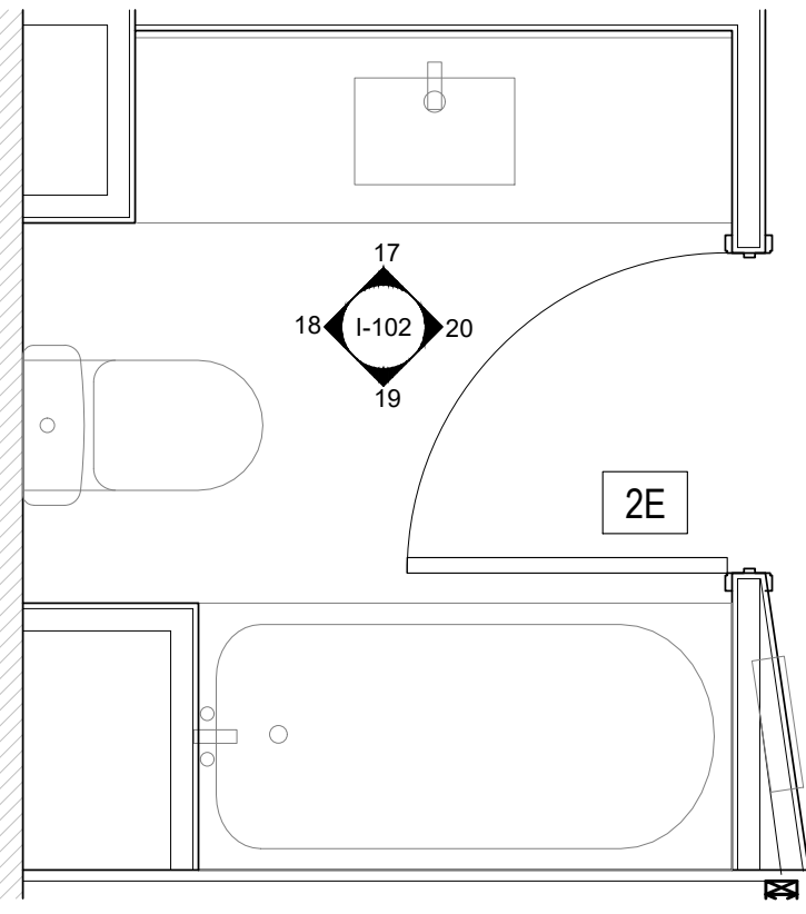
15 SECOND FLOOR GUEST TOILET ENLARGED PLAN 1/2" = 1'
