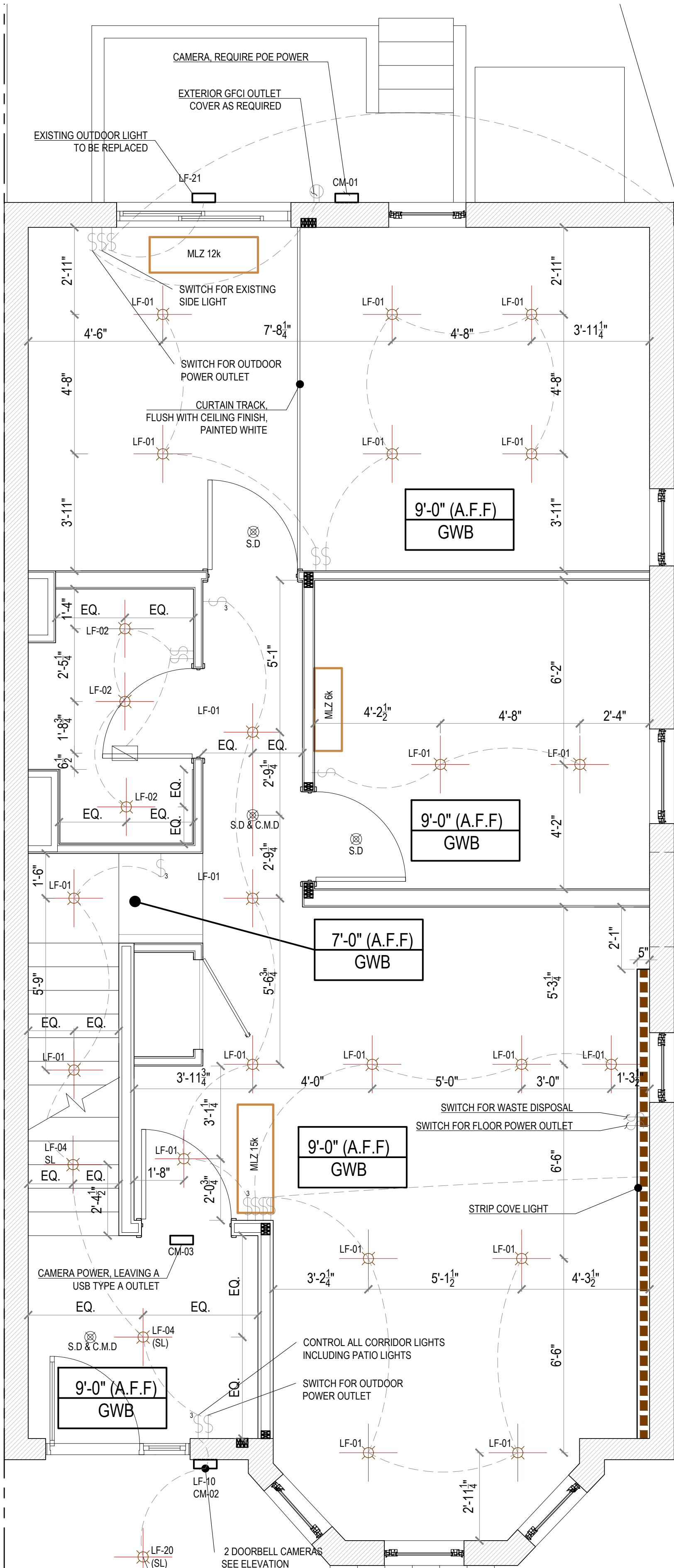
02 1ST FLOOR - RCP
