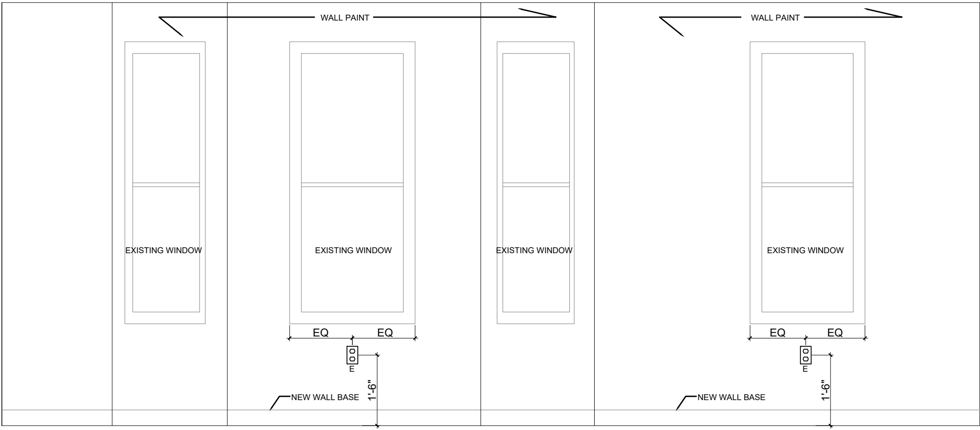
03 SECOND FLOOR LIVING ROOM NORTH ELEVATION 1/2" = 1'
