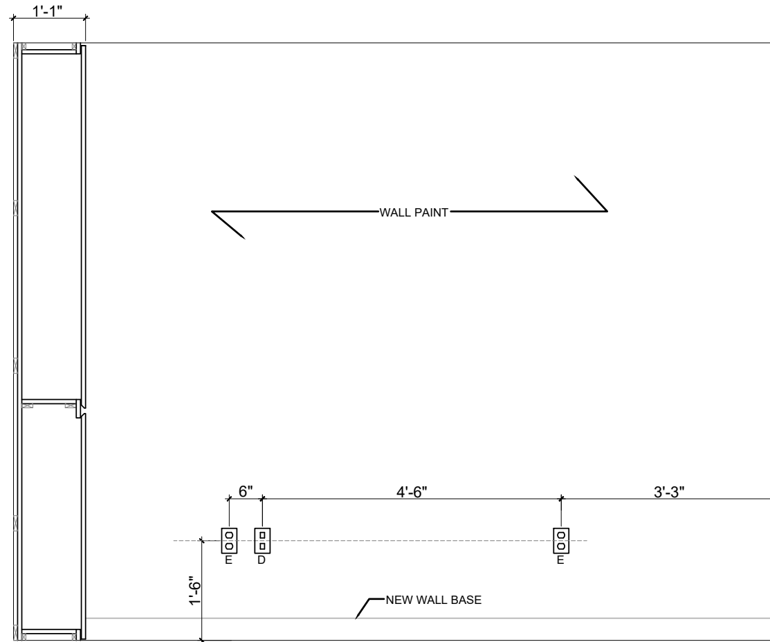
03 FIRST FLOOR MASTER BEDROOM EAST ELEVATION 1/2" = 1'
