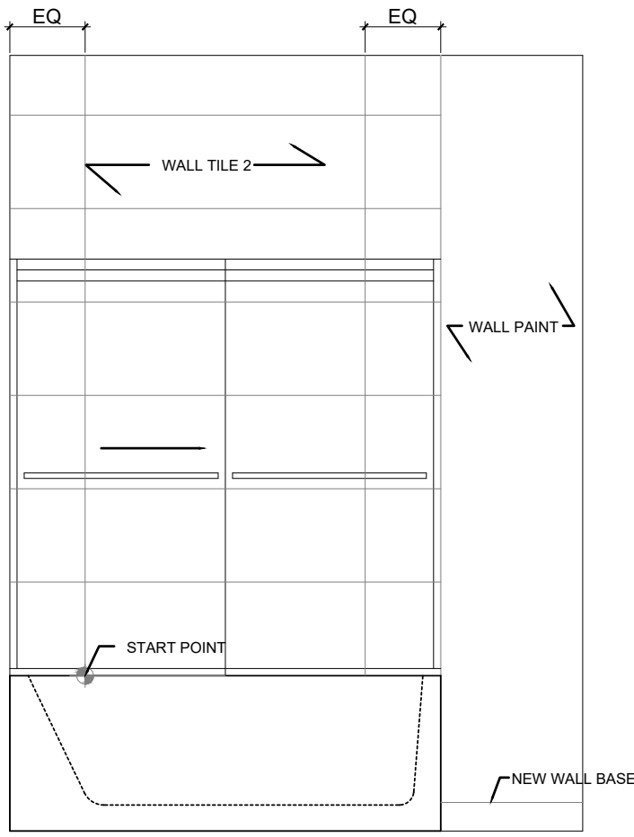
18 SECOND FLOOR GUEST TOILET NORTH ELEVATION 1/2" = 1'
