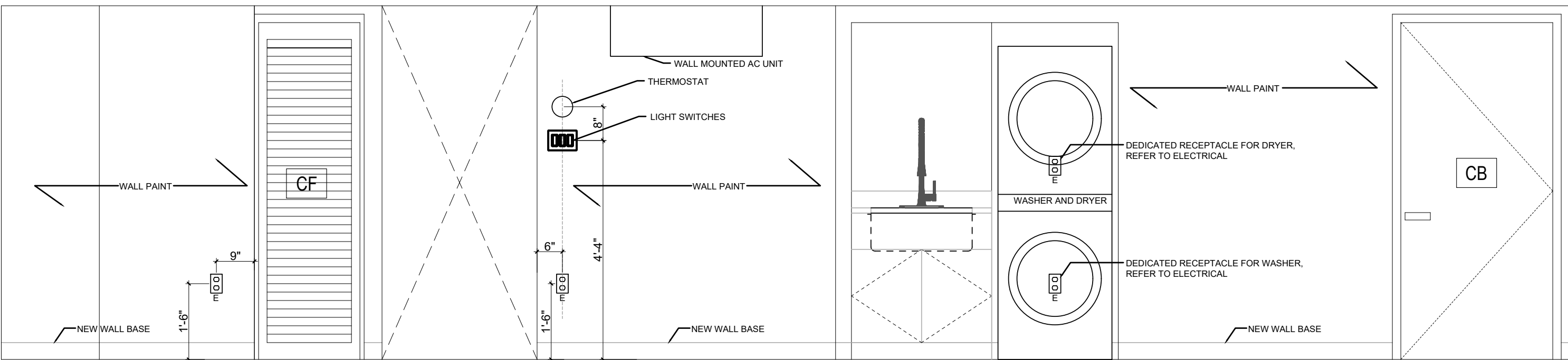
02 CELLAR RECREATION SPACE EAST ELEVATION 1/2" = 1'
