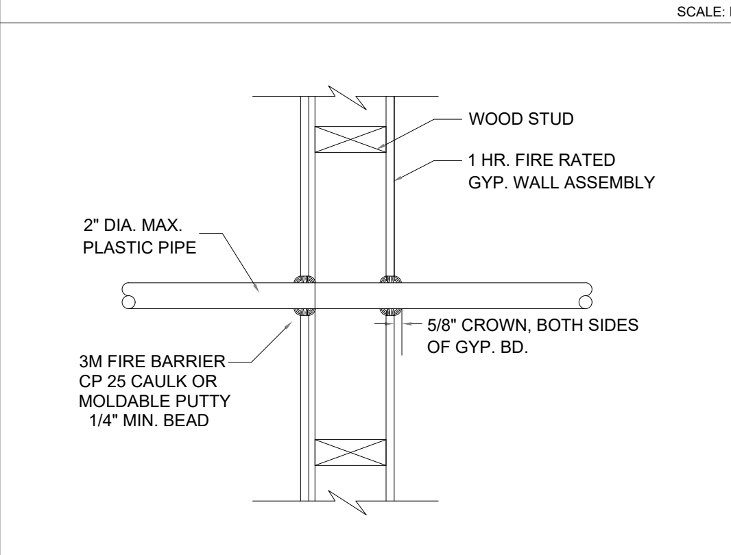
PENETRATION FIRESTOP FOR 2" MAX. DIA. PB, PP, PVC PLASTIC PIPE/ CONDUIT/ COPPER PIPE THROUGH A GYPSUM WALLBOARD ASSEMBLY- 1 HR. RATED U.L. LISTING - W-L-2067
