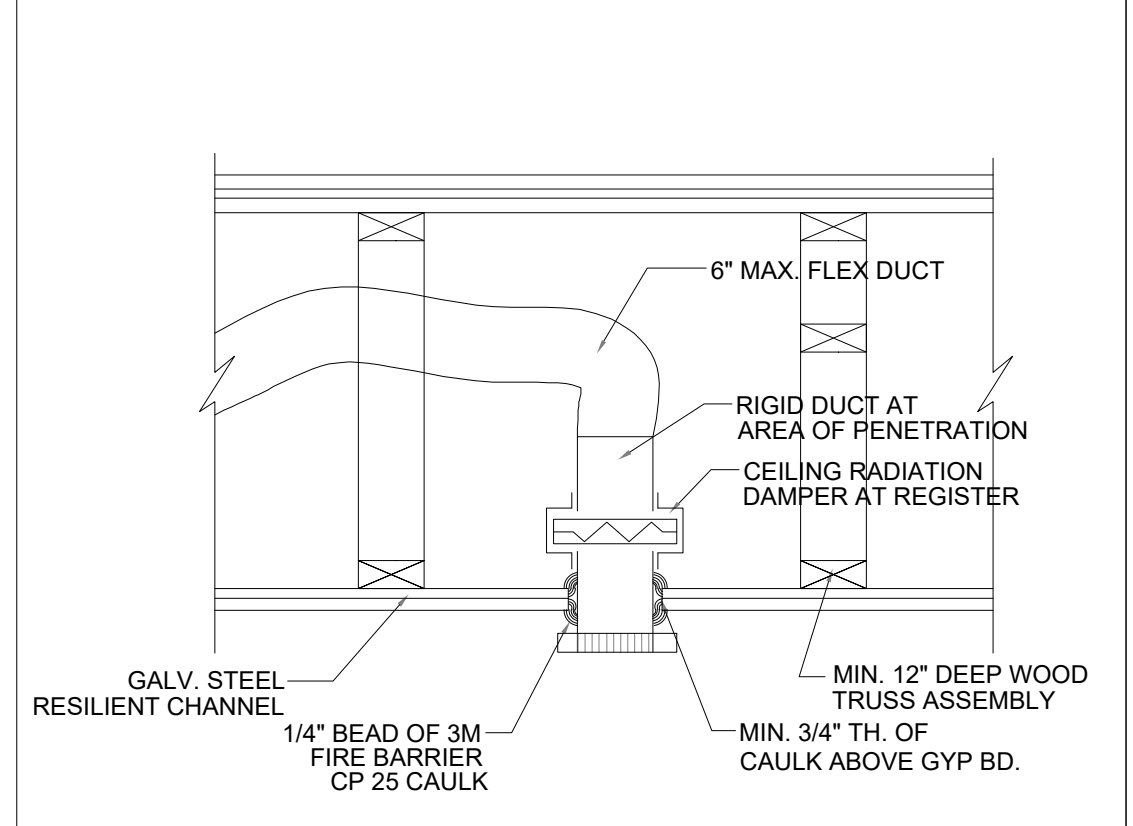
PENETRATION FIRESTOP FOR NOM. 6" MAX. DIA. RIGID SHEET METAL AIR SUPPLY/ RETURN DUCT THROUGH WOOD & METAL PIPE FLOOR ASSEMBLY - 1 HR. RATED U.L. LISTING - F-C-2008
