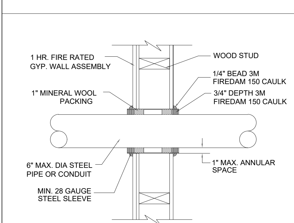
PENETRATION FIRESTOP FOR NOM. 6" MAX. DIA. STEEL PIPE/ COPPER PIPE/ CONDUIT THROUGH A GYPSUM WALLBOARD ASSEMBLY - 1 HR. RATED U.L. LISTING - W-L-1291
