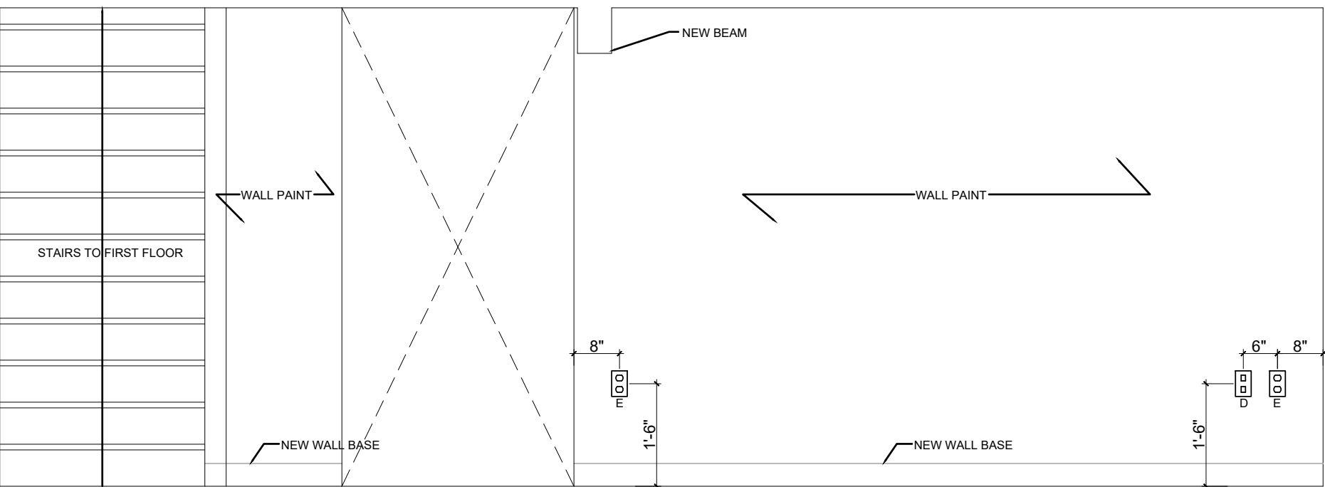
01 CELLAR RECREATION SPACE SOUTH ELEVATION 1/2" = 1'
