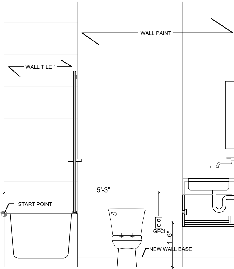
17 SECOND FLOOR GUEST TOILET EAST ELEVATION 1/2" = 1'
