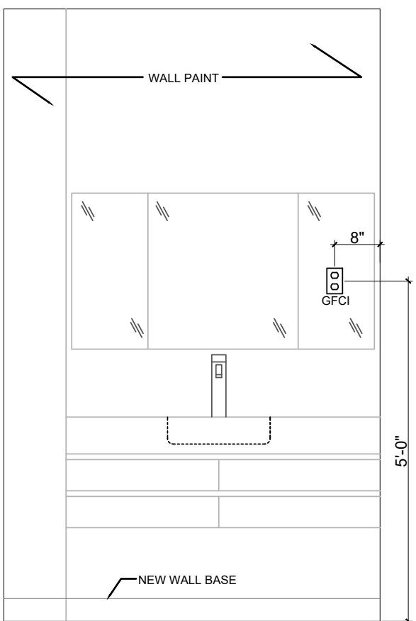
06 FIRST FLOOR TOILET SOUTH ELEVATION 1/12" = 1'
