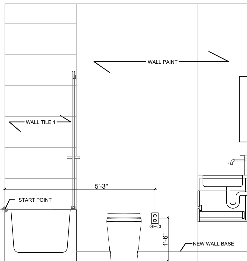
07 FIRST FLOOR TOILET EAST ELEVATION 1/12" = 1'
