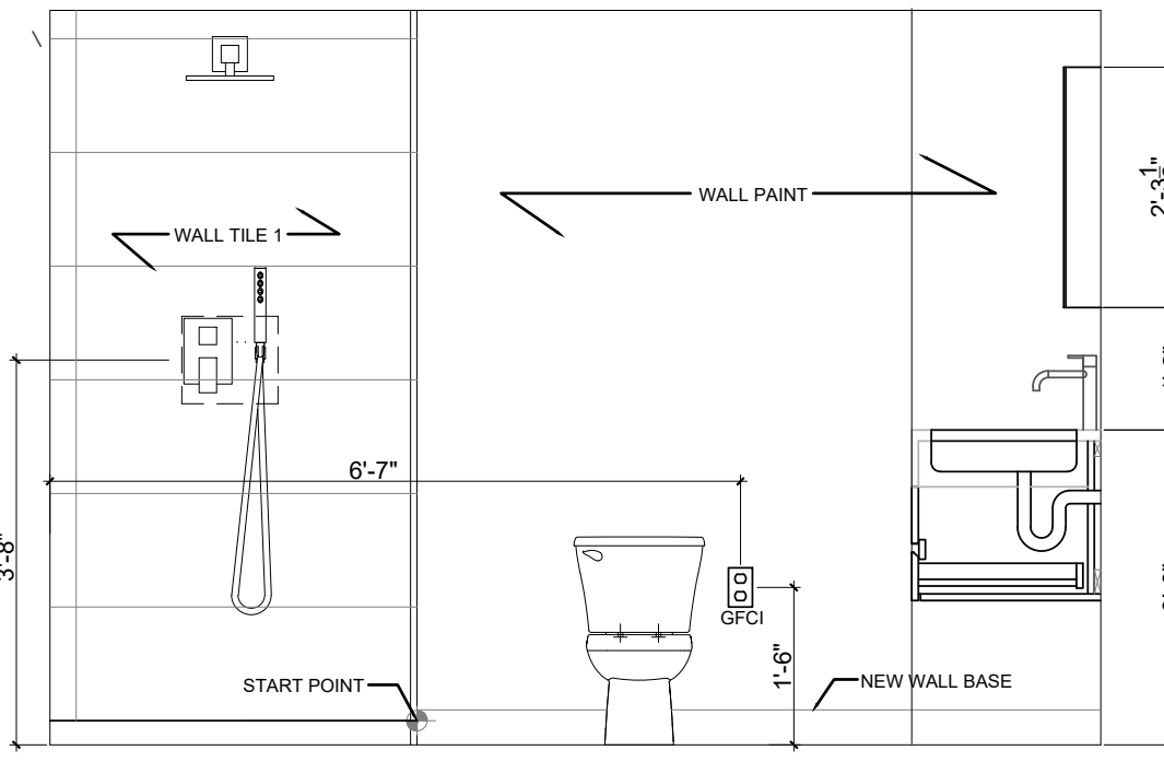
07 CELLAR TOILET EAST ELEVATION 1/2" = 1'
