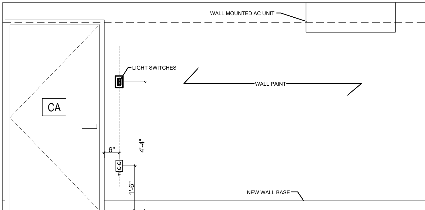
08 CELLAR SMALL STORAGE ROOM EAST ELEVATION 1/2" = 1'
