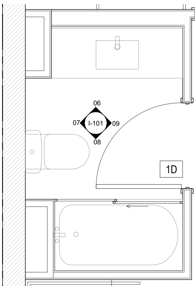
05 FIRST FLOOR TOILET ENLARGED PLAN 1/12" = 1'
