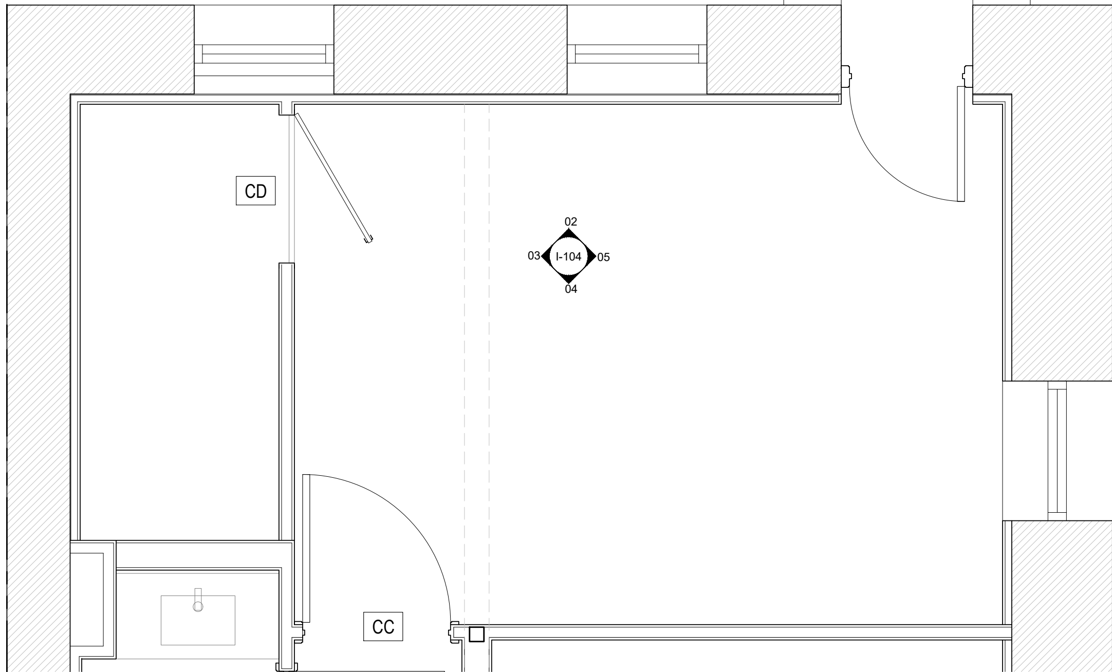
01 CELLAR LARGE STORAGE ROOM ENLARGED PLAN 1/2" = 1'
