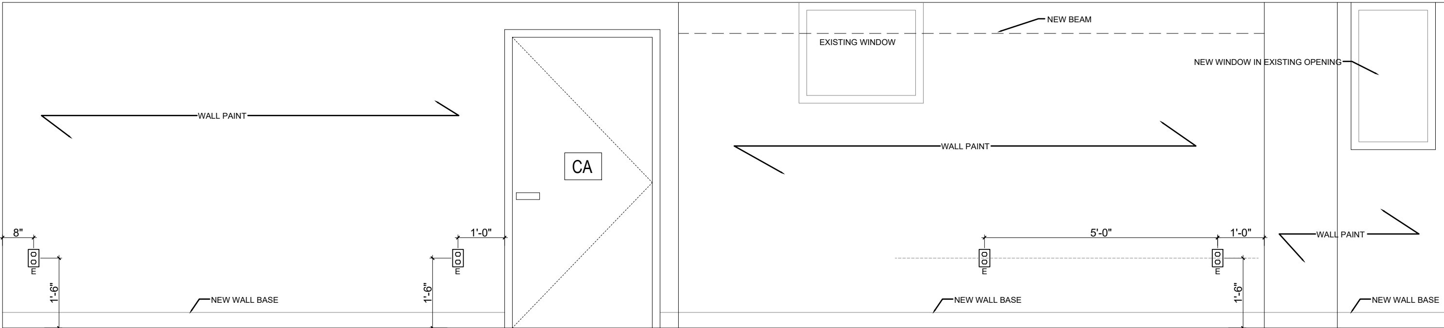
04 SECOND FLOOR LIVING ROOM & CORRIDOR WEST ELEVATION 1/2" = 1'
