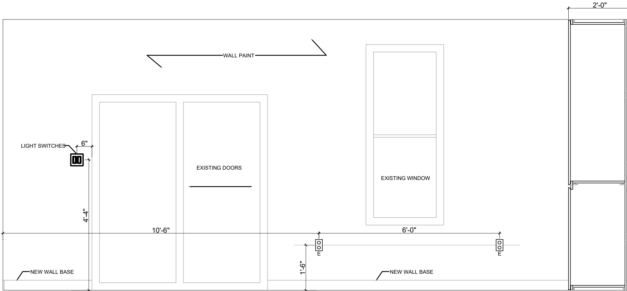
02 FIRST FLOOR MASTER BEDROOM SOUTH ELEVATION 1/2" = 1'
