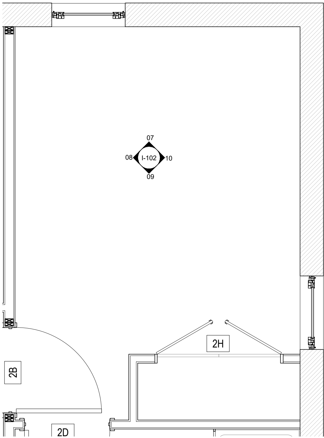
06 SECOND FLOOR MASTER BEDROOM ENLARGED PLAN 1/2" = 1'
