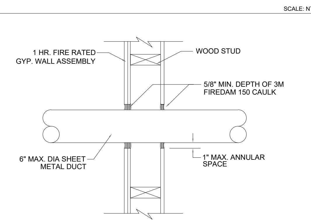
PENETRATION FIRESTOP FOR NOM. 6" MAX. DIA. RIGID SHEET METAL AIR INTAKE / EXHAUST DUCT THROUGH A GYPSUM WALLBOARD ASSEMBLY - 1 HR. RATED U.L. LISTING - W-L-1167
