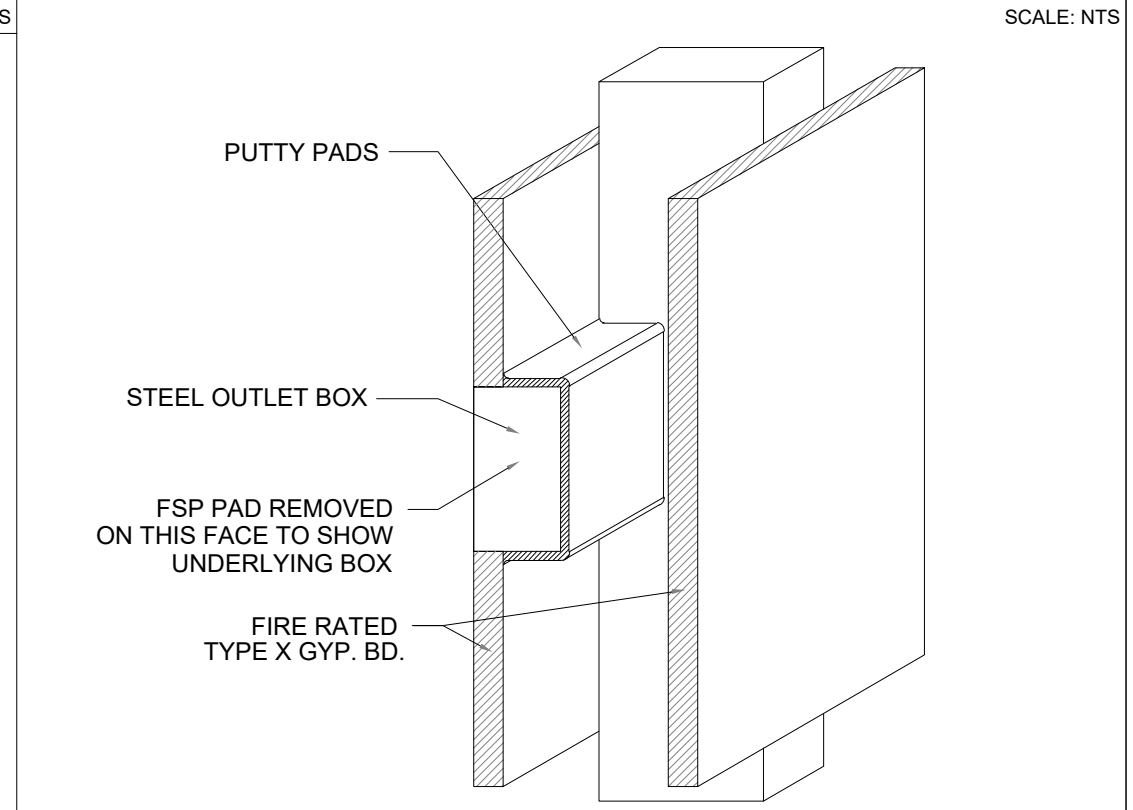
GYPSUM WALL ELECTRICAL OUTLET BOX WALLBOARD ASSEMBLY- 1 HR. ASSEMBLY
