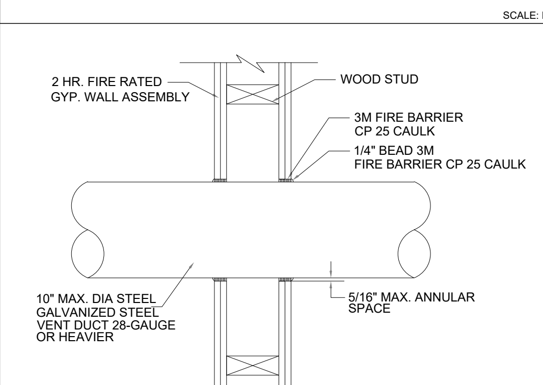
PENETRATION FIRESTOP FOR 10" MAX. DIA. STEEL VENT DUCT THROUGH A GYPSUM WALLBOARD ASSEMBLY - 2 HR. RATED U.L. LISTING - NO. 147
