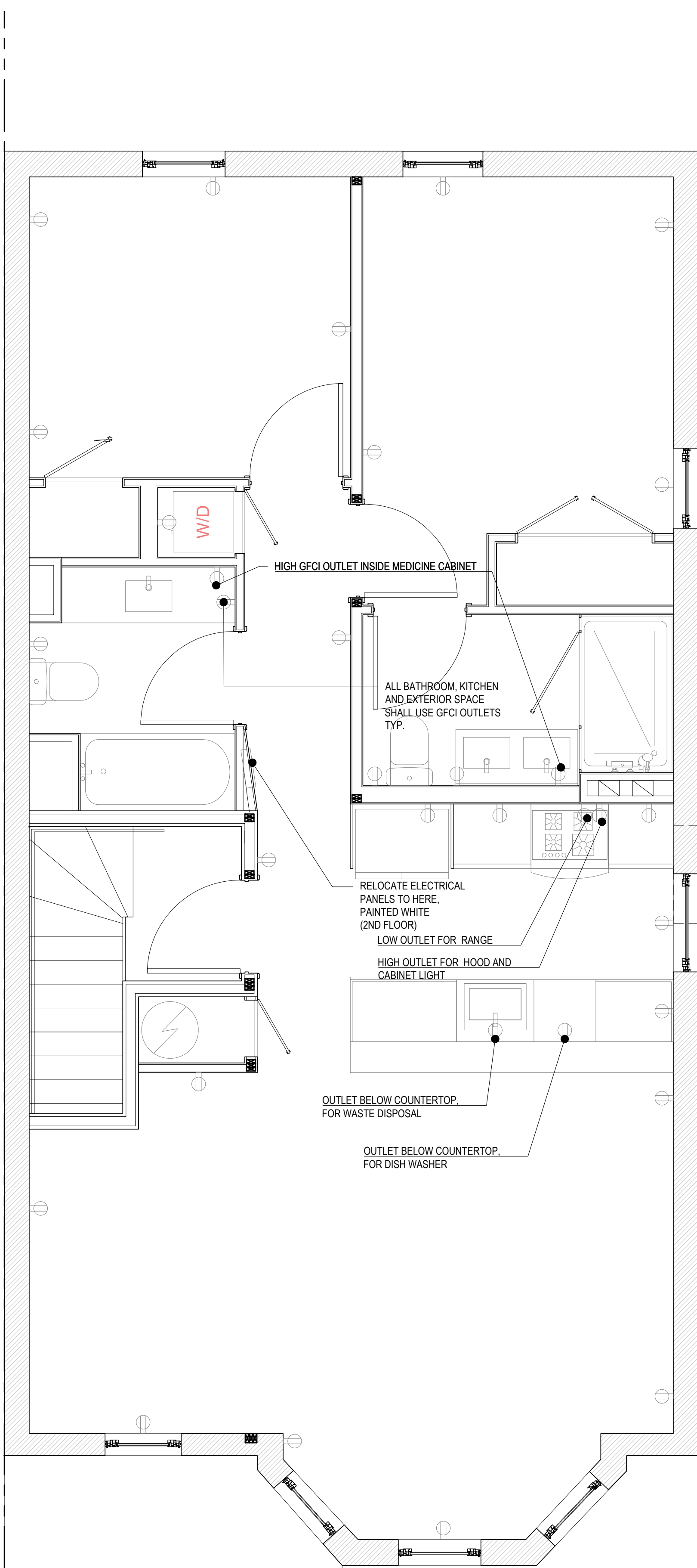
03 2ND FLOOR - POWER PLAN 3/16" = 1'
