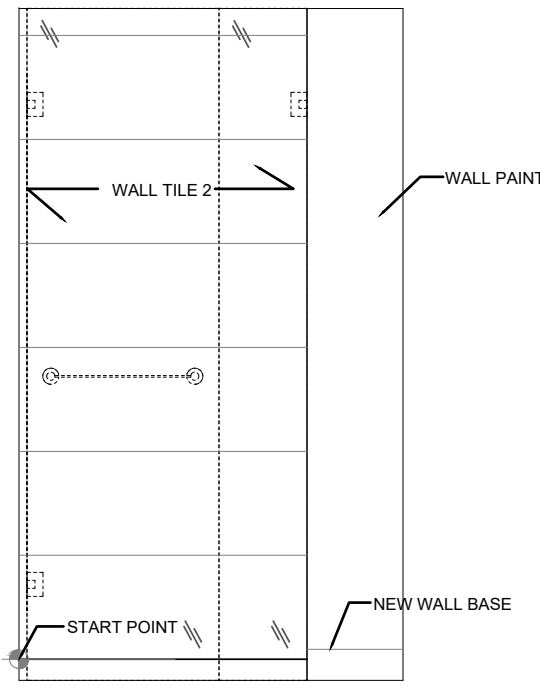
08 CELLAR TOILET NORTH ELEVATION 1/2" = 1'
