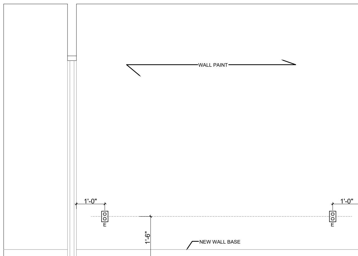
03 SECOND FLOOR GUEST BEDROOM EAST ELEVATION 1/2" = 1'
