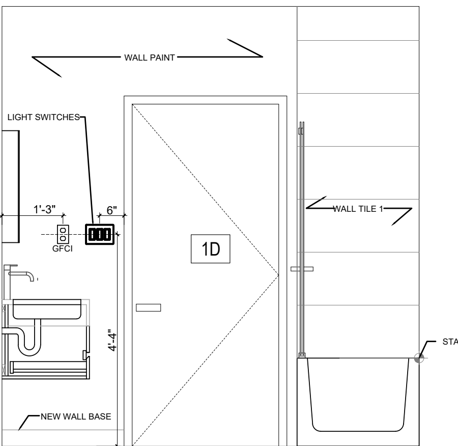
09 FIRST FLOOR TOILET EAST ELEVATION 1/12" = 1'
