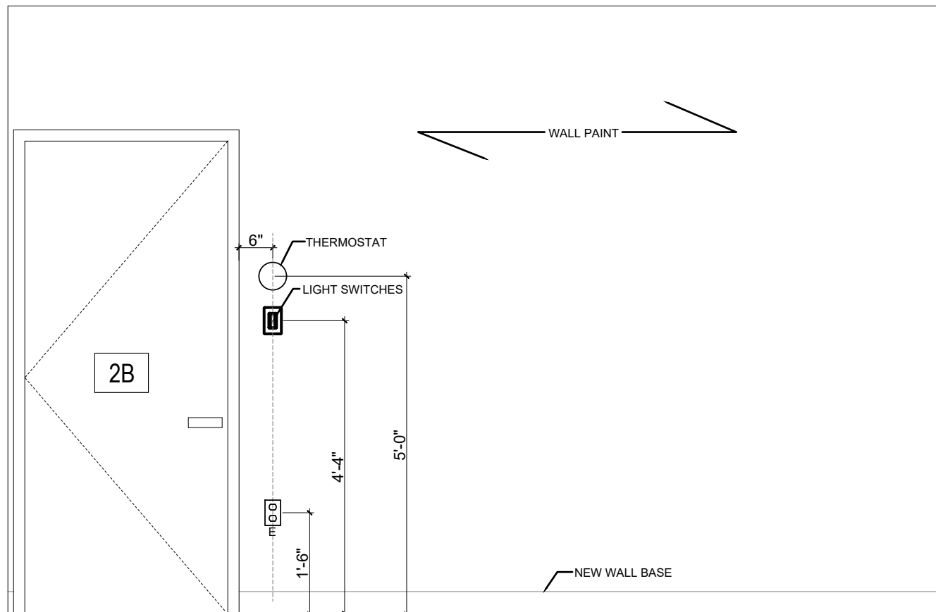
08 SECOND FLOOR MASTER BEDROOM EAST ELEVATION 1/2" = 1'
