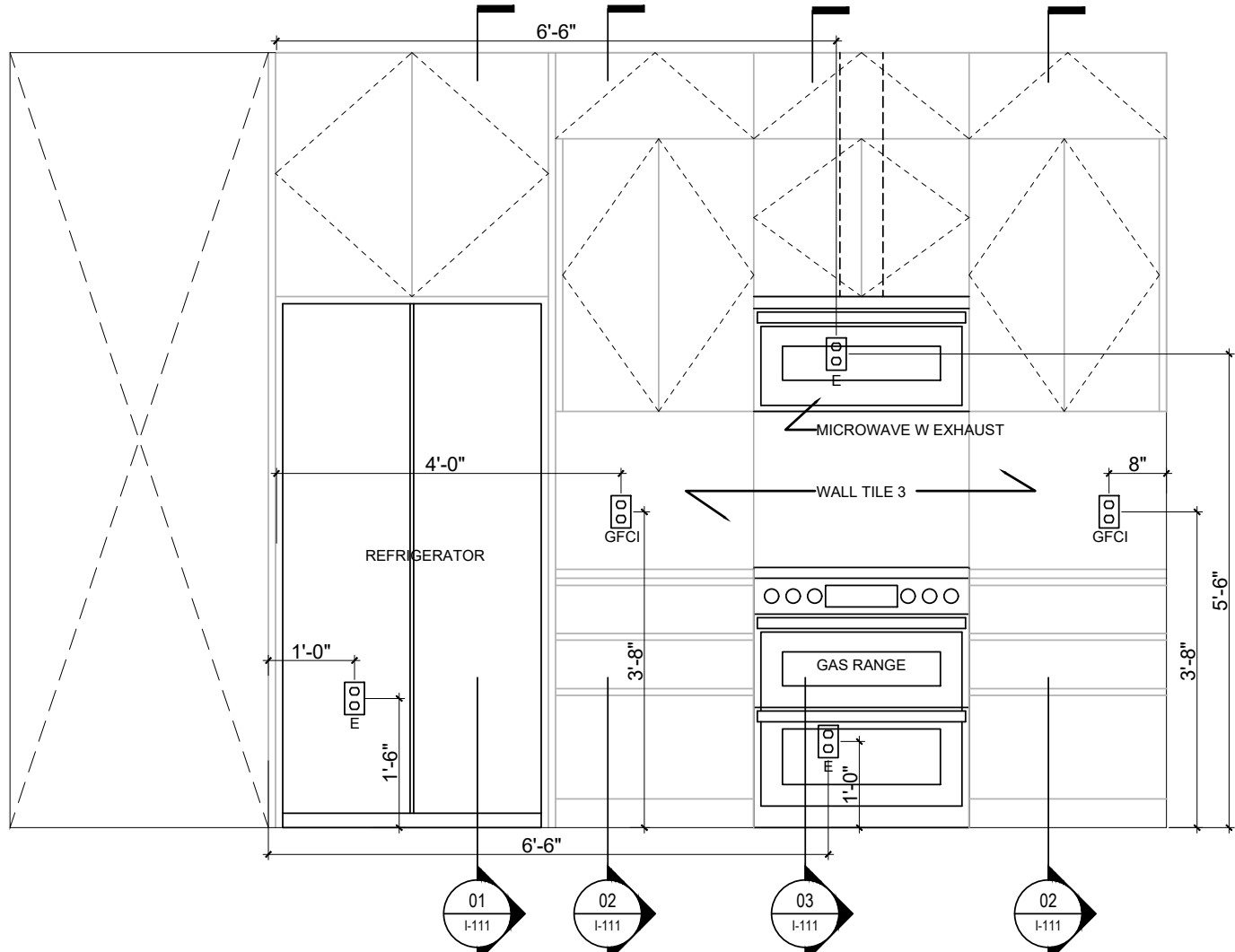
05 SECOND FLOOR KITCHEN SOUTH ELEVATION 1/2" = 1'
