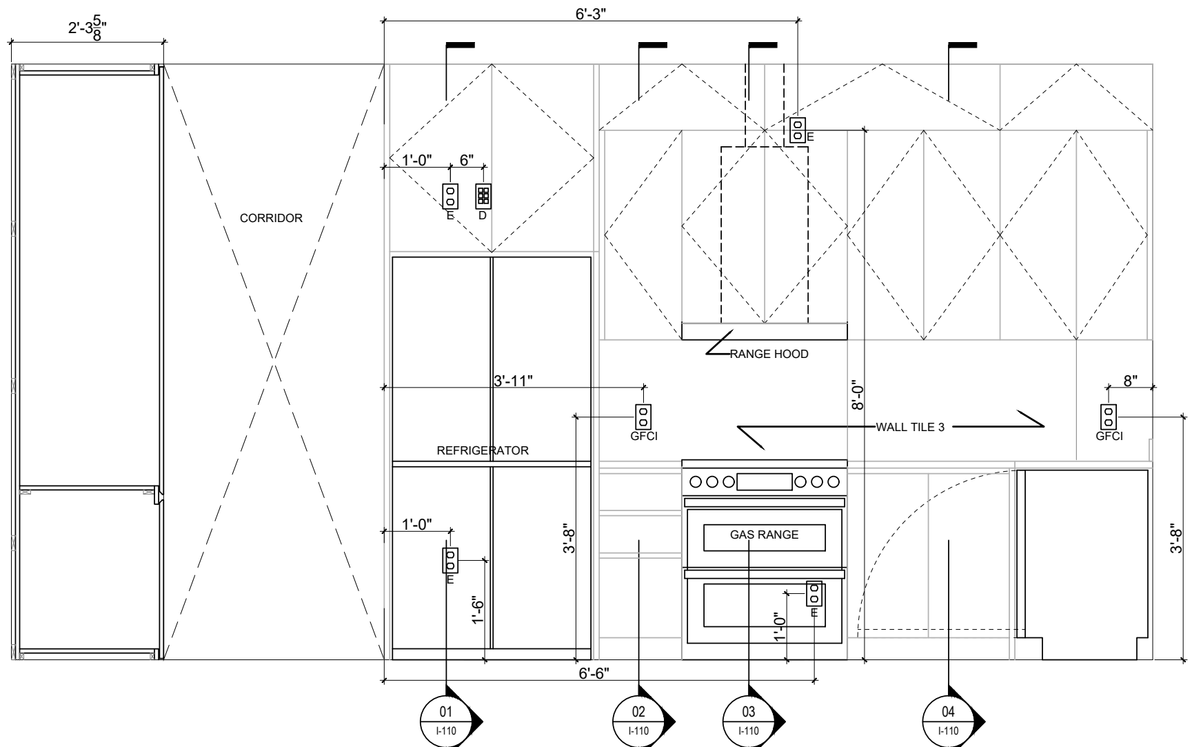
01 FIRST FLOOR LIVING ROOM & KITCHEN SOUTH ELEVATION 1/12" = 1'
