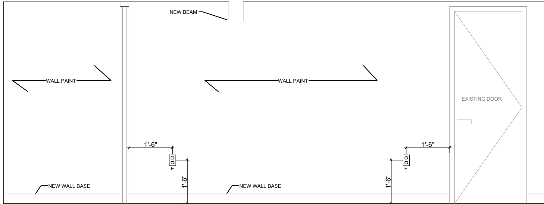
02 CELLAR LARGE STORAGE ROOM SOUTH ELEVATION 1/2" = 1'
