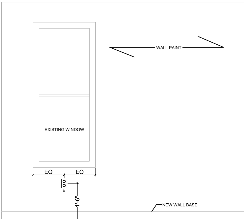
07 SECOND FLOOR MASTER BEDROOM SOUTH ELEVATION 1/2" = 1'
