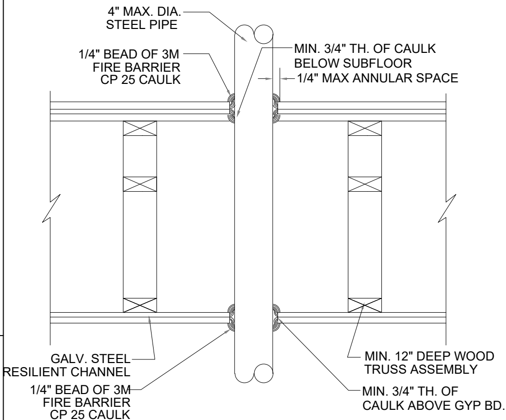
PENETRATION FIRESTOP OF A 4" MAX. DIA. STEEL PIPE 3" COPPER PIPE 4" CAST IRON PIPE STEEL EMT CONDUIT THROUGH A WOOD & METAL PIPE TRUSS FLOOR/ CEILING ASSEMBLY- 1 HR. RATED U.L. LISTING - F-C-1006
