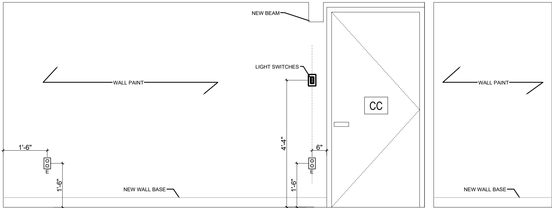
04 CELLAR LARGE STORAGE ROOM NORTH ELEVATION 1/2" = 1'
