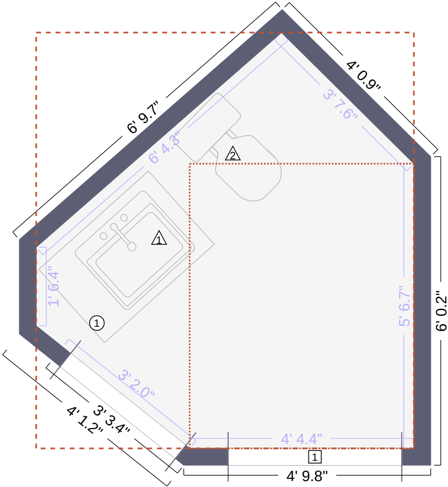
Bathroom Floor Plan
