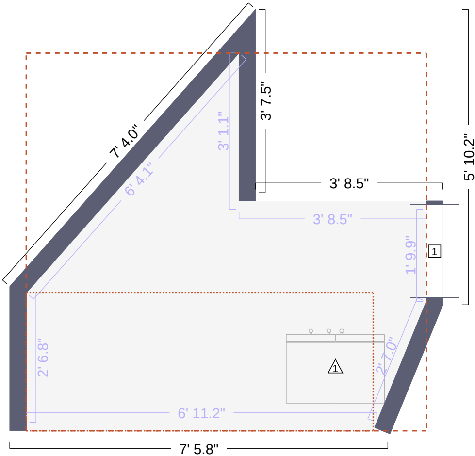
Other 4 Floor Plan
