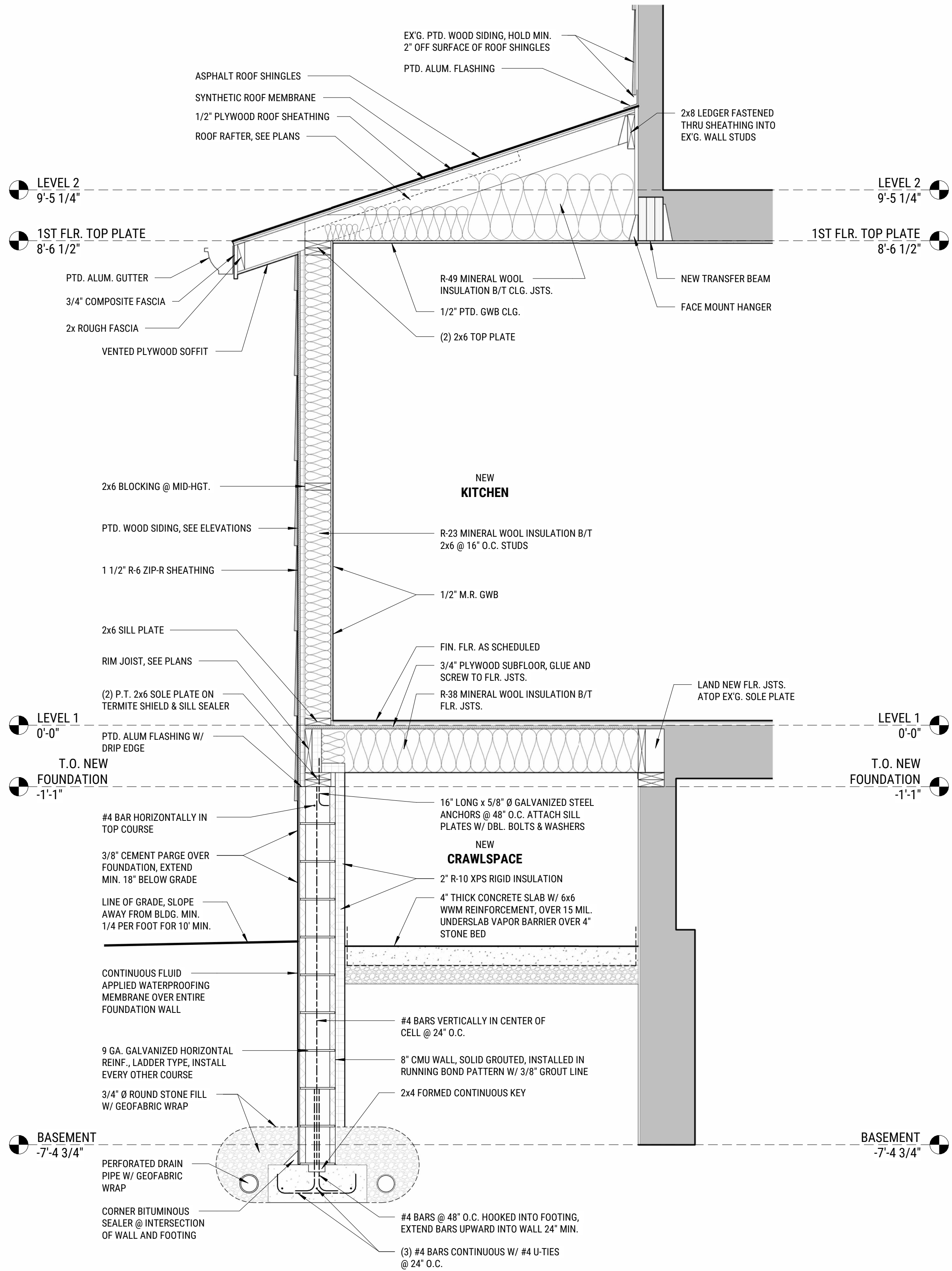
2 SECTION - REAR KITCHEN A300 3/4" = 1'-0"
