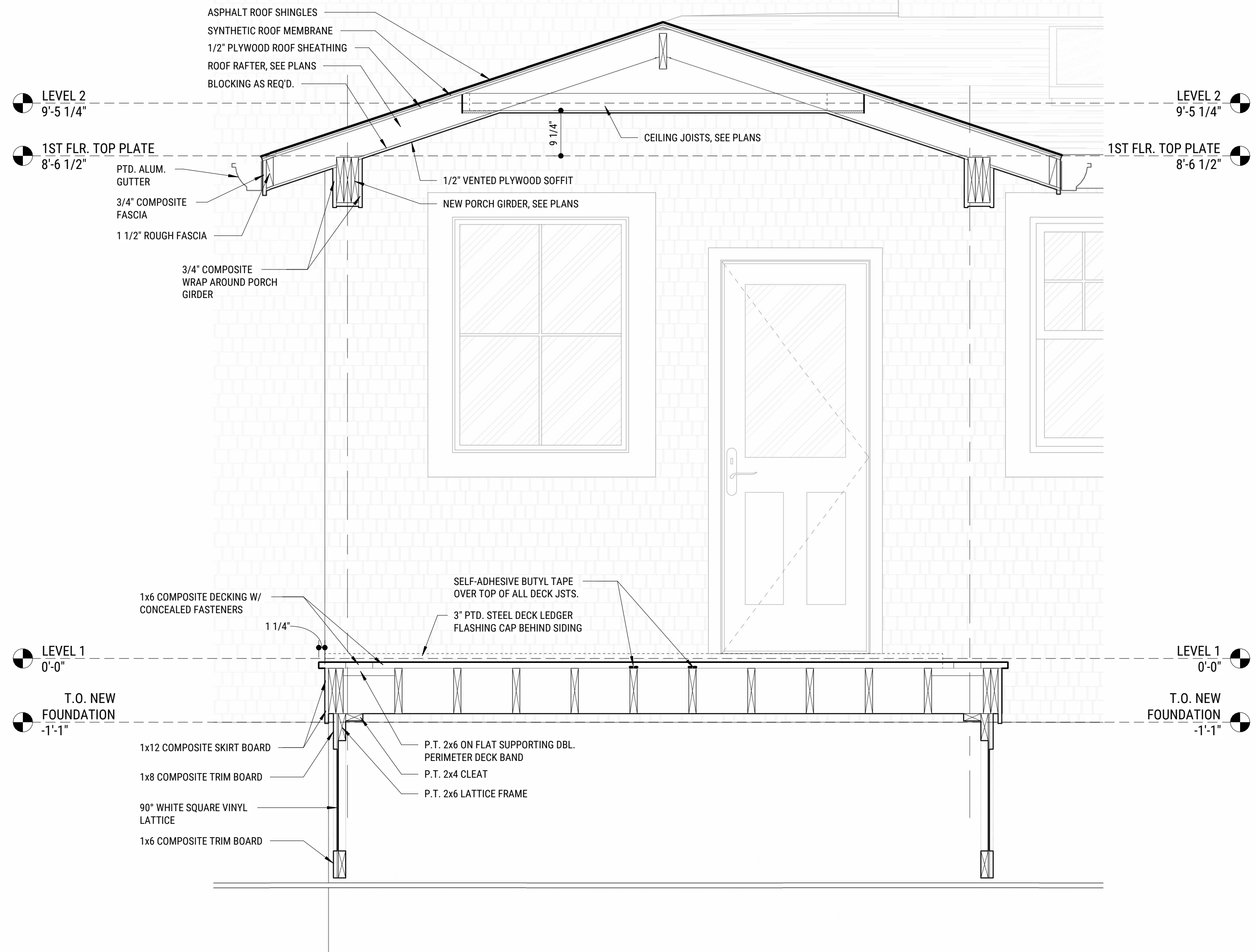
1 SECTION - NEW PORCH A300 3/4" = 1'-0"
