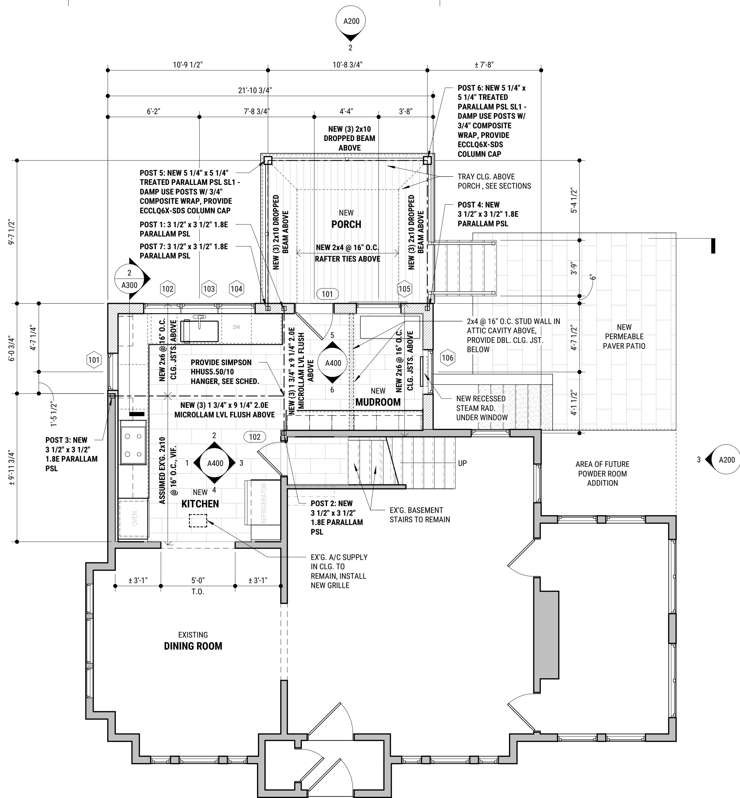
1 CONSTRUCTION PLAN - LEVEL 1 1/4" = 1'-0"
