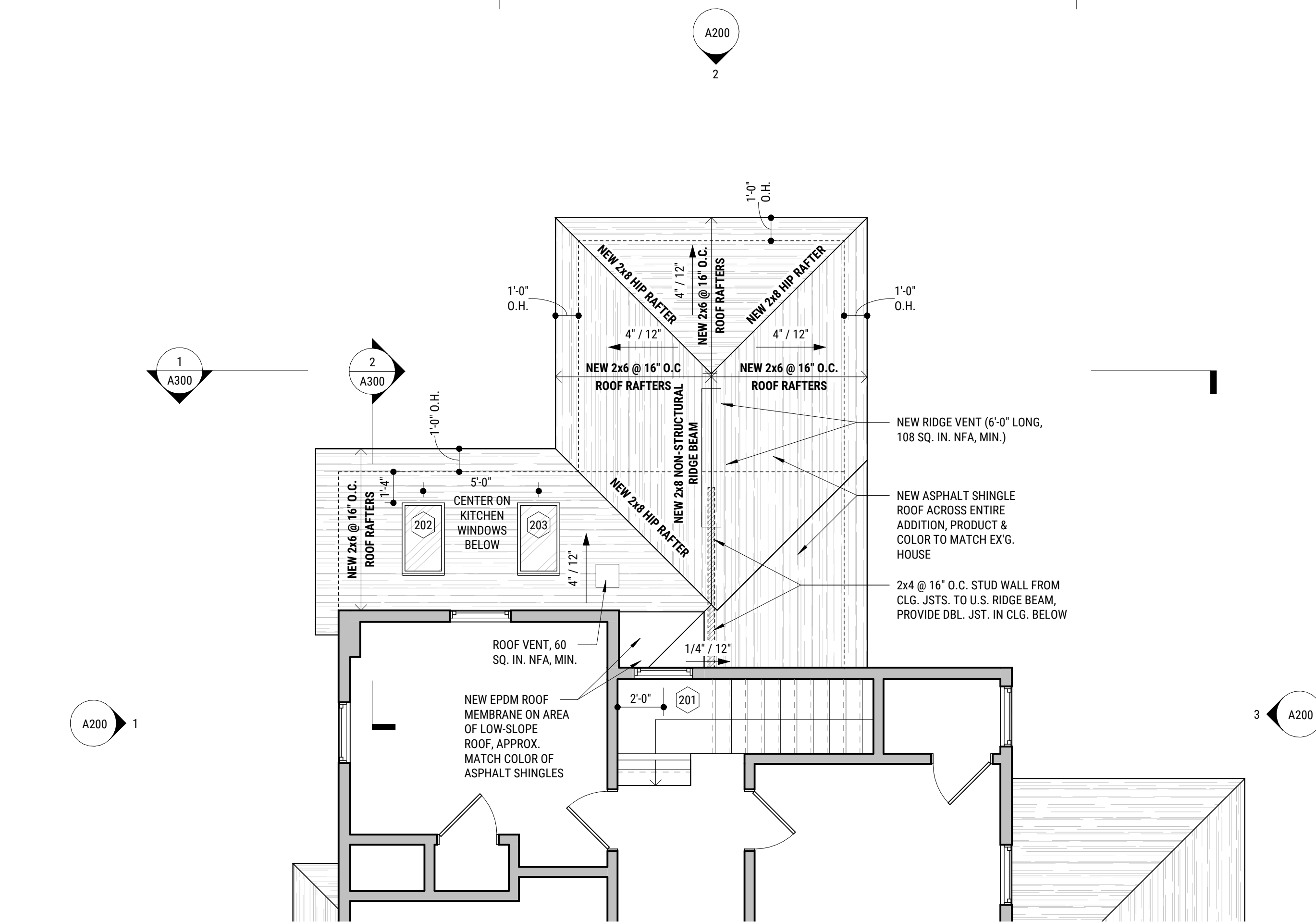
3 CONSTRUCTION PLAN - LEVEL 2 1/4" = 1'-0"
