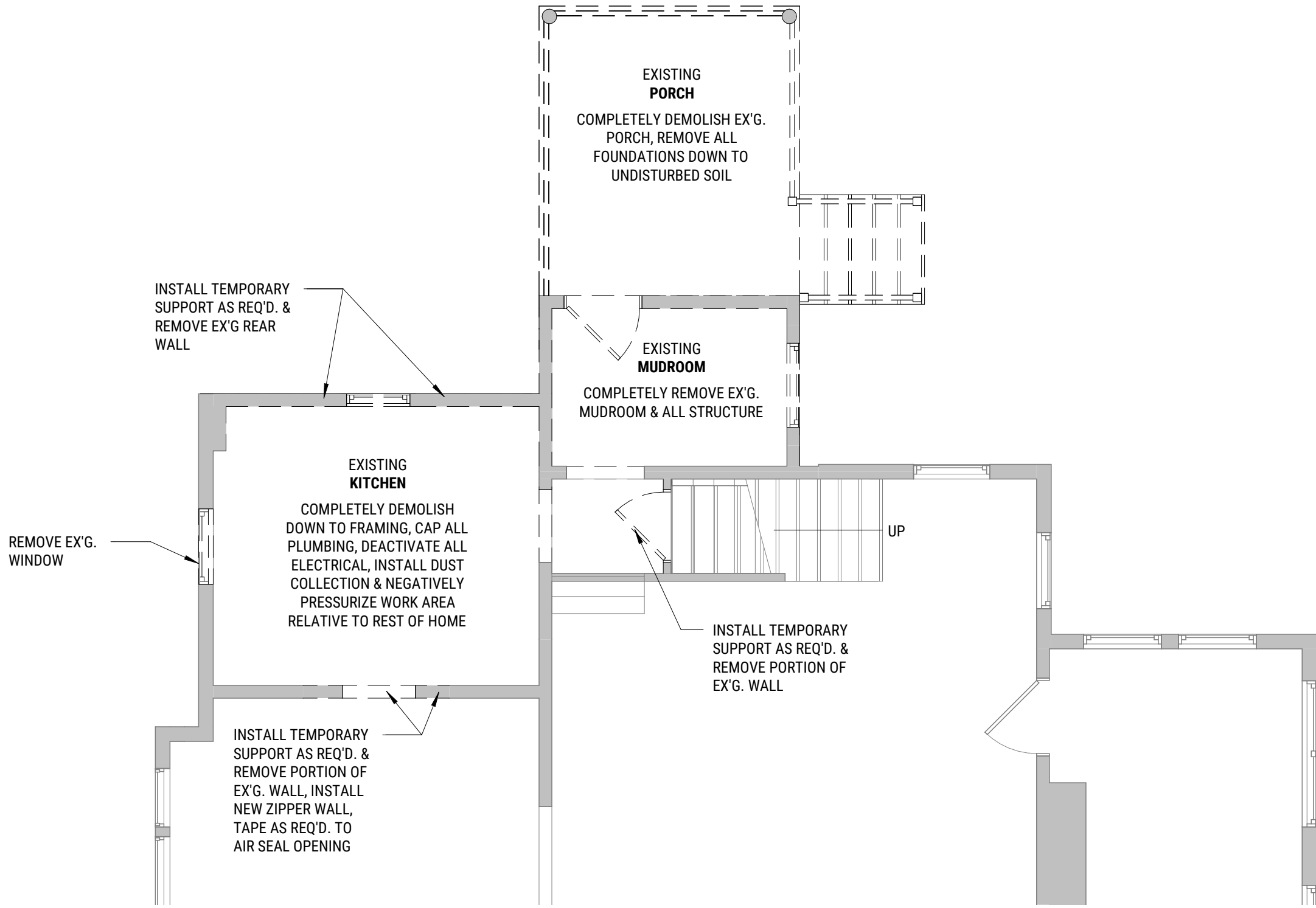
1 DEMOLITION PLAN - LEVEL 1 A050 1/4" = 1'-0"
