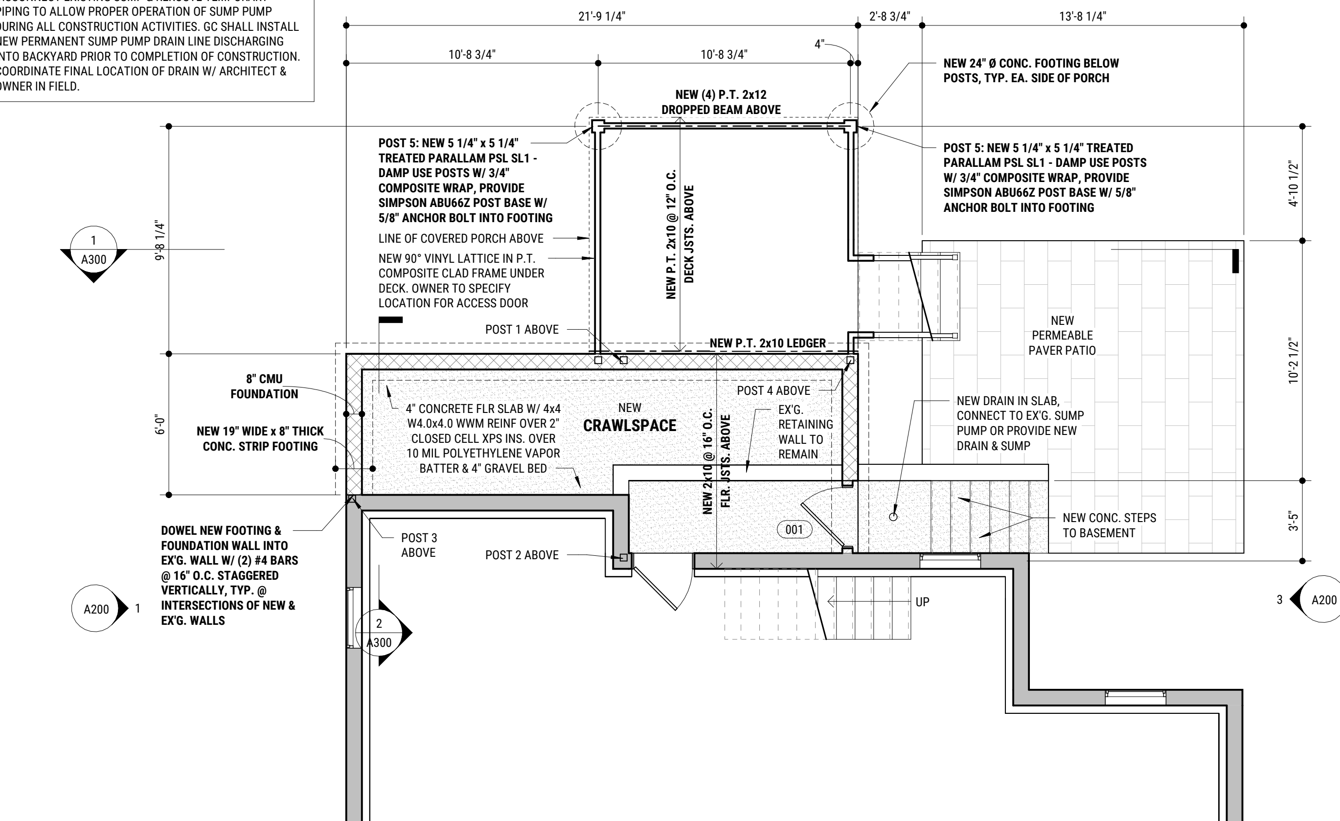
2 CONSTRUCTION PLAN - BASEMENT 1/4" = 1'-0"
