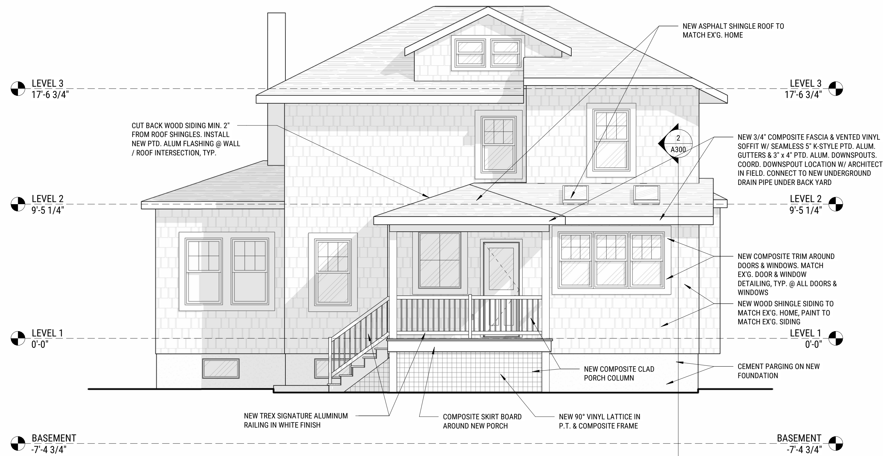
2 A200 EXTERIOR ELEVATION - REAR 1/4" = 1'-0"
