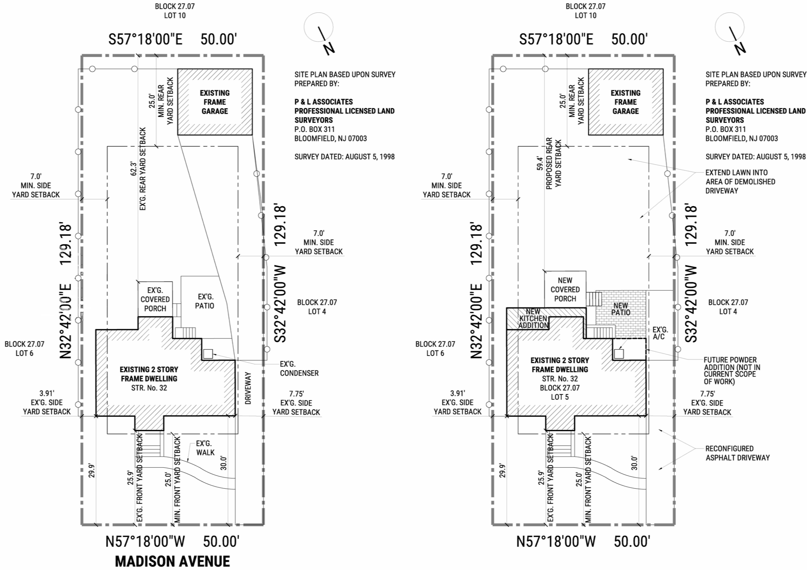
1 EXISTING SITE PLAN SCALE: 1/16" = 1'-0"
