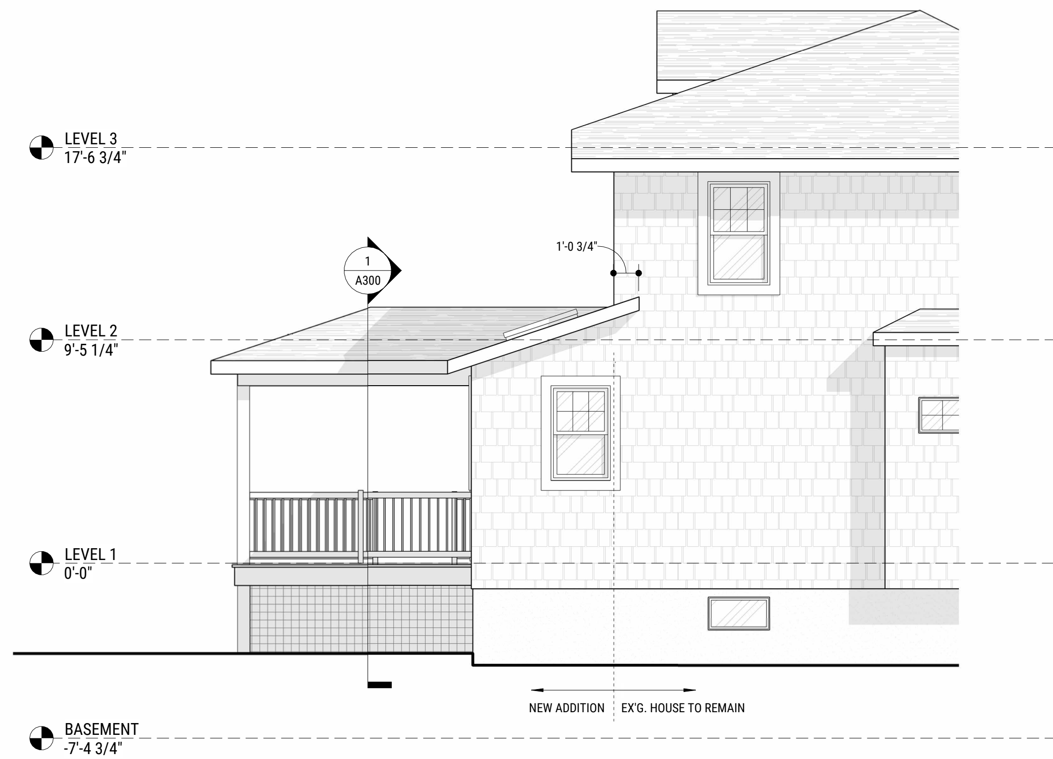
1 A200 EXTERIOR ELEVATION - LEFT 1/4" = 1'-0"
