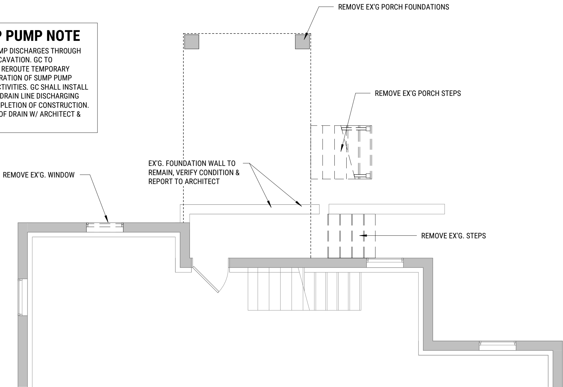
2 DEMOLITION PLAN - BASEMENT A050 1/4" = 1'-0"
