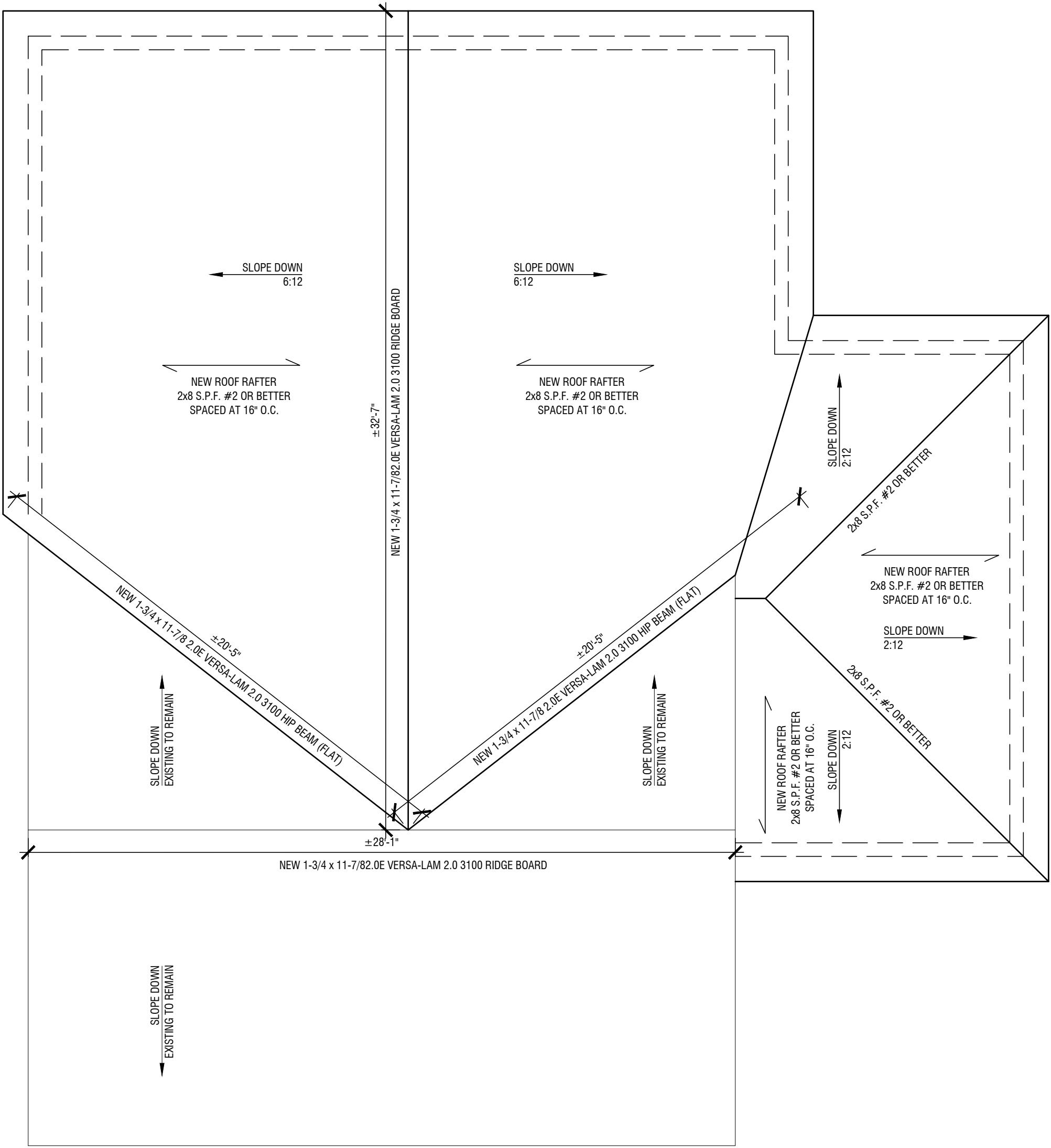
3 PROPOSED PLAN - ROOF SCALE: 1/4"=1'-0"
