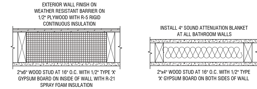
1 EXTERIOR WALL TYPE TYPICAL
