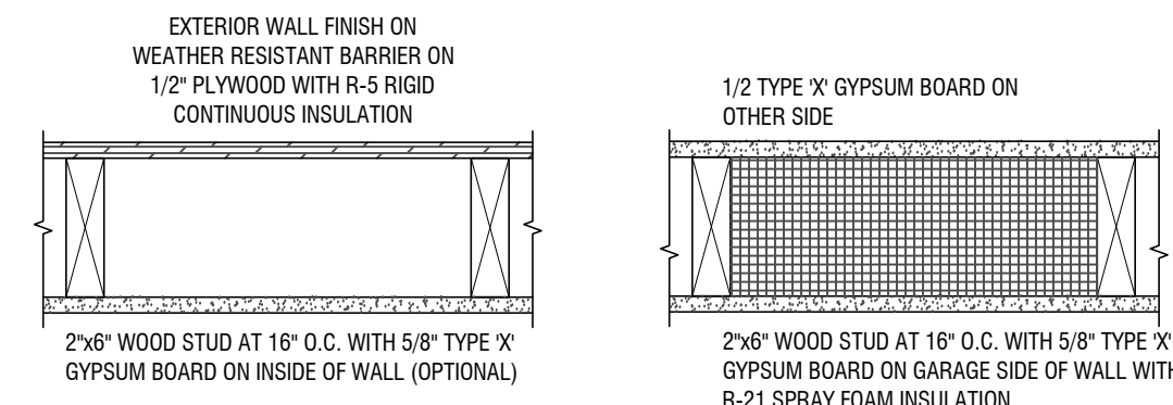
3 EXTERIOR WALL TYPE AT GARAGE
