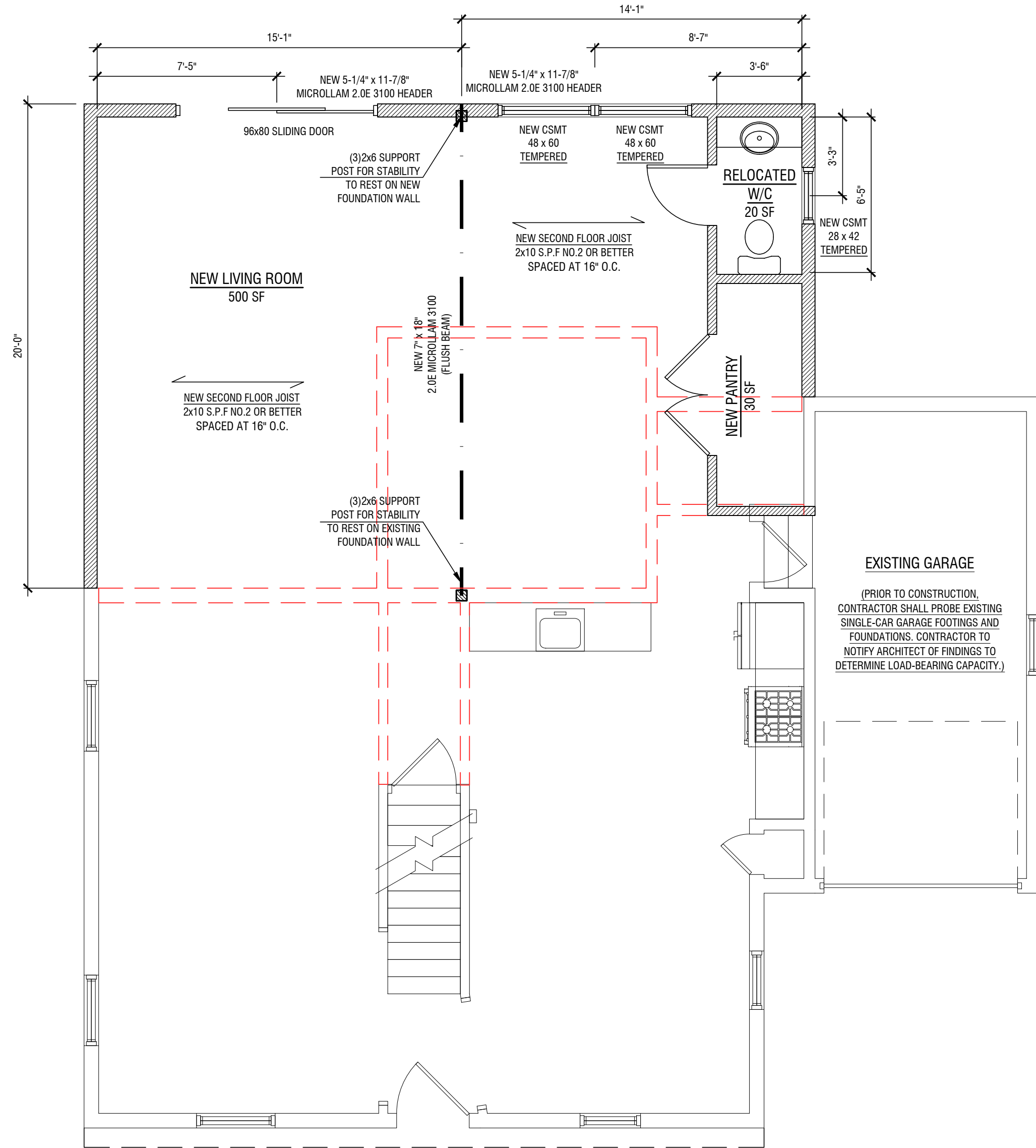
1 CONSTRUCTION PLAN - FIRST FLOOR SCALE: 1/4"=1'-0"
