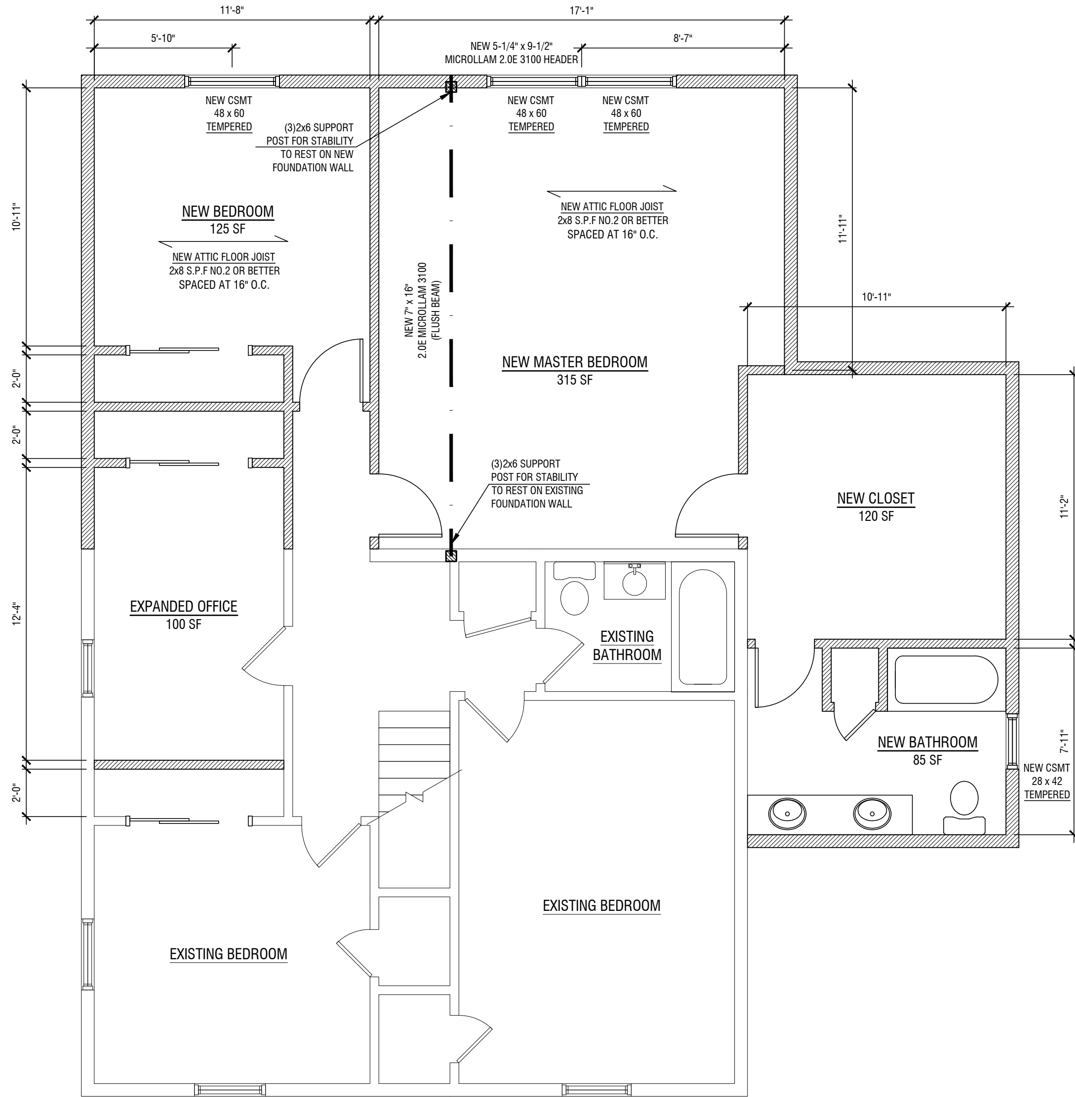
2 CONSTRUCTION PLAN - SECOND FLOOR SCALE: 1/4"=1'-0"
