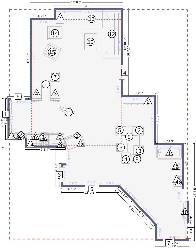
Other 1 Floor Plan
