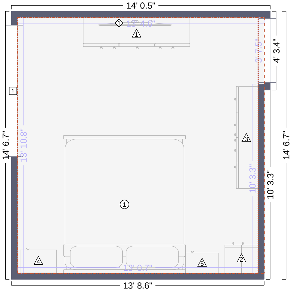
Bedroom 1 Floor Plan
