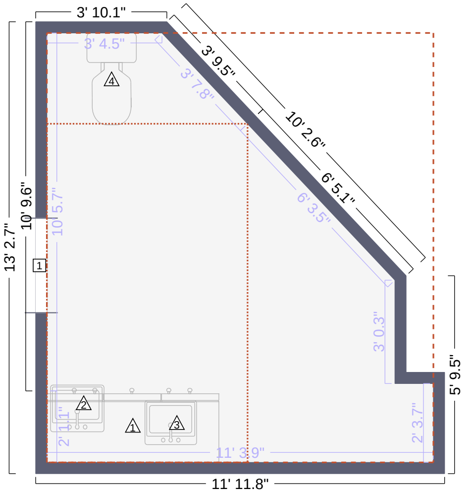
Bathroom 1 Floor Plan
