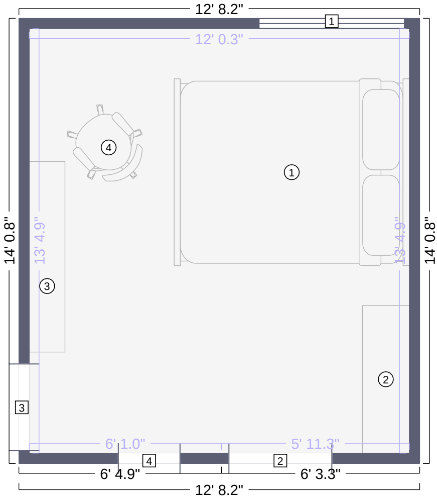
Bedroom 3 Floor Plan
