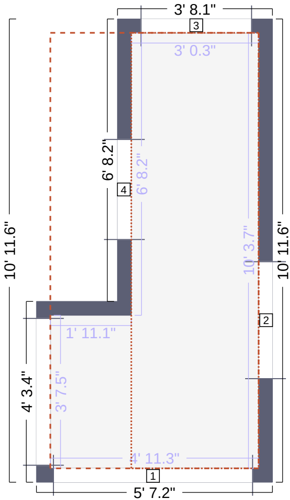
Other 2 Floor Plan
