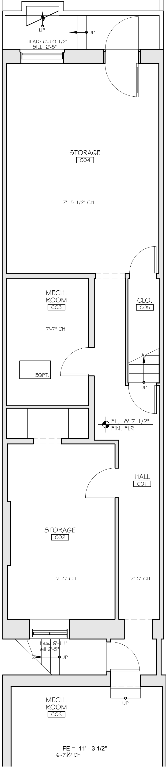
1 EXISTING CELLAR FLOOR PLAN SCALE: 1/4" = 1'-0"
