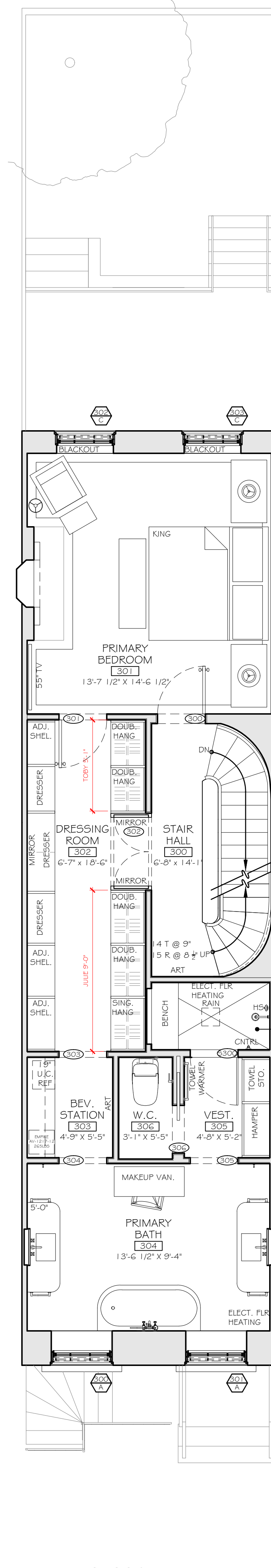
4 PROPOSED 3RD FLOOR PLAN SCALE: 1/4"=1'-0"
