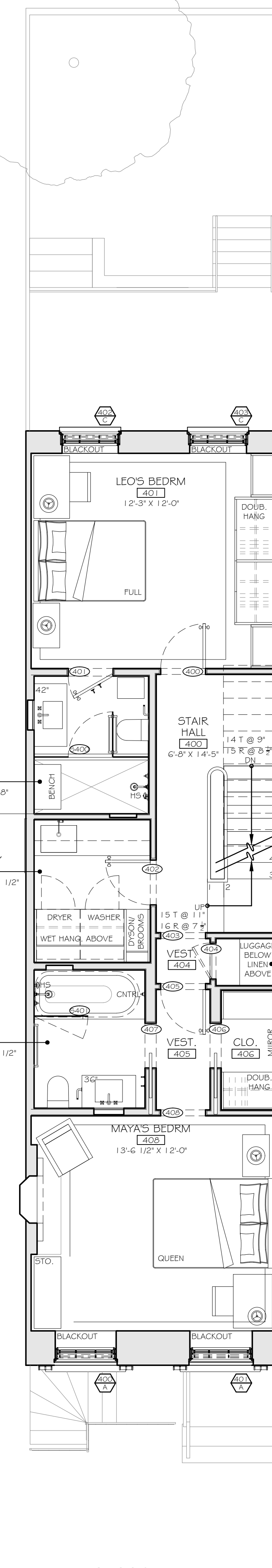
5 PROPOSED 4TH FLOOR PLAN SCALE: 1/4"=1'-0"
