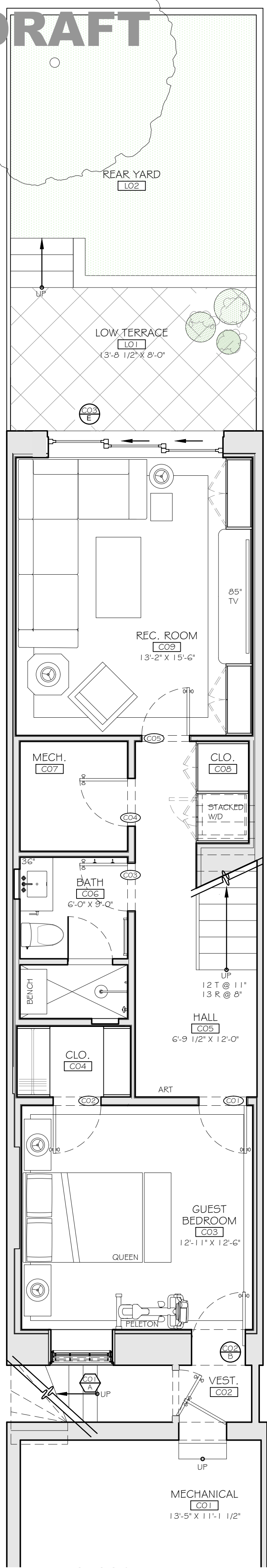
1 PROPOSED CELLAR PLAN A-100 SCALE: 1/4"=1'-0"
