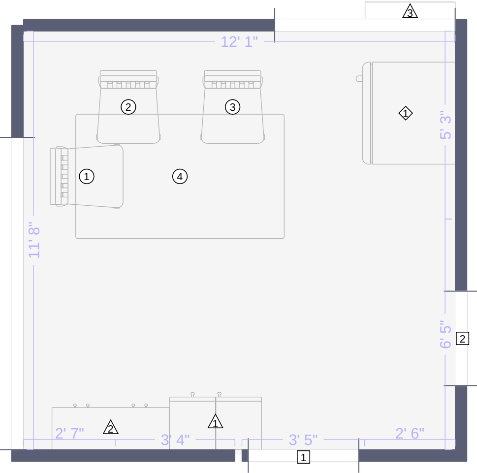
Other 2 Floor Plan
