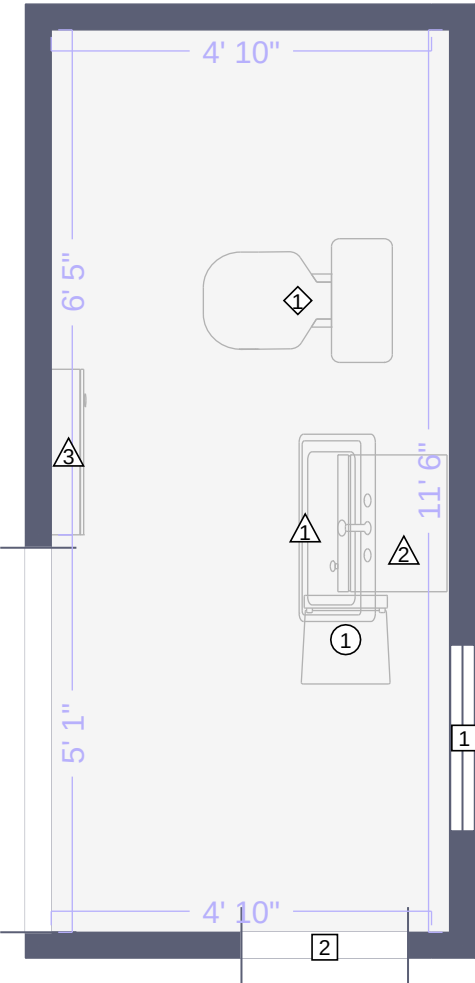
Bathroom 2 Floor Plan
