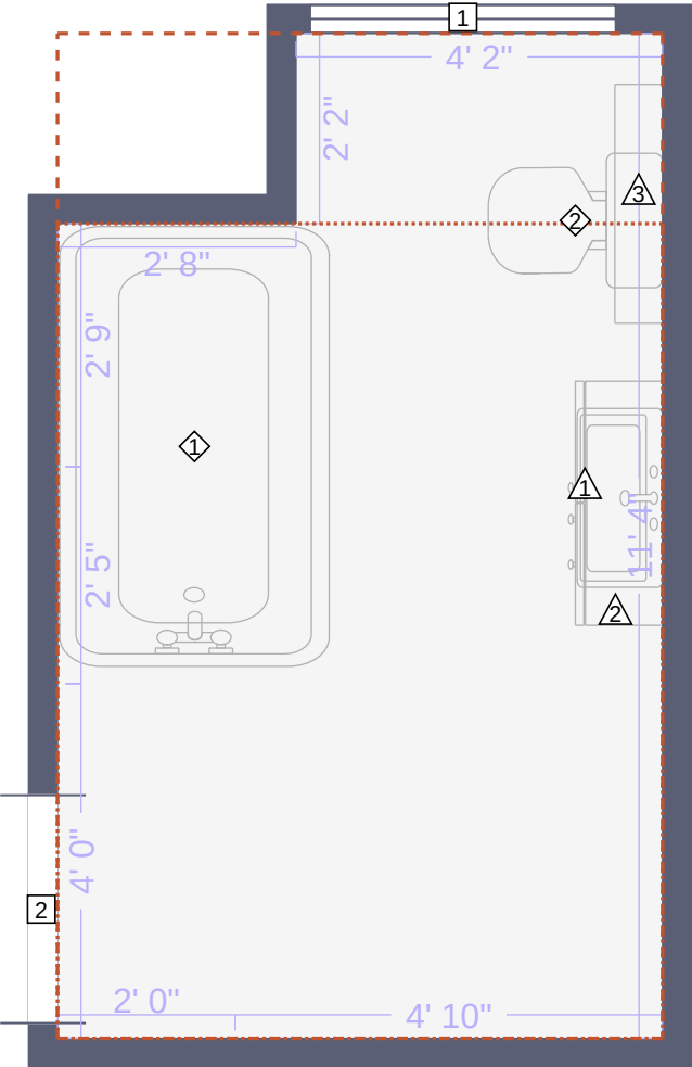
Bathroom 1 Floor Plan
