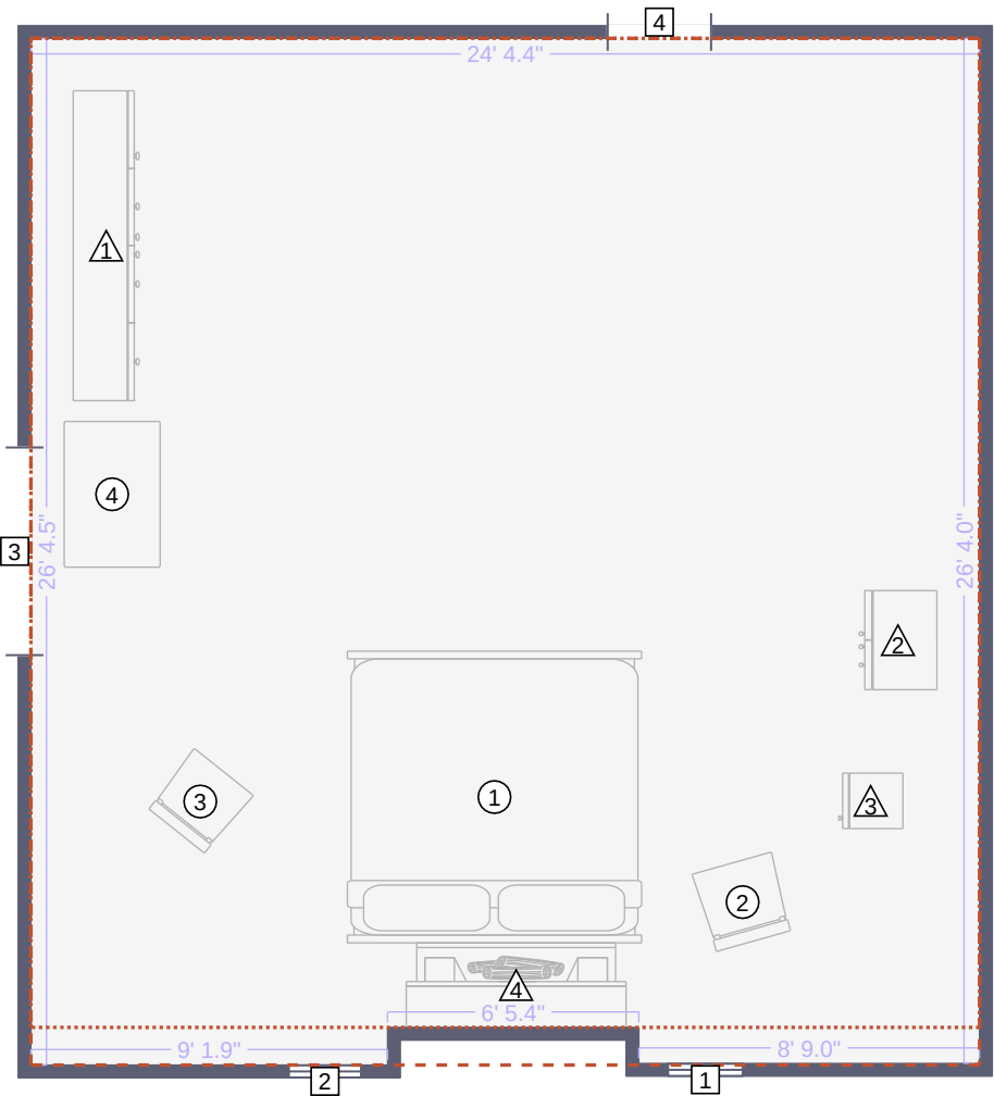
Bedroom 1 Floor Plan
