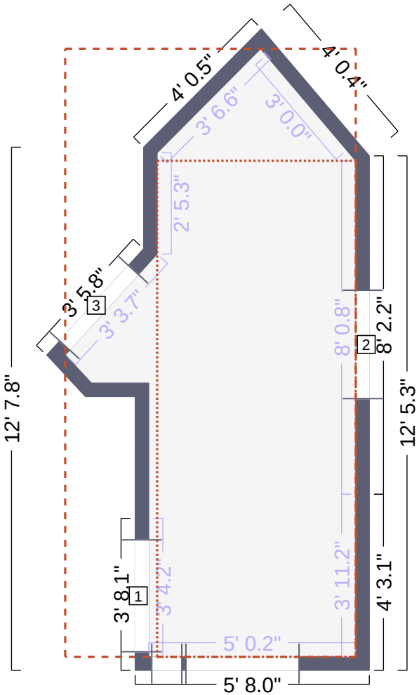
Other 4 Floor Plan
