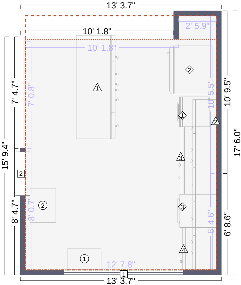
Kitchen 1 Floor Plan
