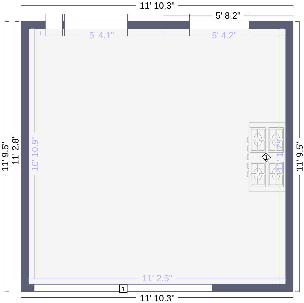
Kitchen 2 Floor Plan
