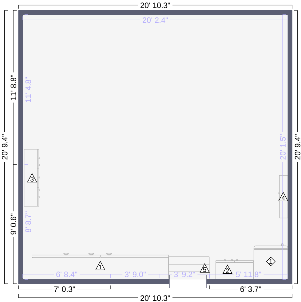
Kitchen 1 Floor Plan
