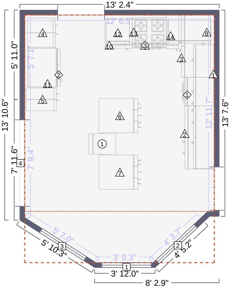
Kitchen 2 Floor Plan
