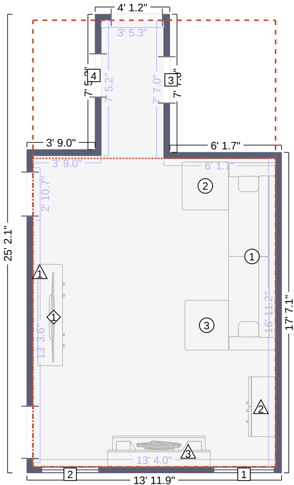
Living Room 2 Floor Plan
