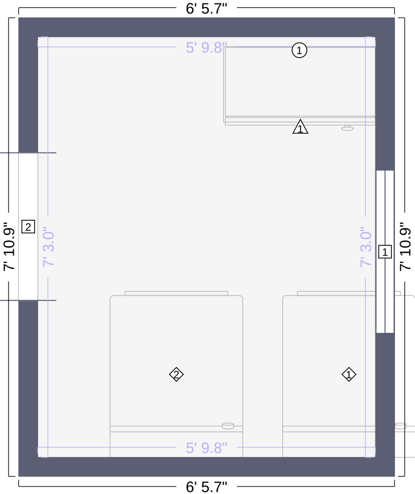
Laundry Floor Plan
