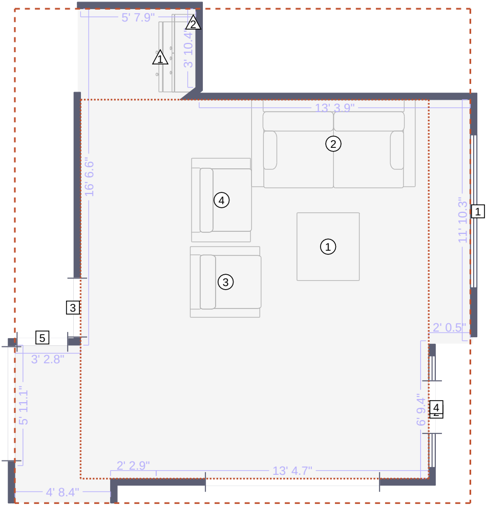
Living Room Floor Plan
