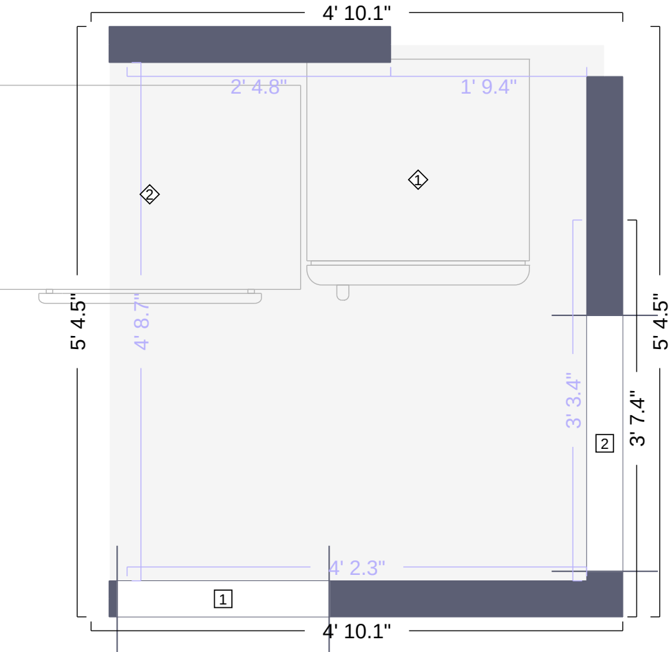
Other 8 Floor Plan
