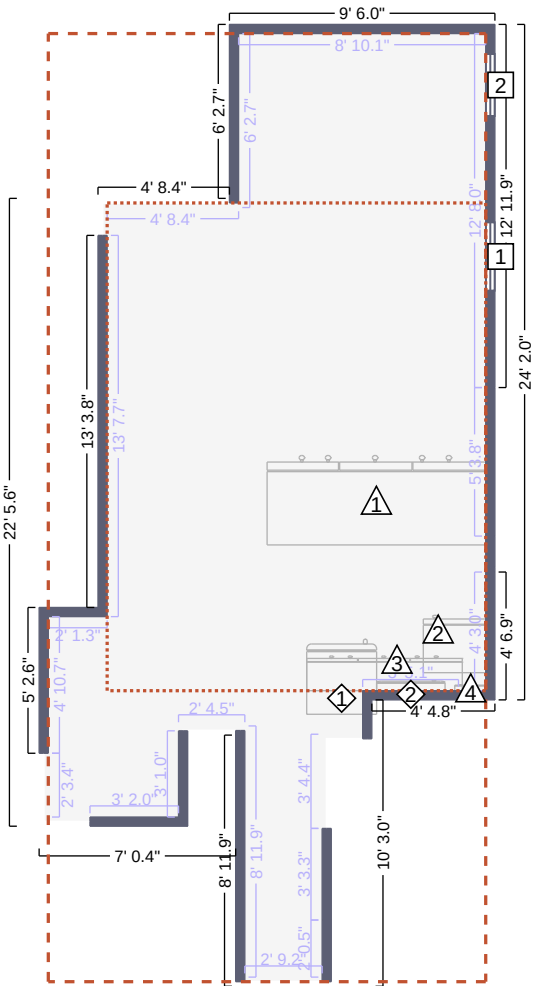
Kitchen Floor Plan
