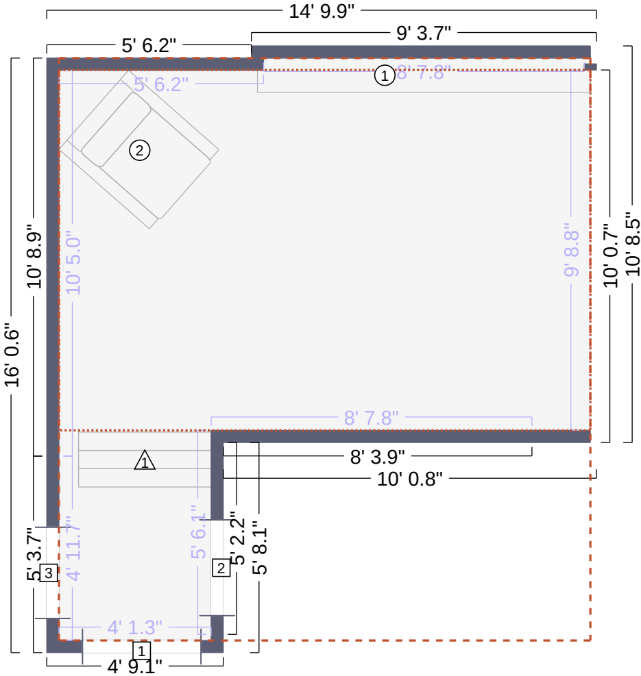
Living Room 3 Floor Plan
