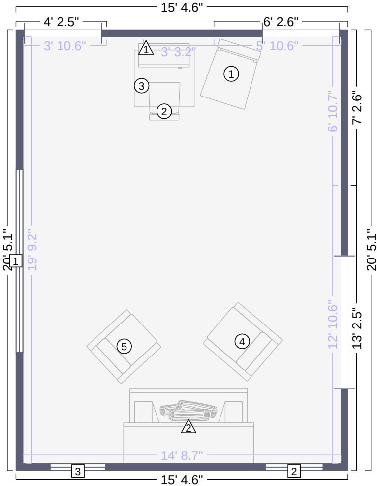
Living Room 1 Floor Plan
