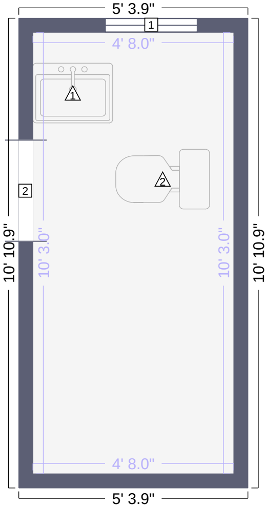
Bathroom 2 Floor Plan
