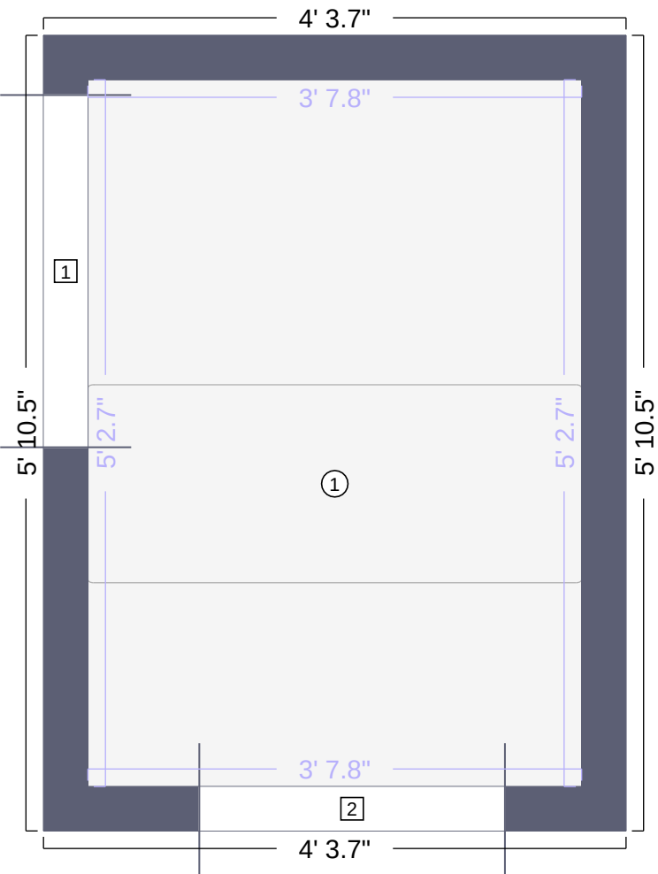
Other 6 Floor Plan
