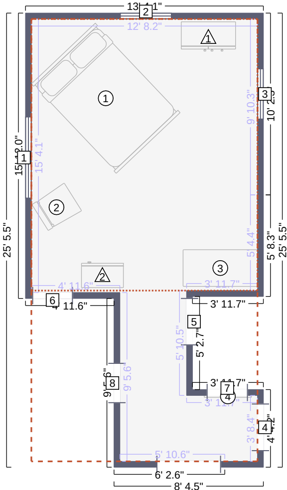
Bedroom 1 Floor Plan
