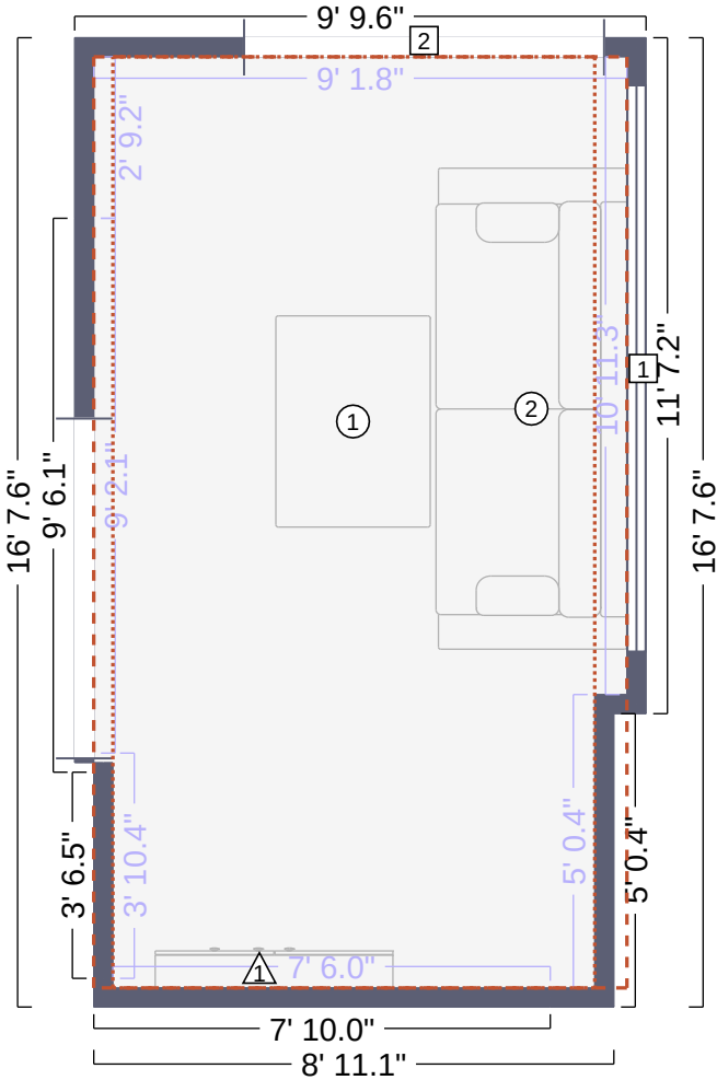
Other 2 Floor Plan
