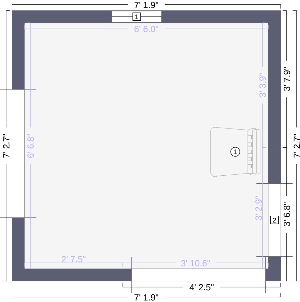
Other 4 Floor Plan
