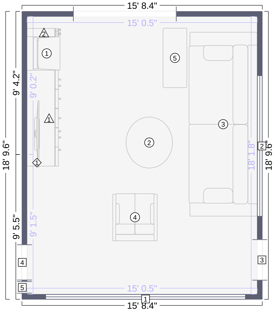
Living Room 1 Floor Plan
