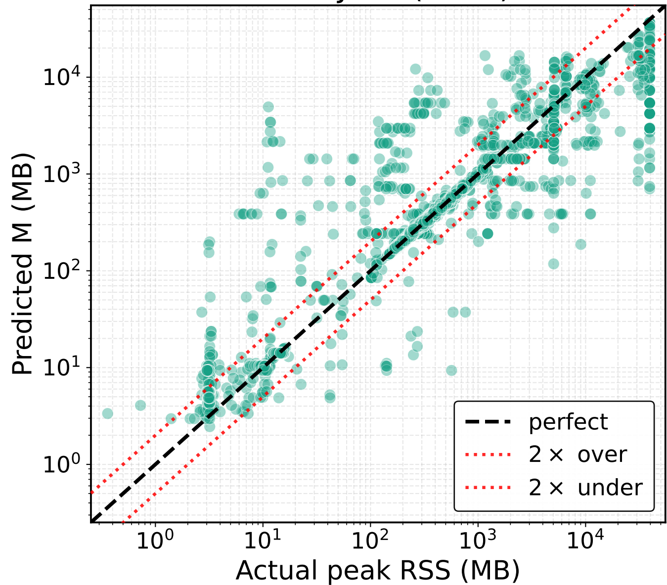
LGBM Joint (a + c)
