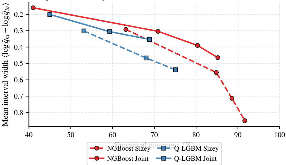
Sharpness vs Coverage
