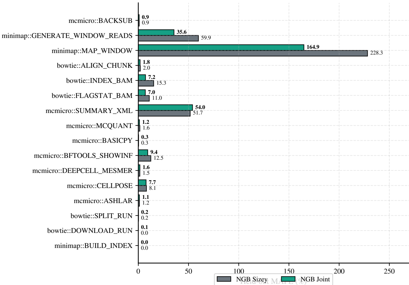
Per-Bucket NGBoost Error
