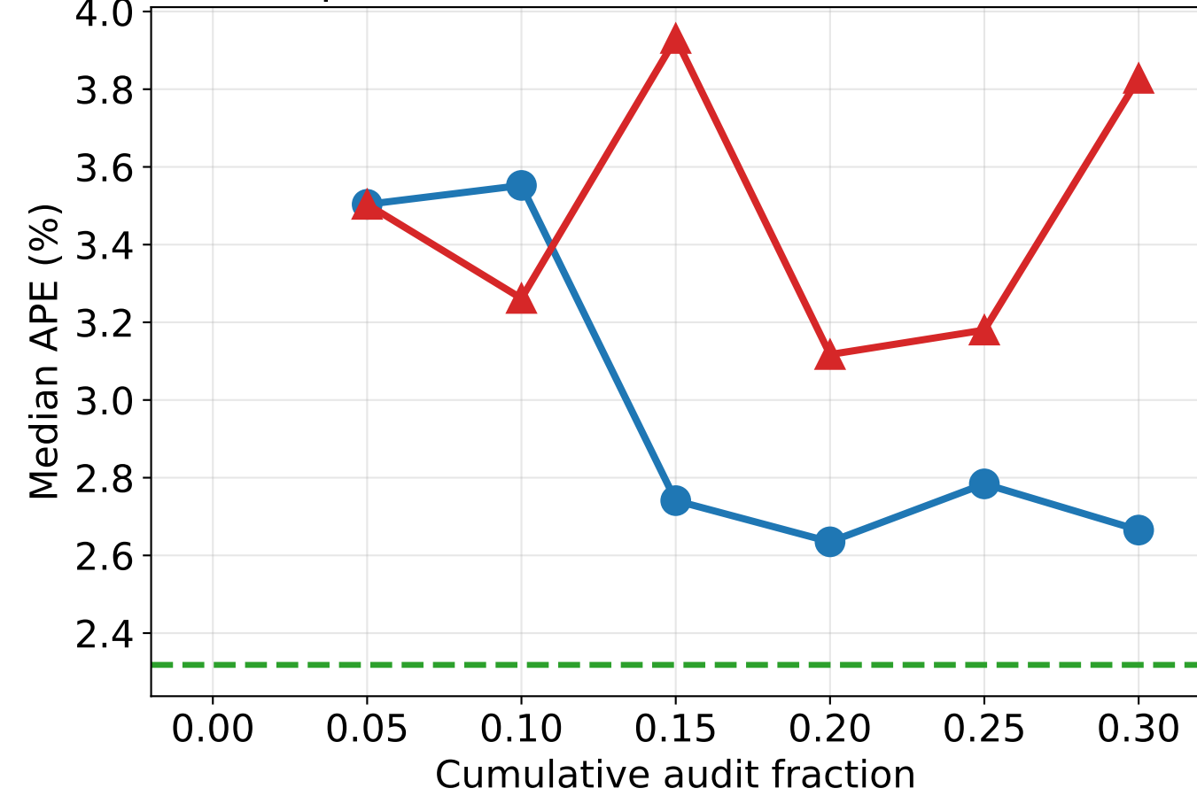
Experiment 3 — Active-learning convergence vs random sampling
