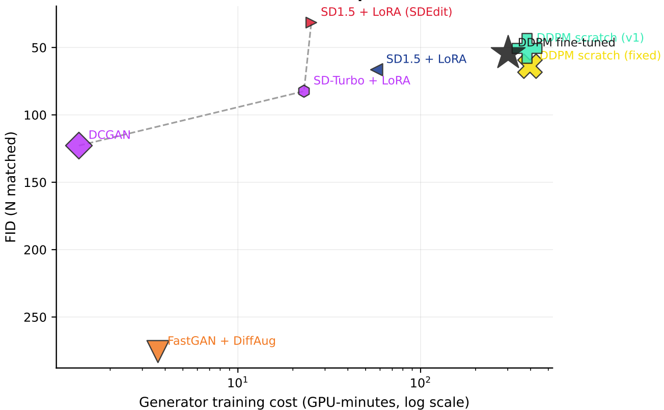
Quality per unit of compute (bubble area \propto trainable parameters)
