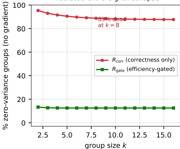
Predicted GRPO signal collapse
