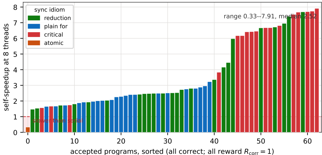
What the correctness-only reward cannot see: 20x scaling spread at identical reward
