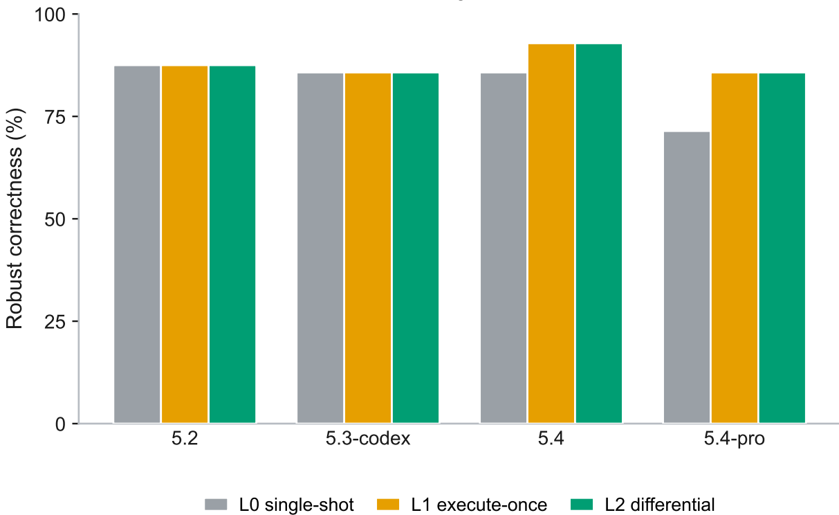
Robust correctness by model and tool level
