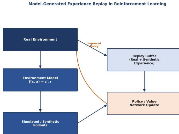
Figure 4: Model-generated experience replay mechanism.
