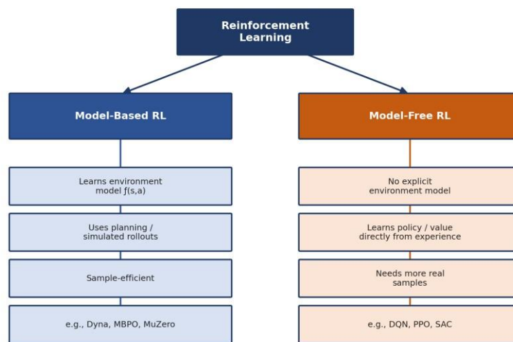
Concept Map: Model-Based RL vs Model-Free RL
