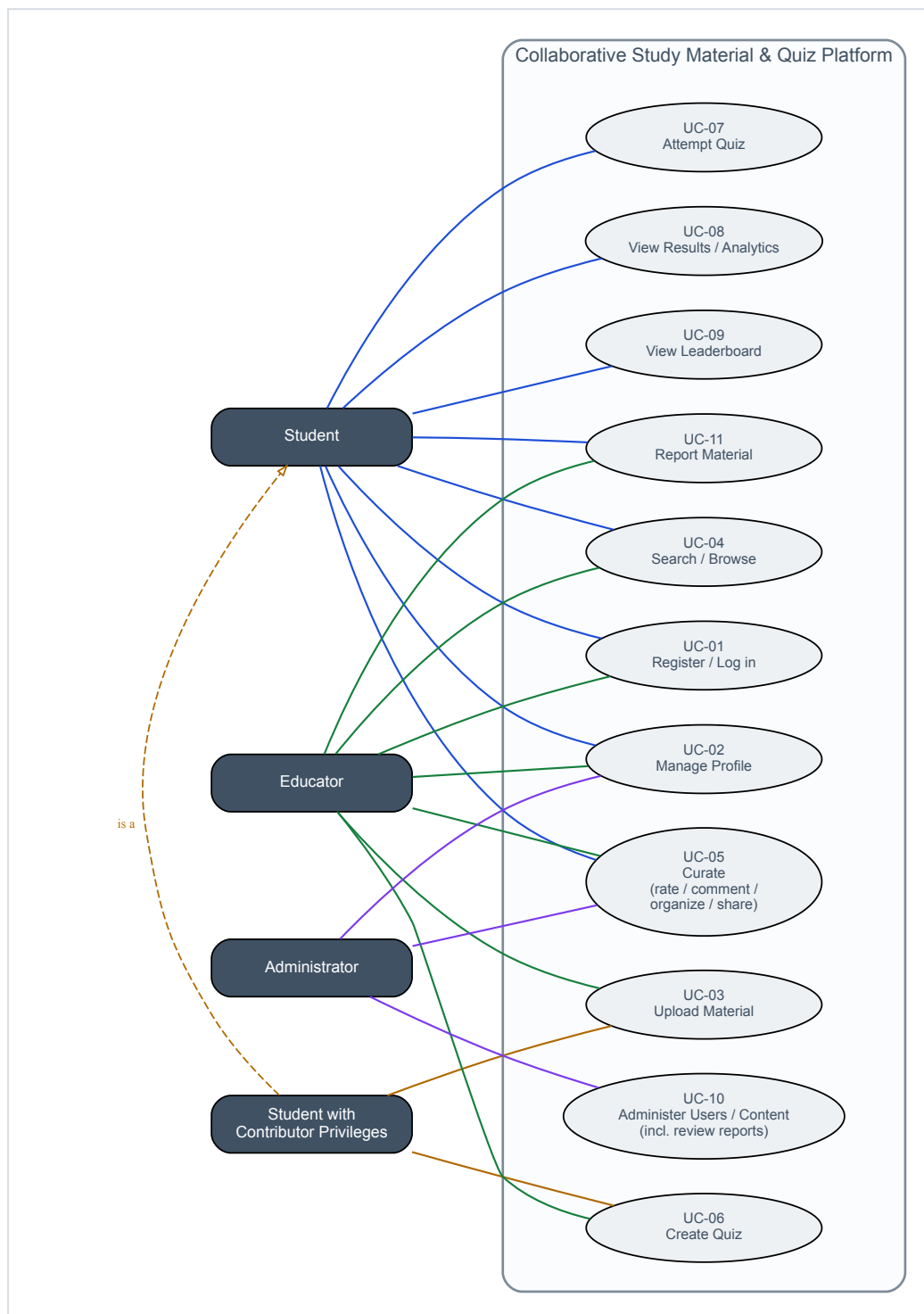
Figure 1 — Use case diagram. “Student with Contributor Privileges” is a generalization of Student (inherits all Student use cases and adds upload/create-quiz).
