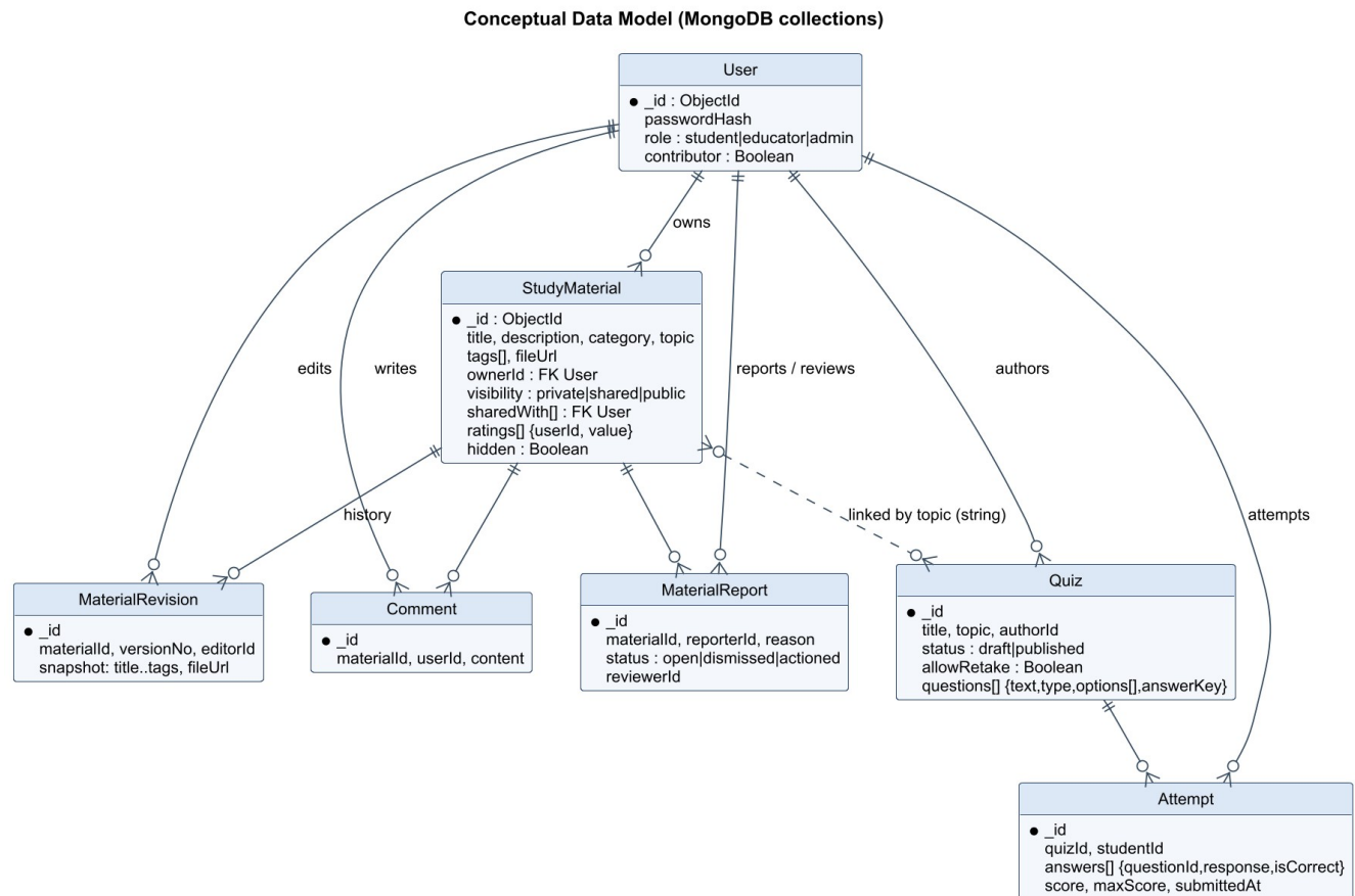
Figure SRS-3: Conceptual data model (MongoDB collections)
