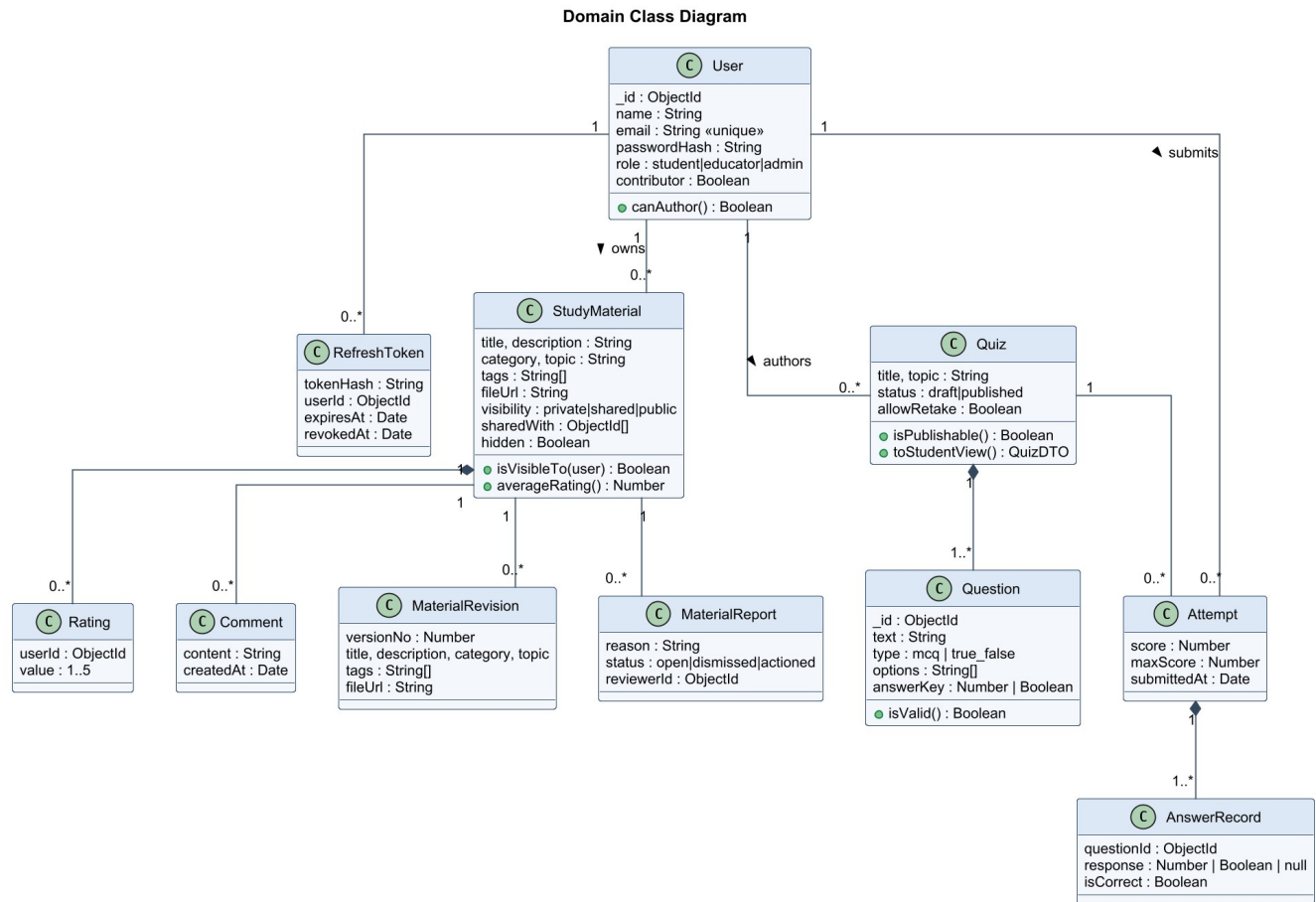
Figure SAD-2: UML class diagram of the domain model
