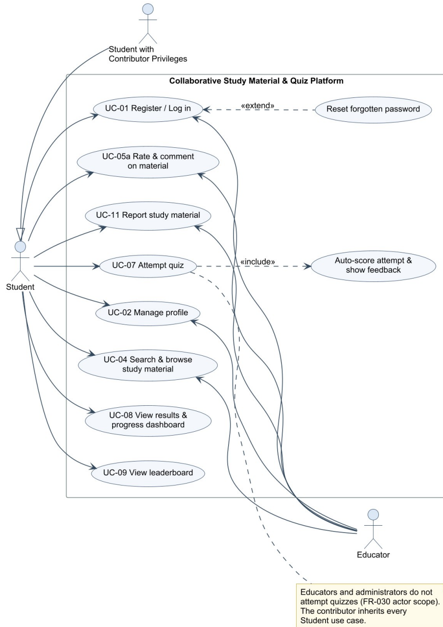
Figure SRS-1: UML Use-Case Diagram 1 — Learning &amp; Self-Assessment
