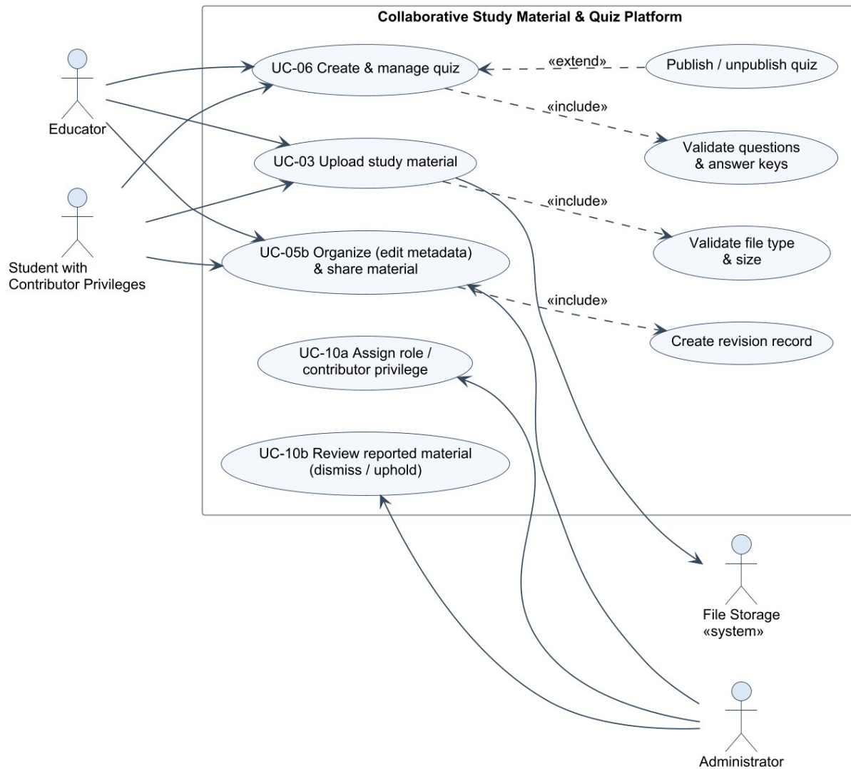
Figure SRS-2: UML Use-Case Diagram 2 — Content Authoring &amp; Administration
