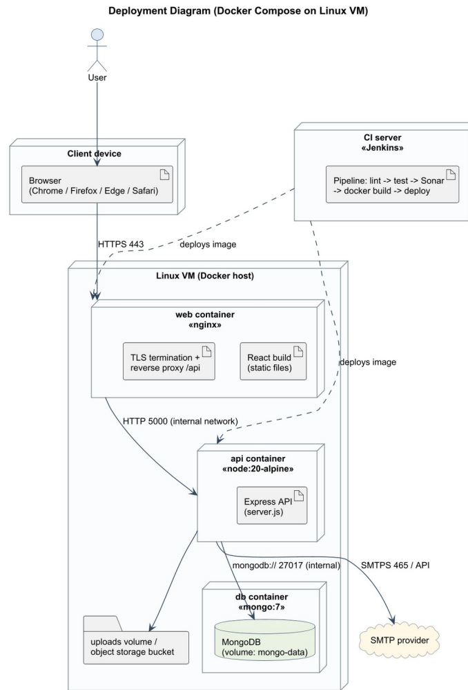
Figure SAD-3: UML deployment diagram
