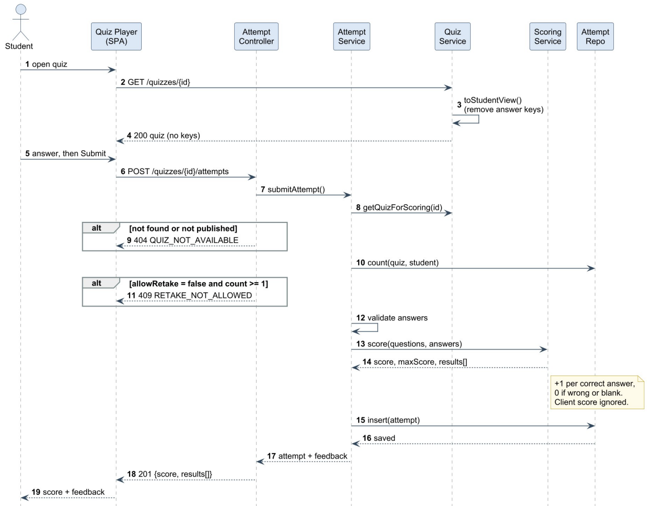
Figure SAD-7: SD-4 Attempt a quiz with automatic scoring
