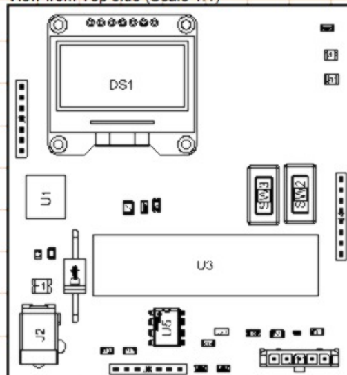
View from Top side (Scale 1:1)
