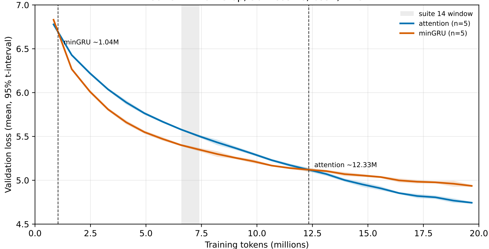
Suite 24: 20M stop, 50M cosine, bs32, n=5
