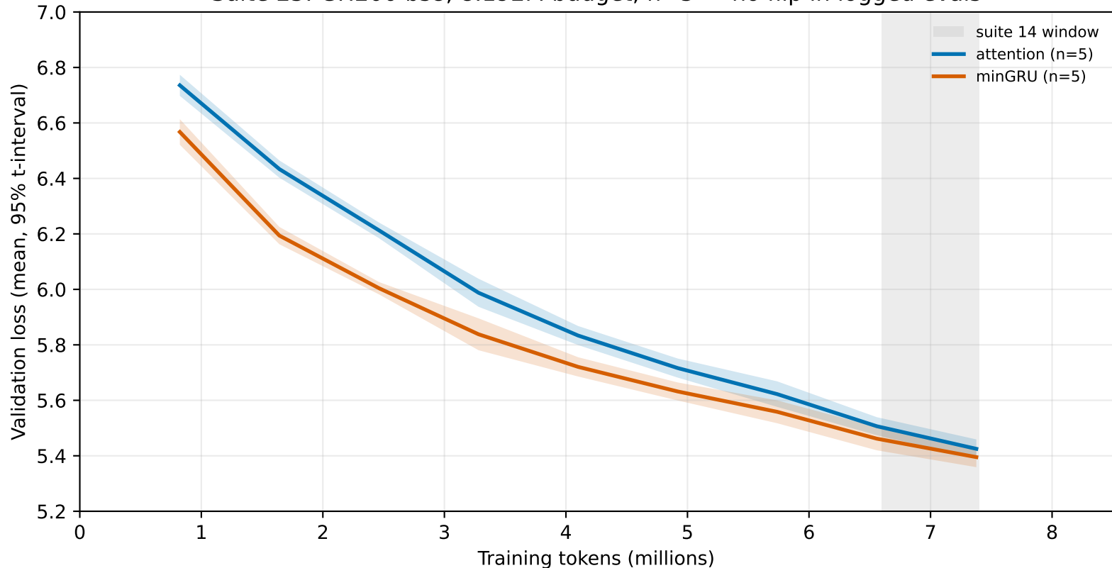
Suite 25: GH200 bs8, 8.192M budget, n=5 — no flip in logged evals
