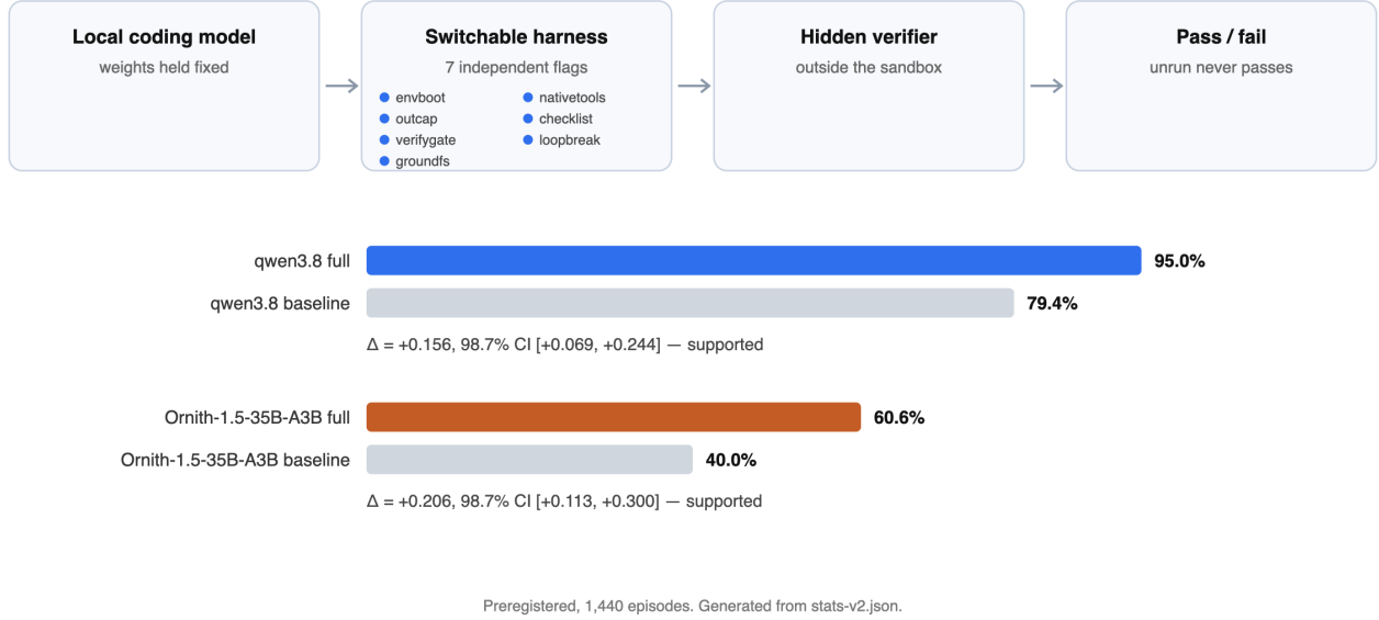
Figure 1. Graphical abstract. The object of measurement is the harness around a frozen local model: seven independently switchable components, a sandbox the agent can write, and a verifier the agent cannot. On the eight-task hard suite under the registered v2 protocol, Qwen 3.8 27B goes from 79.4% (baseline) to 95.0% (full) and Ornith-1.5 35B-A3B from 40.0% to 60.6%. Both deltas exclude zero at the Šidák-corrected 98.7% level. The 720-episode v1 grid that revision 2 reported is superseded and appears only as §5.9’s instrument-failure record. This figure is generated from stats-v2.json like every other data figure; the hand-drawn version it replaces still carried protocol-1’s 97.5%-versus-75% and \Delta + 22.5 , which revision 2 had already archived as not-the-headline.
