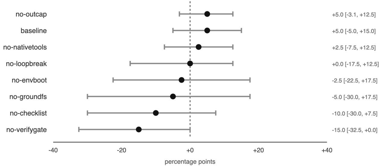
Figure 5. Interaction \Delta_{\text{weaker}} - \Delta_{\text{stronger}} per ablation, unpaired resampling, 95% intervals. This is the block the manuscript cites.
