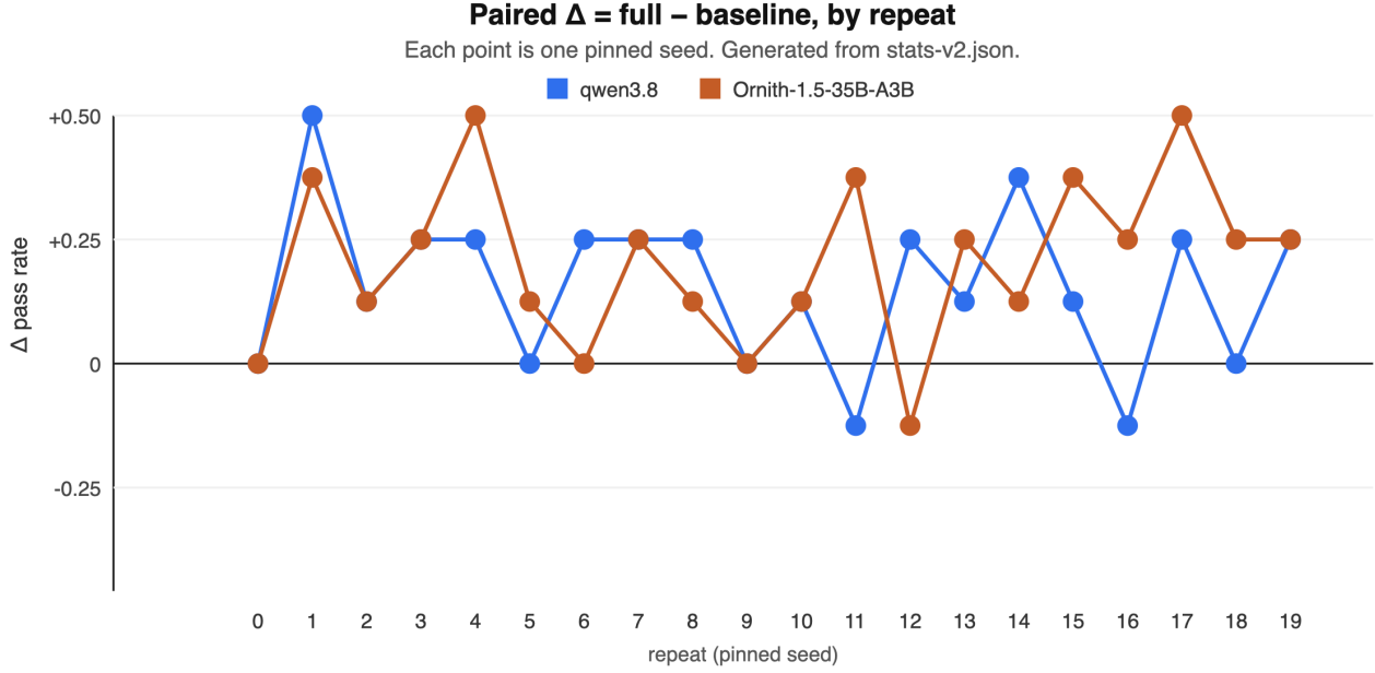
Figure 4. Paired \Delta (full – baseline) at each of the twenty pinned seeds, both arms. Every point is one repeat’s difference of eight-task pass rates. The spread is the quantity the bootstrap resamples; it is what an interval on a single run cannot show.
