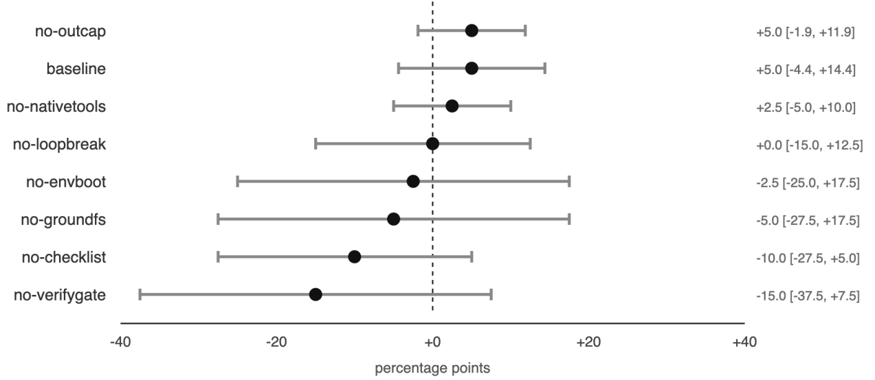
Figure 6. The same statistic under the seed-paired scheme the protocol describes. Published side by side deliberately: the two procedures give different interval widths on the same data, and choosing one silently is the error this pair is meant to prevent.
