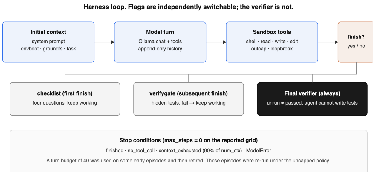
Figure 2. Control flow of one episode. Initial context, the model turn, and sandbox tools are flag-gated. The first finish may inject a checklist. A later finish may run the hidden verifier and bounce the model back to work. A final verifier always runs after the loop stops, whatever the model claimed.
