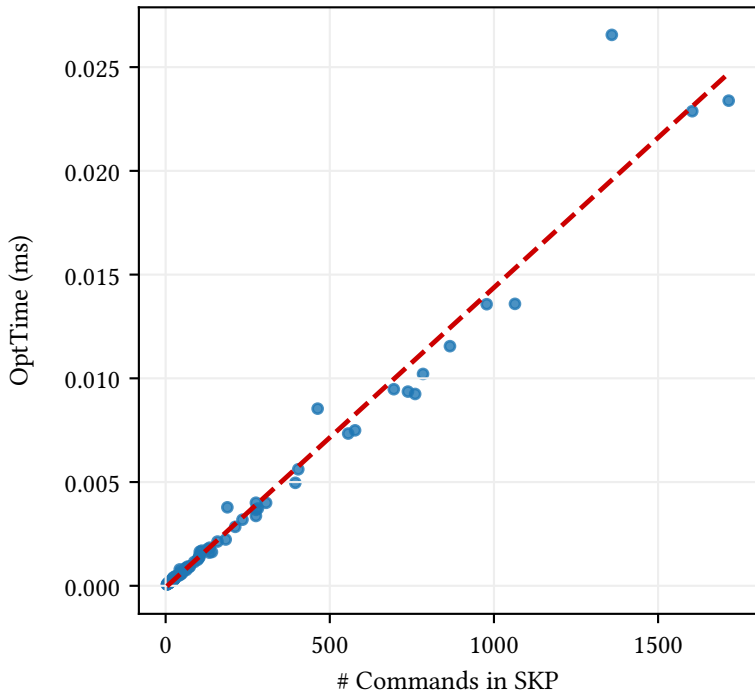
OptTime vs command count (on graphite-metal backend, n=99)
