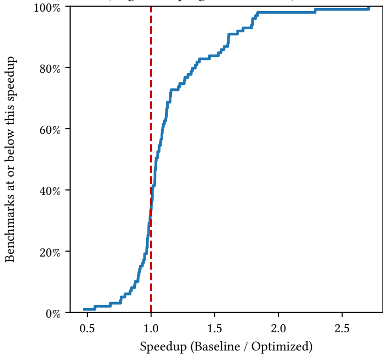
Empirical CDF of speedup (on ganesh-opengl backend, n=99)
