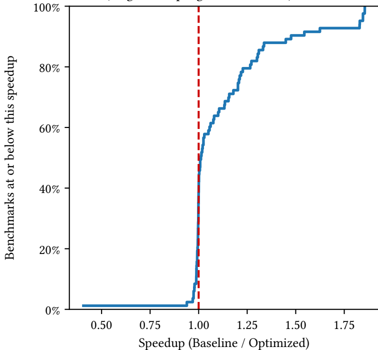
Empirical CDF of speedup (on ganesh-opengl backend, n=83)
