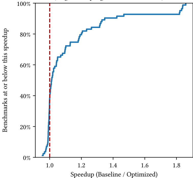
Empirical CDF of speedup (on ganesh-opengl-intel backend, n=83)
