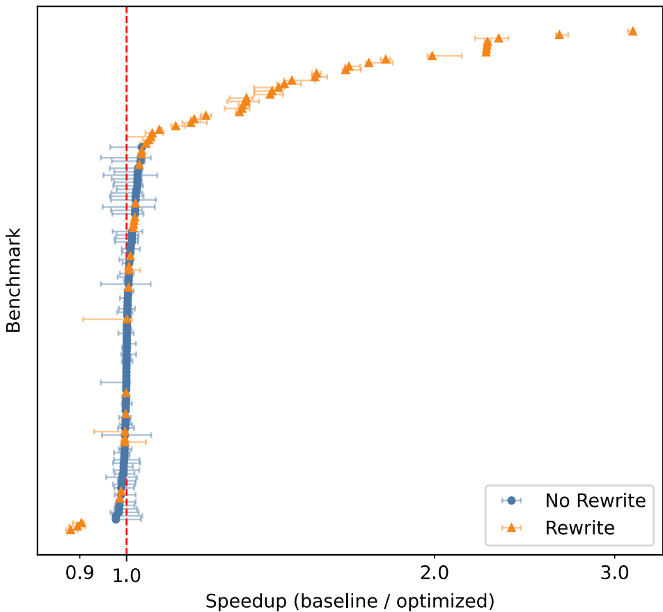
Speedup Confidence Intervals (on Graphite/Intel, N = 143)
