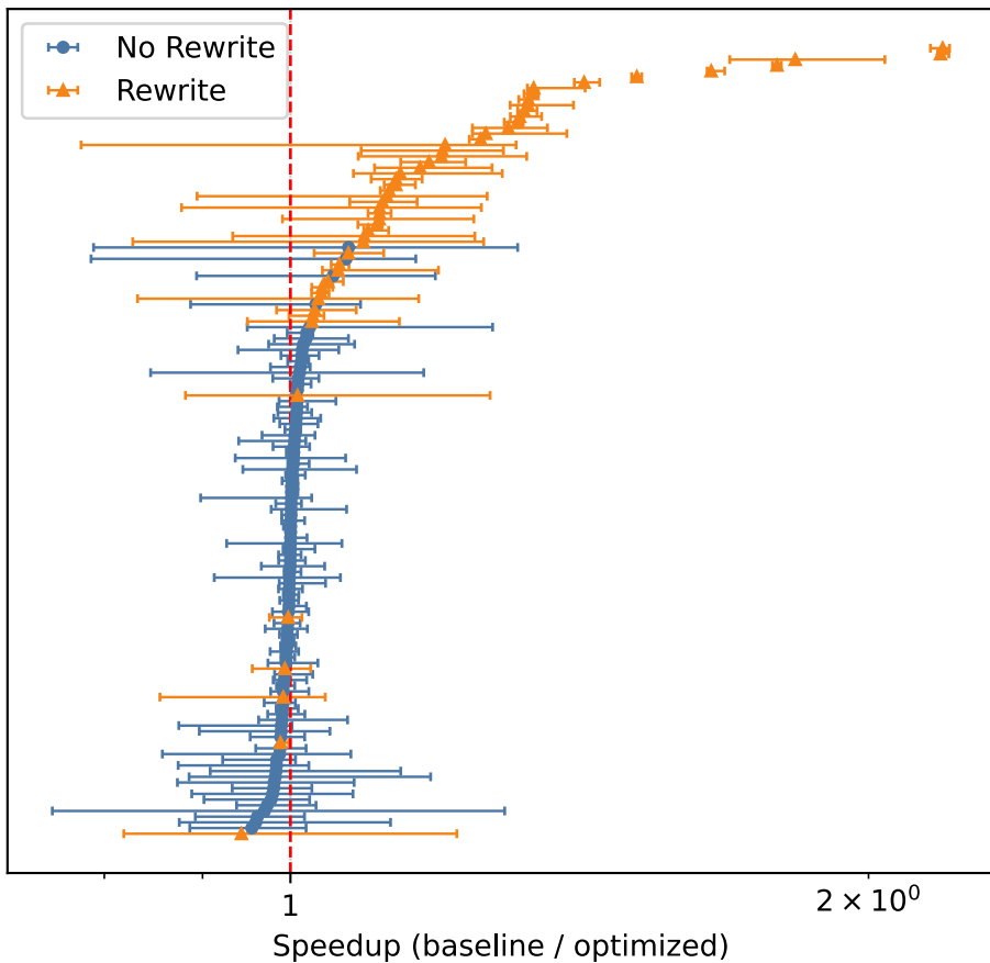
Speedup Confidence Intervals (on Ganesh/Apple, N = 139)
