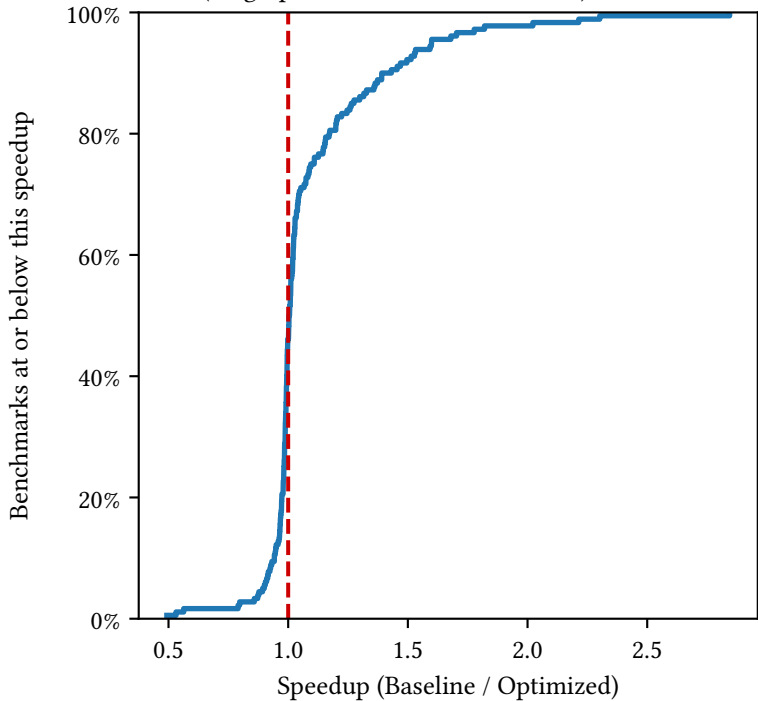
Empirical CDF of speedup (on graphite-metal backend, n=180)
