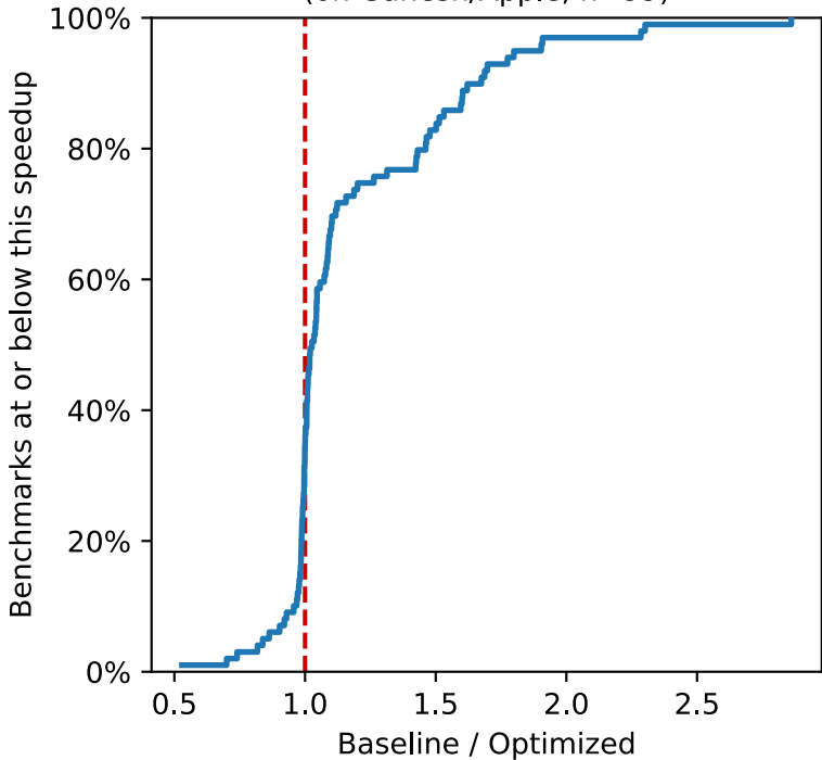
Empirical CDF of speedup (on Ganesh/Apple, n=99)
