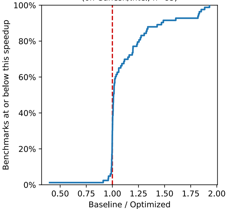
Empirical CDF of speedup (on Ganesh/Intel, n=83)
