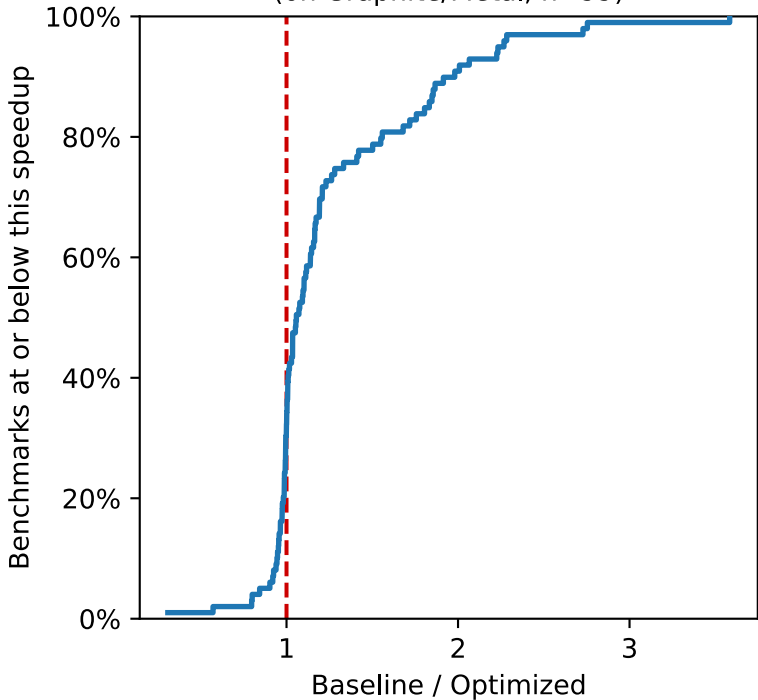
Empirical CDF of speedup (on Graphite/Metal, n=99)
