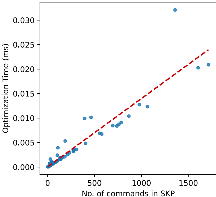
Optimization Time vs Program Size (on Graphite/Metal, n=99)
