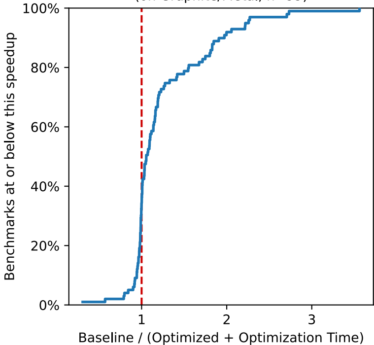
Empirical CDF of total speedup (on Graphite/Metal, n=99)
